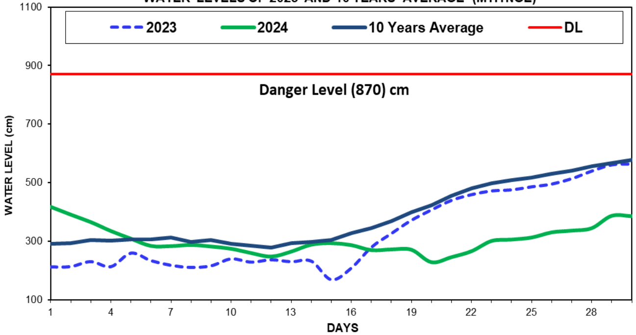
Fig(8) COMPARISON OF JUNE WATER LEVELS OF 2024 WITH JUNE WATER LEVELS OF 2023 AND 10 YEARS AVERAGE (MYITNGE)
