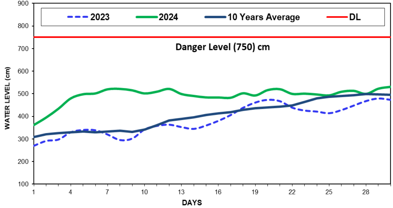
Fig(13) COMPARISON OF JUNE WATER LEVELS OF 2024 WITH JUNE WATER LEVELS OF 2023 AND 10 YEARS AVERAGE (HPA-AN)
