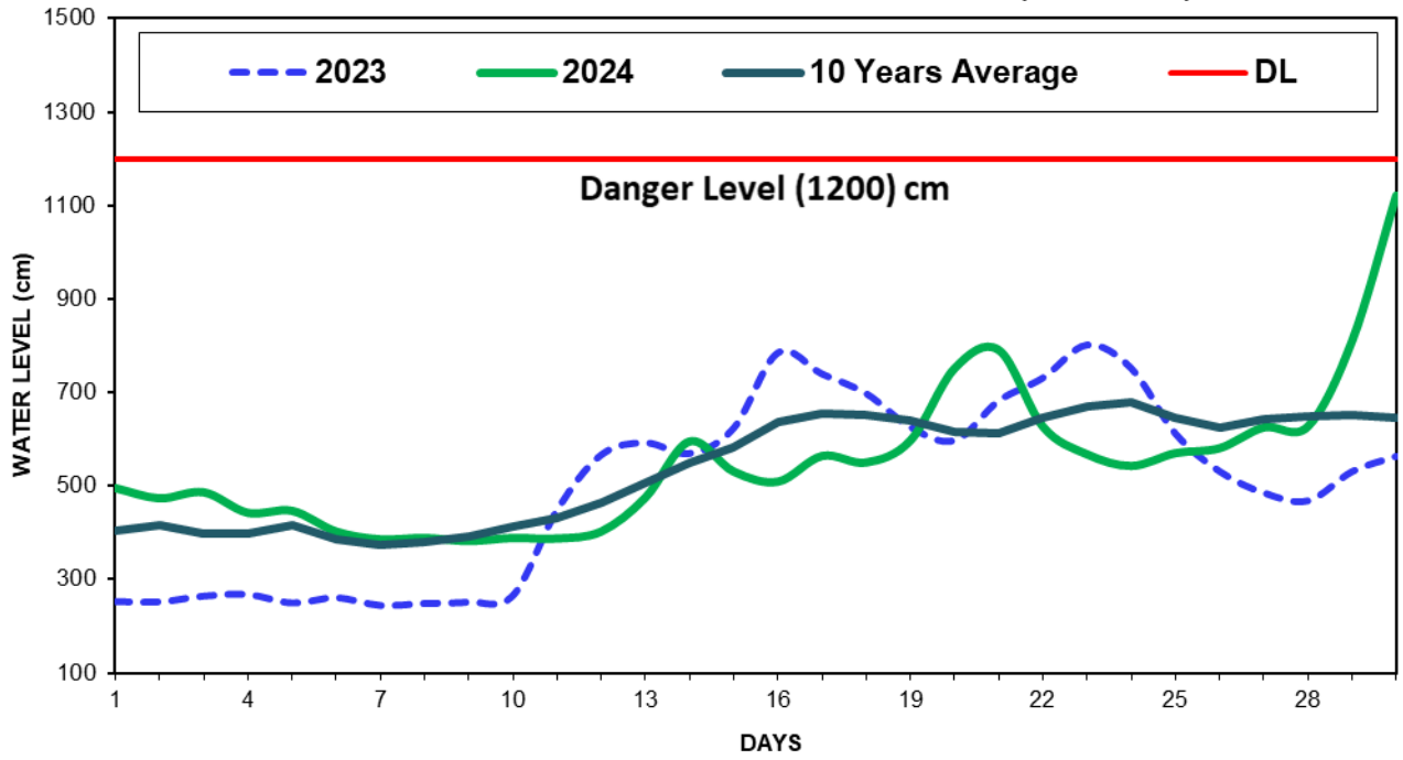
Fig(1) COMPARISON OF JUNE WATER LEVELS OF 2024 WITH JUNE WATER LEVELS OF 2023 AND 10 YEARS AVARAGE (MYITKYINA)
