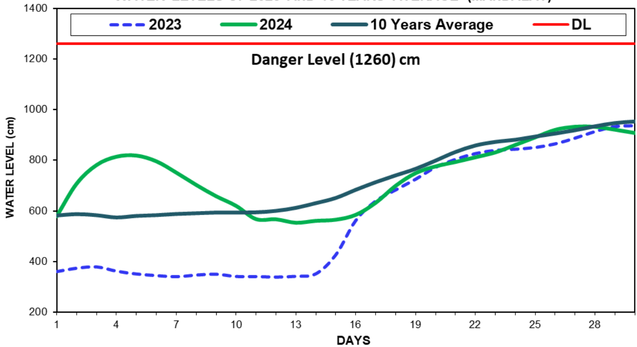
Fig(2) COMPARISON OF JUNE WATER LEVELS OF 2024 WITH JUNE WATER LEVELS OF 2023 AND 10 YEARS AVERAGE (MANDALAY)
