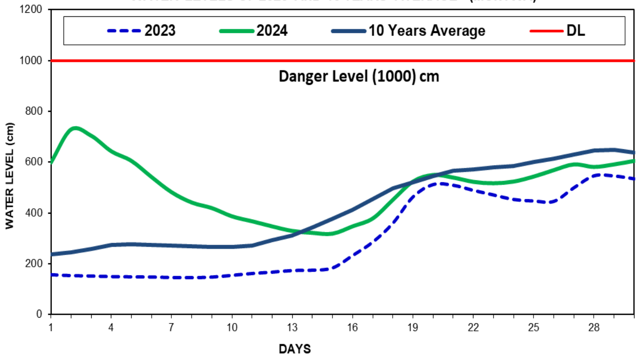
Fig(7) COMPARISON OF JUNE WATER LEVELS OF 2024 WITH JUNE WATER LEVELS OF 2023 AND 10 YEARS AVERAGE (MONYWA)
