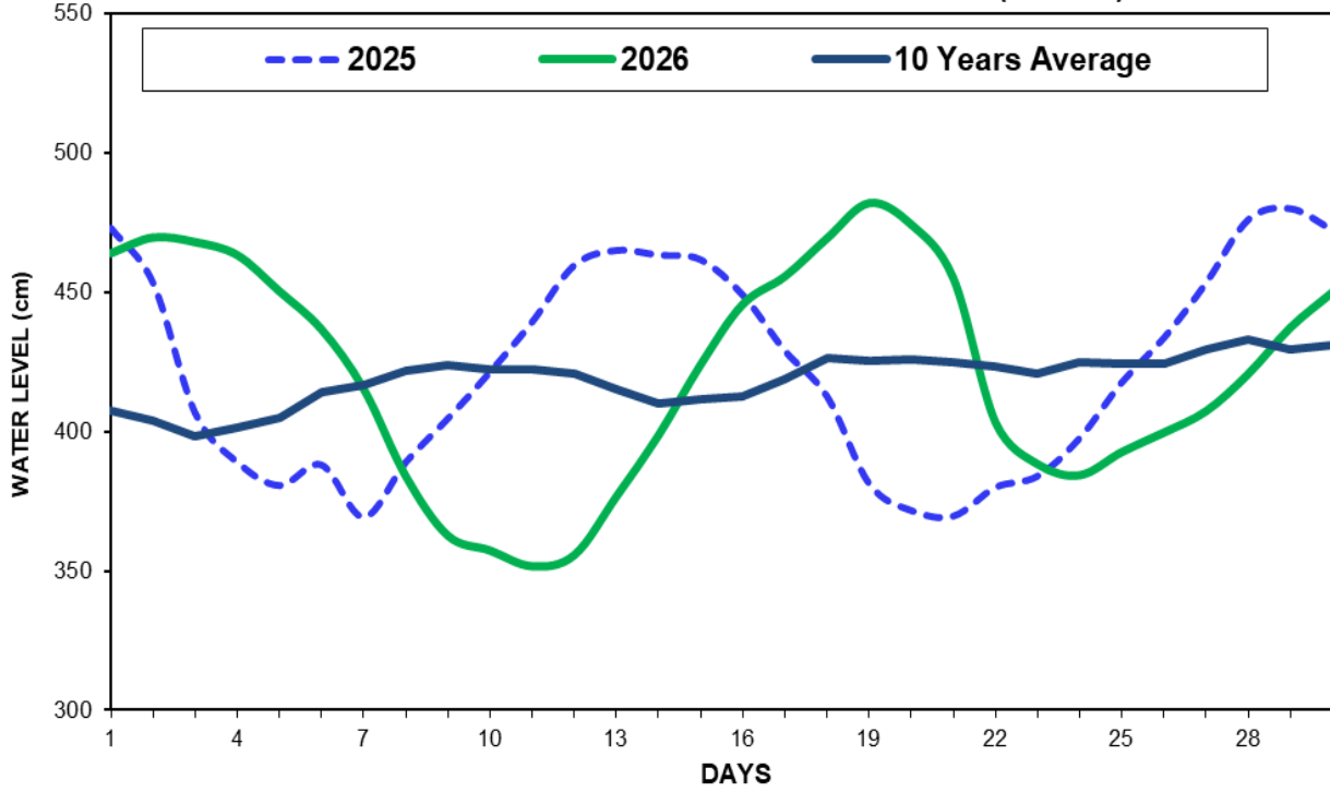
Fig(15) COMPARISON OF APRIL WATER LEVELS OF 2026 WITH APRIL WATER LEVELS OF 2025 AND 10 YEARS AVERAGE (MAUBIN)
