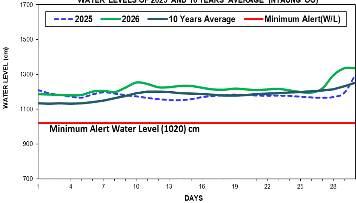
Fig(3) COMPARISON OF APRIL WATER LEVELS OF 2026 WITH APRIL WATER LEVELS OF 2025 AND 10 YEARS AVERAGE (NYAUNG OO)
