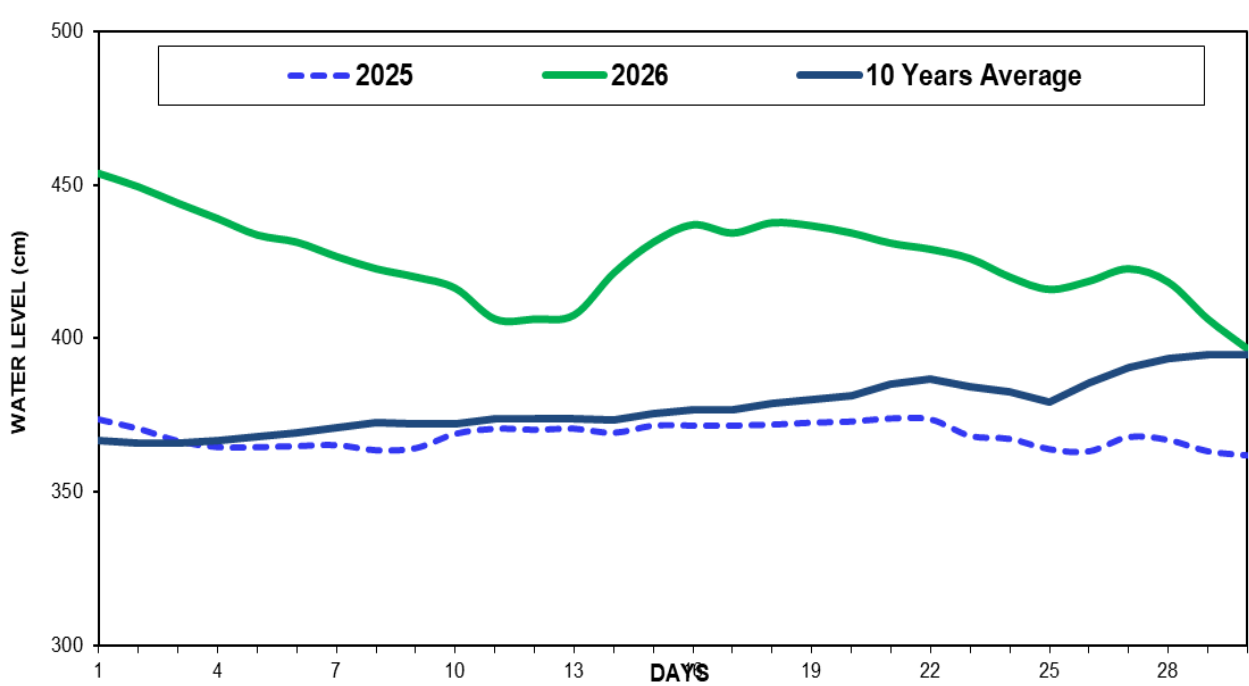
Fig(14) COMPARISON OF APRIL WATER LEVELS OF 2026 WITH APRIL WATER LEVELS OF 2025 AND 10 YEARS AVERAGE (NGATHAINGCHAUNG)
