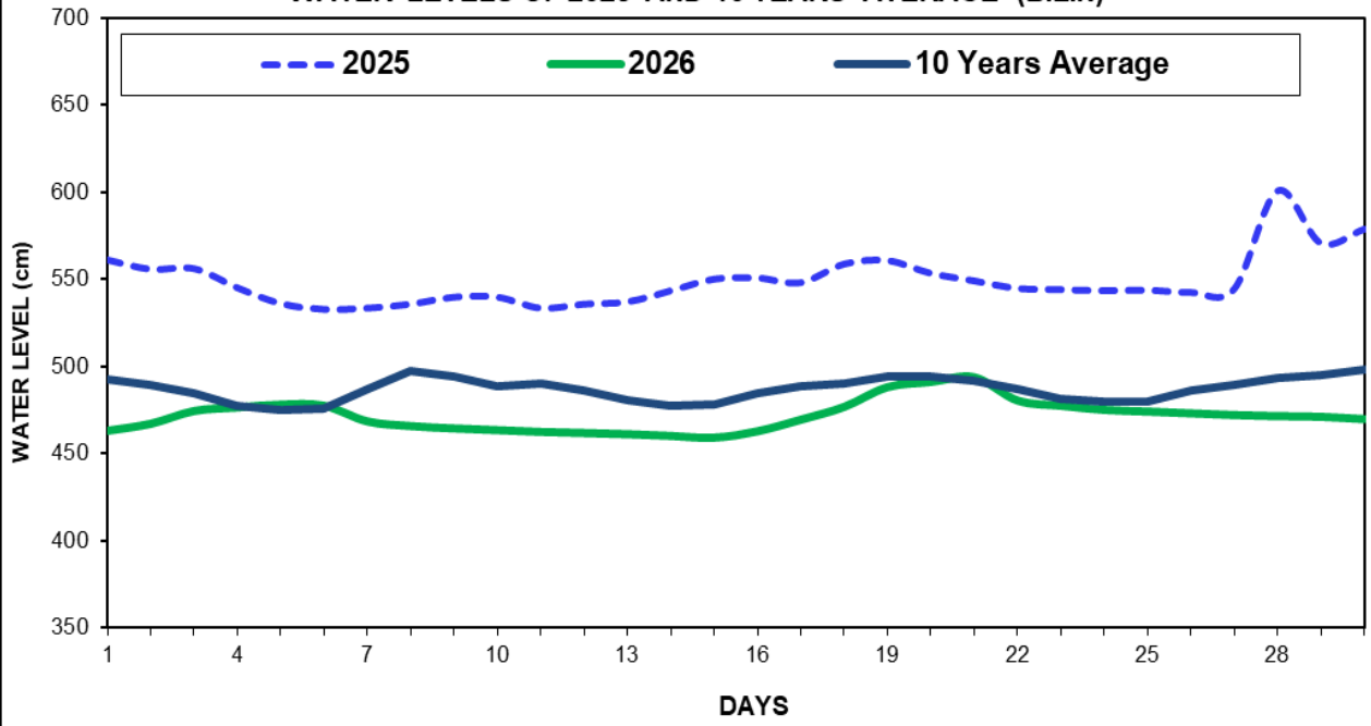
Fig(17) COMPARISON OF APRIL WATER LEVELS OF 2026 WITH APRIL WATER LEVELS OF 2025 AND 10 YEARS AVERAGE (BILIN)
