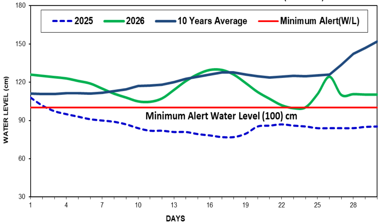
Fig(7) COMPARISON OF APRIL WATER LEVELS OF 2026 WITH APRIL WATER LEVELS OF 2025 AND 10 YEARS AVERAGE (MONYWA)
