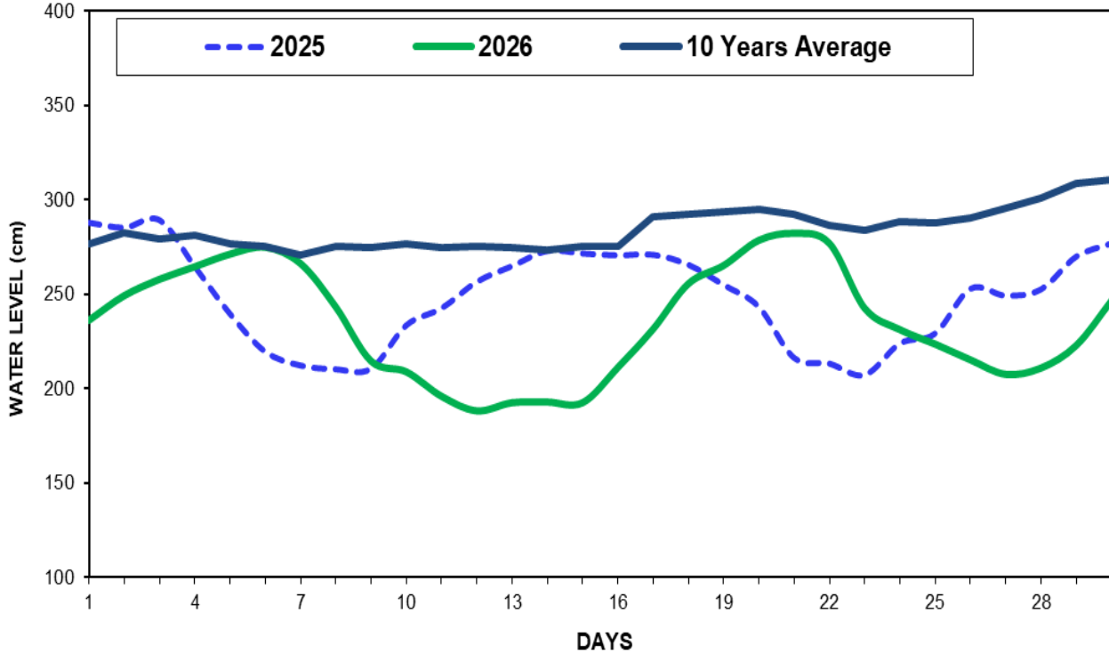
Fig(12) COMPARISON OF APRIL WATER LEVELS OF 2026 WITH APARIL WATER LEVELS OF 2025 AND 10 YEARS AVERAGE (BAGO)
