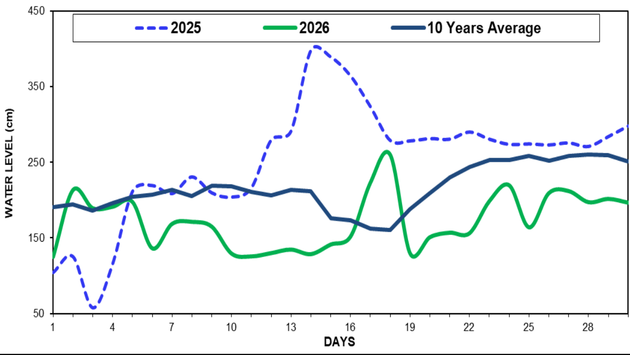
Fig(8) COMPARISON OF APRIL WATER LEVELS OF 2026 WITH APRIL WATER LEVELS OF 2025 AND 10 YEARS AVERAGE (MYITNGE)
