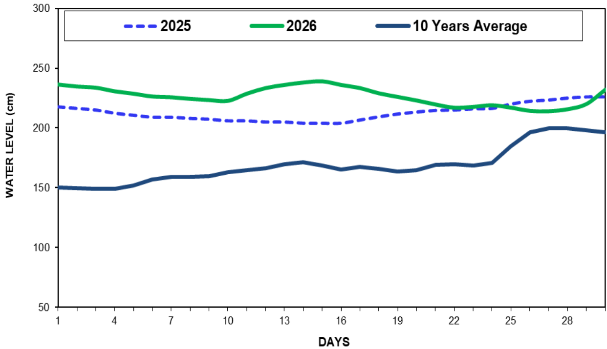
Fig(6) COMPARISON OF APRIL WATER LEVELS OF 2026 WITH APRIL WATER LEVELS OF 2025 AND 10 YEARS AVERAGE (MAWLAIK)
