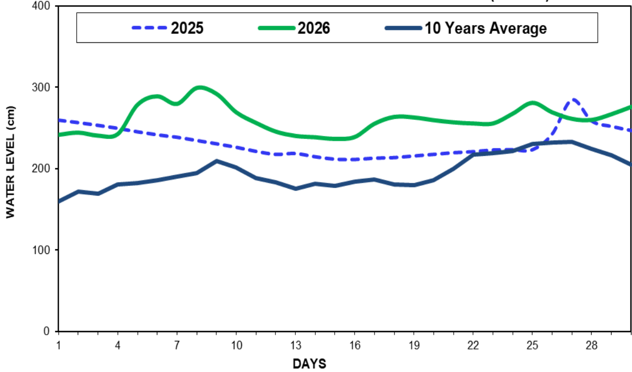
Fig(5) COMPARISON OF APRIL WATER LEVELS OF 2026 WITH APRIL WATER LEVELS OF 2025 AND 10 YEARS AVERAGE (HKAMTI)
