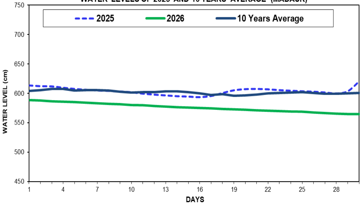
Fig(10) COMPARISON OF APRIL WATER LEVELS OF 2026 WITH APRIL WATER LEVELS OF 2025 AND 10 YEARS AVERAGE (MADAUK)
