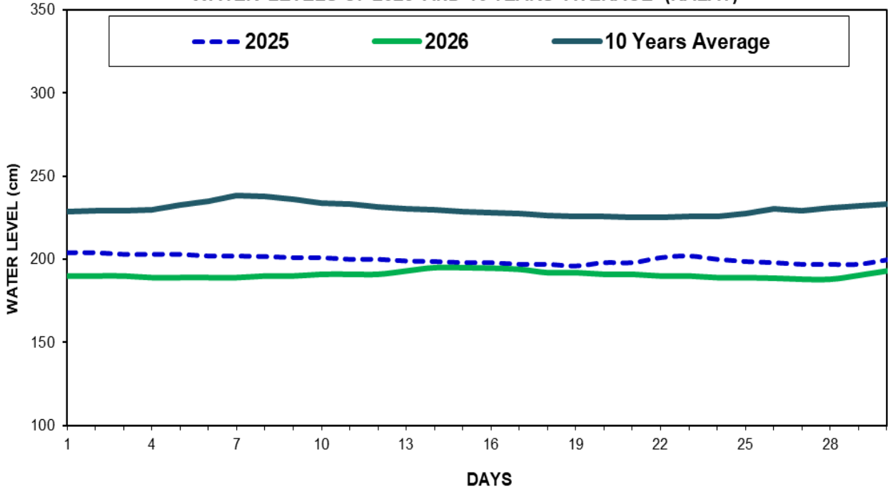
Fig(16) COMPARISON OF APRIL WATER LEVELS OF 2026 WITH APRIL WATER LEVELS OF 2025 AND 10 YEARS AVERAGE (KALAY)
