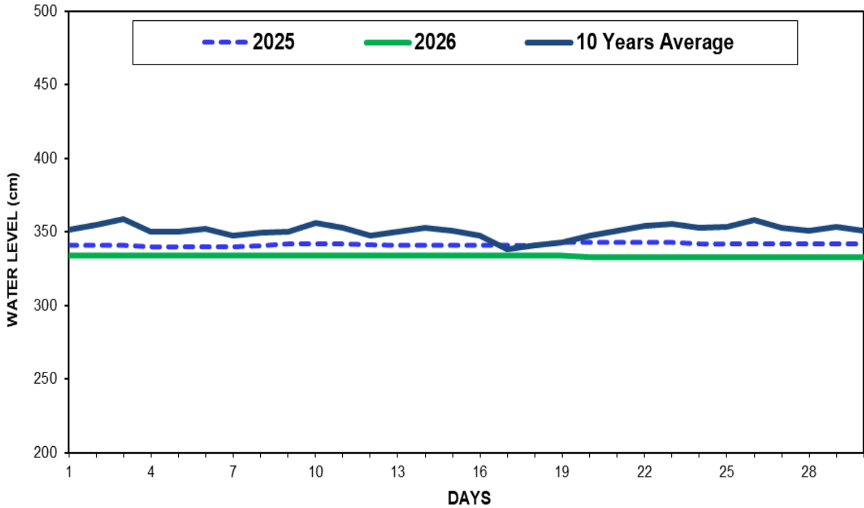
Fig(11) COMPARISON OF APRIL WATER LEVELS OF 2026 WITH APRIL WATER LEVELS OF 2025 AND 10 YEARS AVERAGE (SHWEGYIN)
