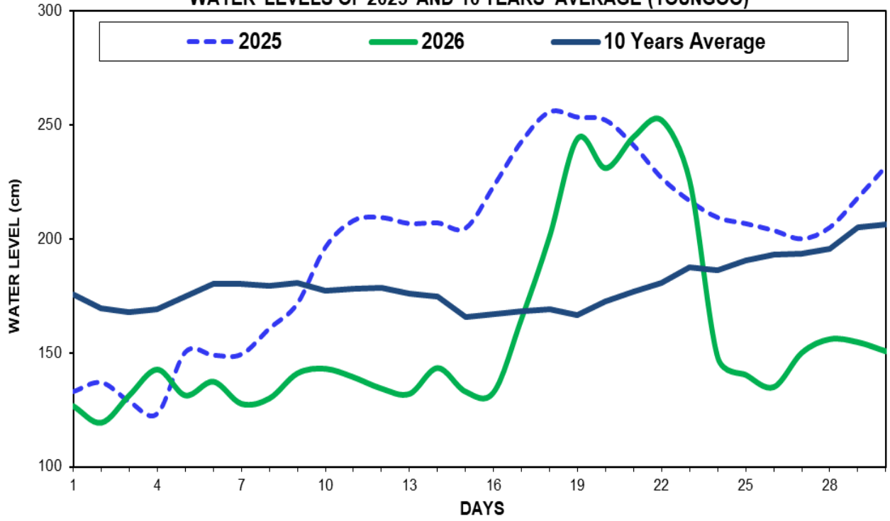
Fig(9) COMPARISON OF APRIL WATER LEVELS OF 2026 WITH APRIL WATER LEVELS OF 2025 AND 10 YEARS AVERAGE (TOUNGOO)
