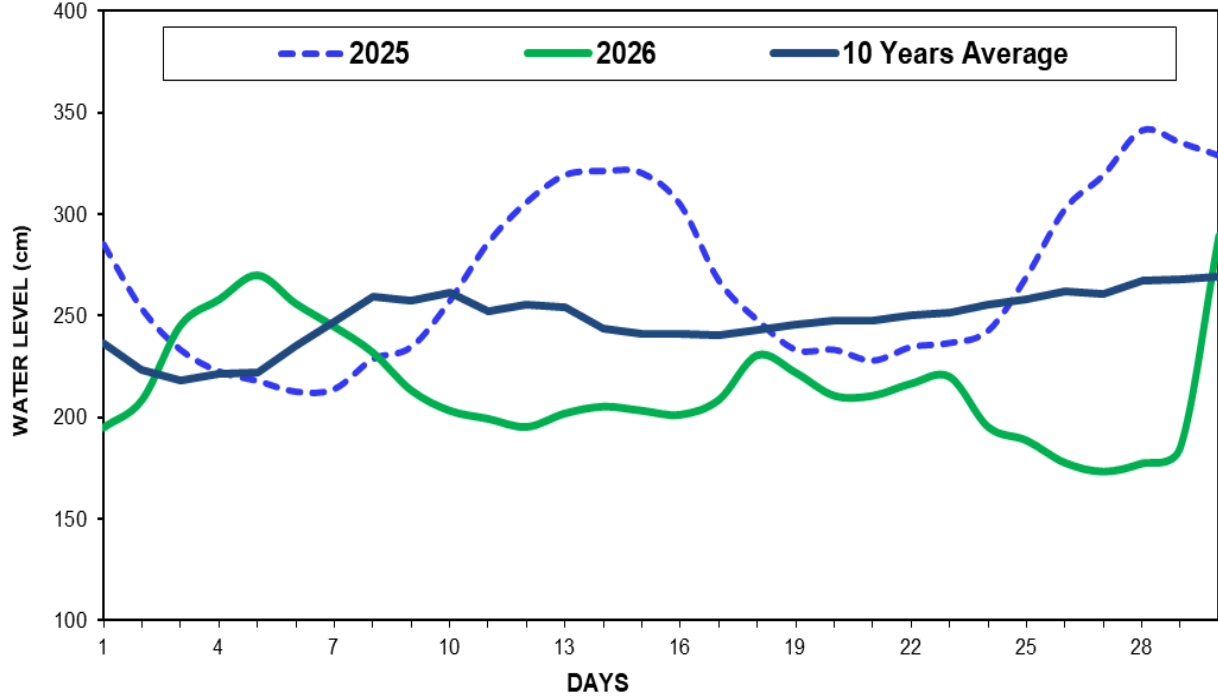
Fig(13) COMPARISON OF APRIL WATER LEVELS OF 2026 WITH APRIL WATER LEVELS OF 2025 AND 10 YEARS AVERAGE (HPA-AN)
