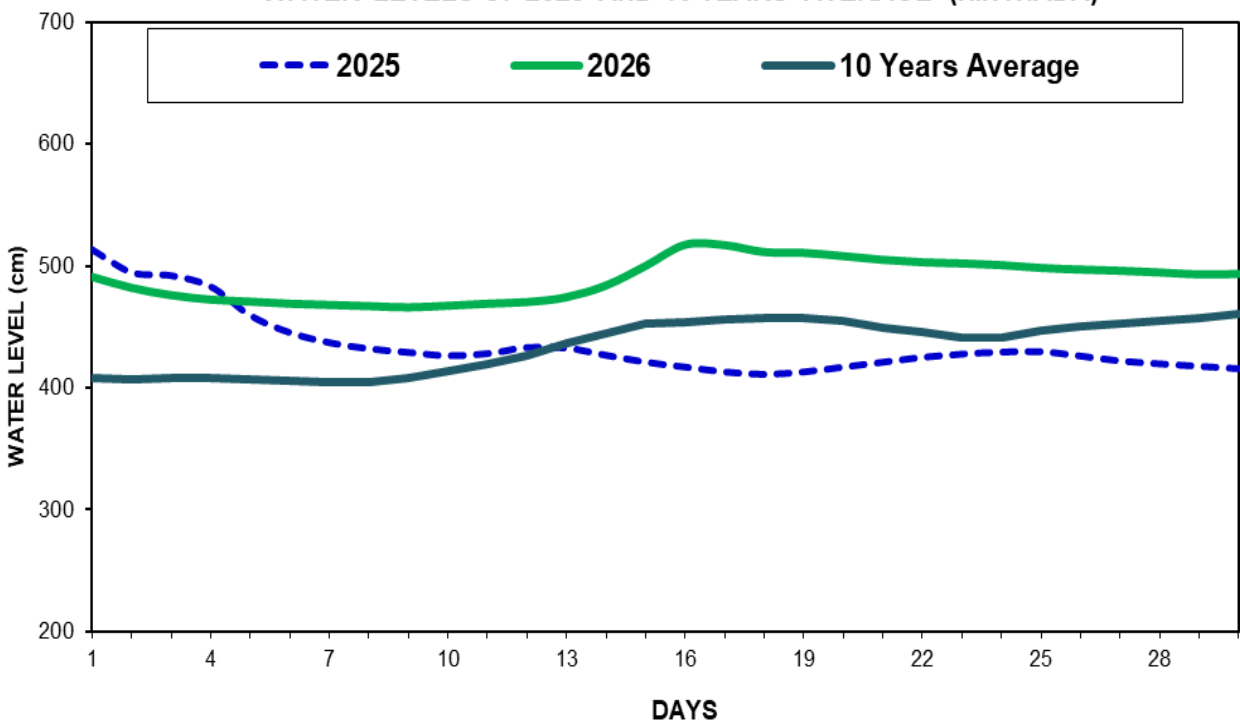
Fig(4) COMPARISON OF APRIL WATER LEVELS OF 2026 WITH APRIL WATER LEVELS OF 2025 AND 10 YEARS AVERAGE (HINTHADA)
