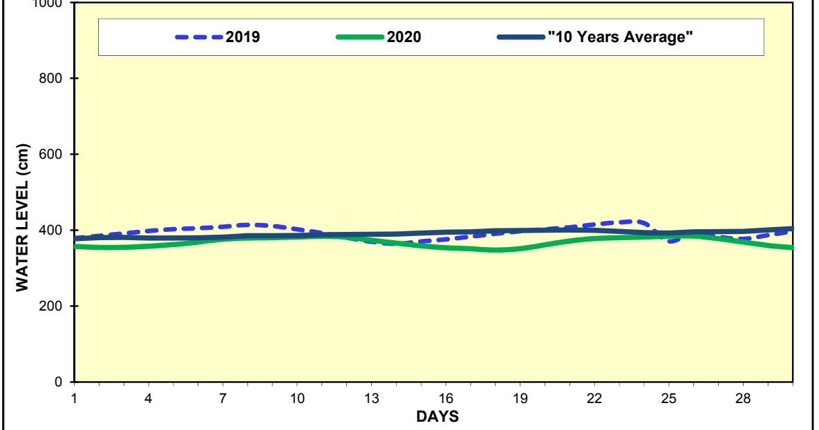
Fig(14) COMPARISON OF APRIL WATER LEVELS OF 2020 WITH APRIL WATER LEVELS OF 2019 AND 10 YEARS AVERAGE(NGATHAINGCHAUNG)
