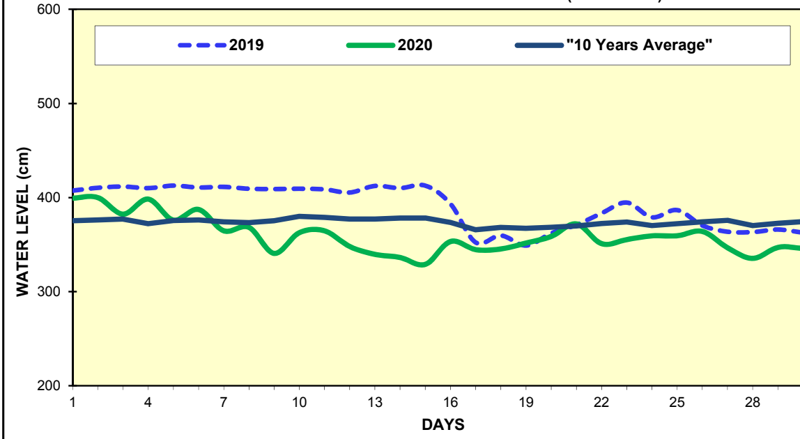
Fig(11) COMPARISON OF APRIL WATER LEVELS OF 2020 WITH APRIL WATER LEVELS OF 2019 AND 10 YEARS AVERAGE (SHWEGYIN)
