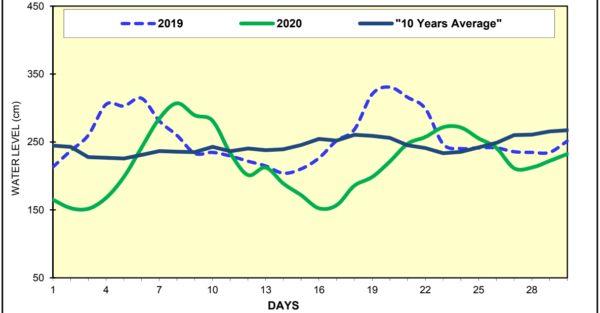
Fig(13) COMPARISON OF APRIL WATER LEVELS OF 2020 WITH APRIL WATER LEVELS OF 2019 AND 10 YEARS AVERAGE (HPA-AN)
