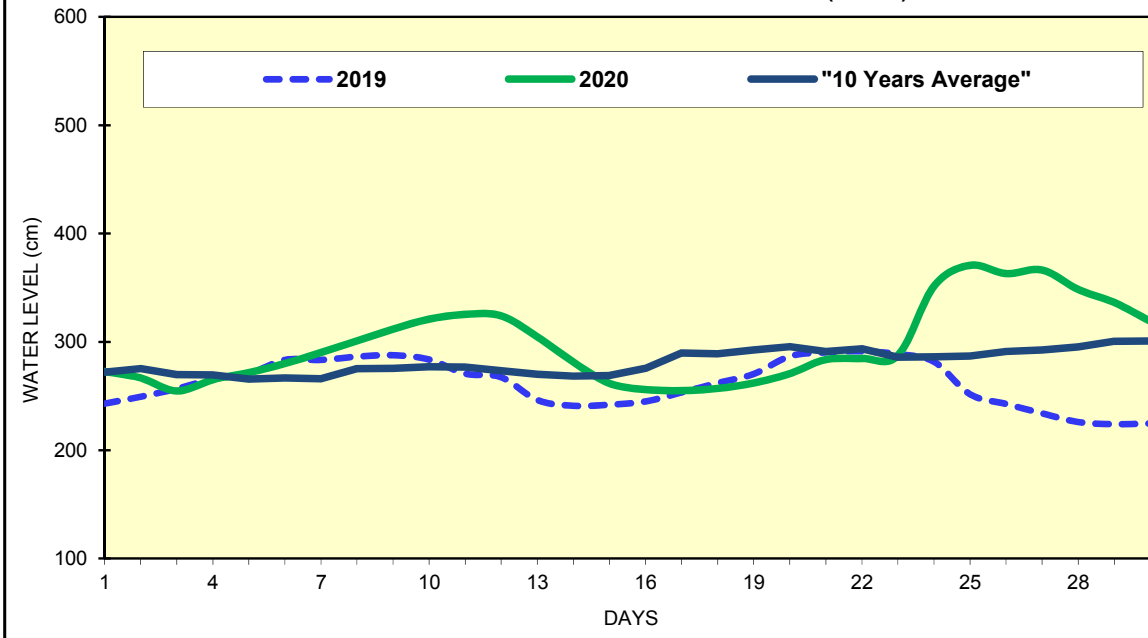
Fig(12) COMPARISON OF APRIL WATER LEVELS OF 2020 WITH APRIL WATER LEVELS OF 2019 AND 10 YEARS AVERAGE (BAGO)
