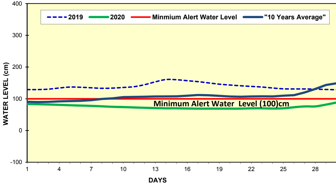
Fig(7) COMPARISON OF APRIL WATER LEVELS OF 2020 WITH APRIL WATER LEVELS OF 2019 AND 10 YEARS AVERAGE (MONYWA)
