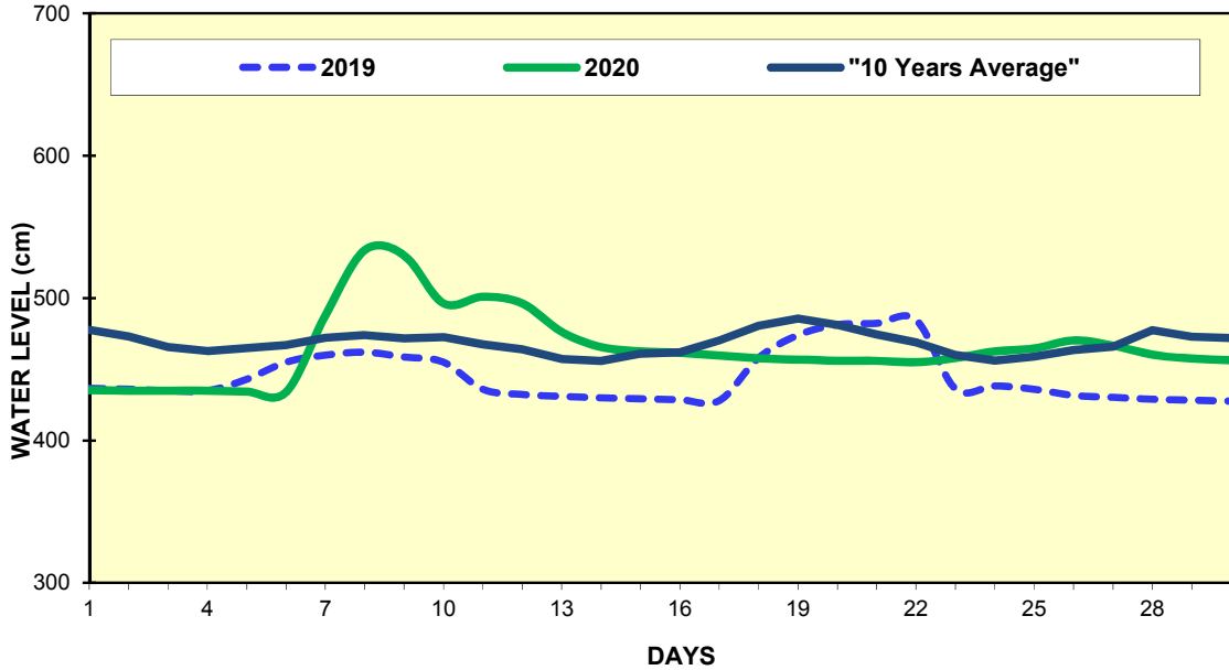
Fig(17) COMPARISON OF APRIL WATER LEVELS OF 2020 WITH APRIL WATER LEVELS OF 2019 AND 10 YEARS AVERAGE (BILIN)
