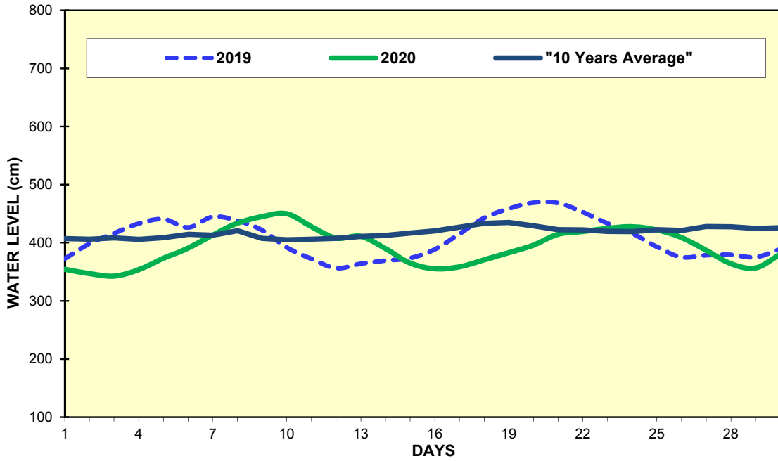
Fig(15) COMPARISON OF APRIL WATER LEVELS OF 2020 WITH APRIL WATER LEVELS OF 2019 AND 10 YEARS AVERAGE (MAUBIN)
