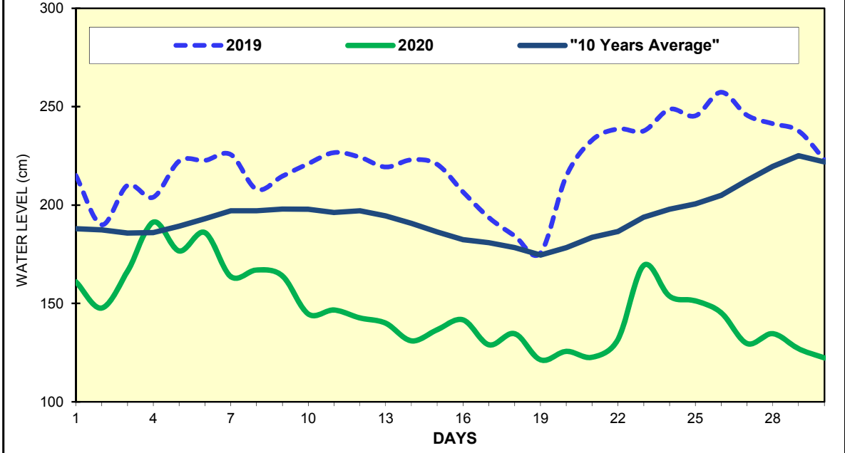
Fig(9) COMPARISON OF APRIL WATER LEVELS OF 2020 WITH APRIL WATER LEVELS OF 2019 AND 10 YEARS AVERAGE (TOUNGOO)
