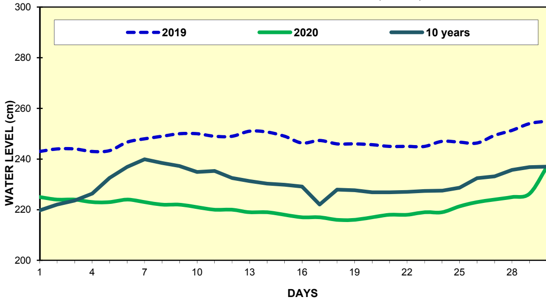
Fig(18) COMPARISON OF APRIL WATER LEVELS OF 2020 WITH APRIL WATER LEVELS OF 2019 AND 10 YEARS AVERAGE (KALAY)
