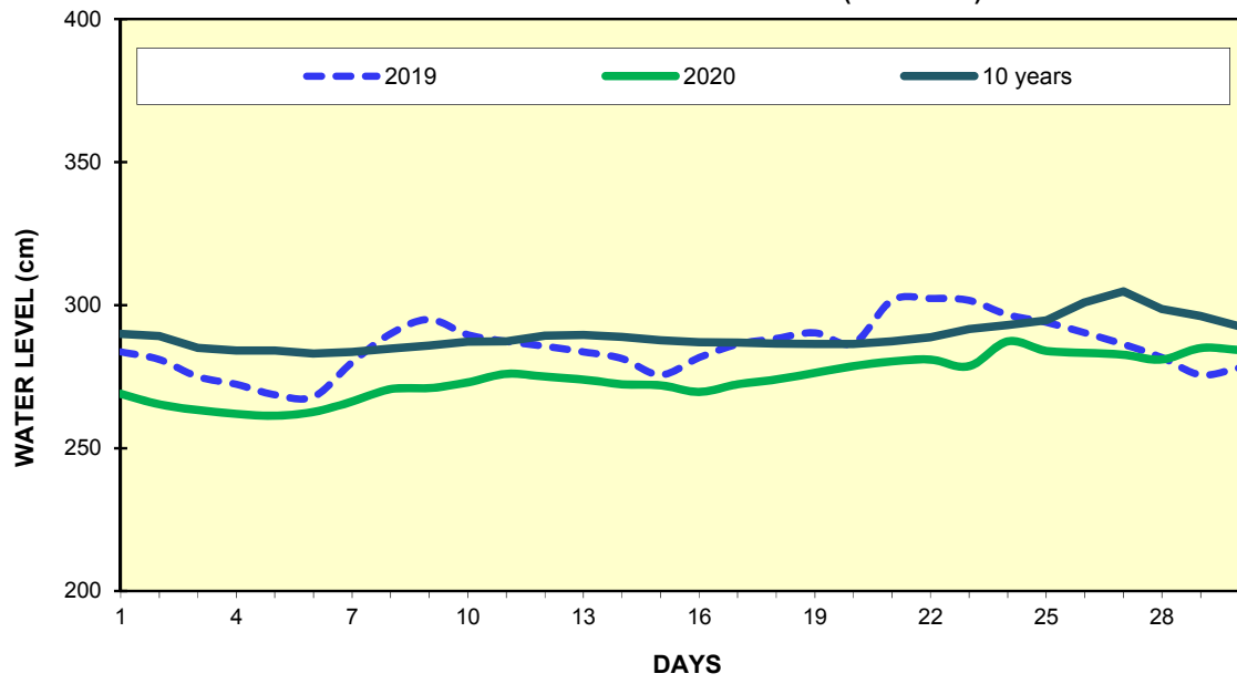
Fig(19) COMPARISON APRIL WATER LEVELS OF 2020 WITH APRIL WATER LEVELS OF 2019 AND 10 YEARS AVERAGE (PALETWA)
