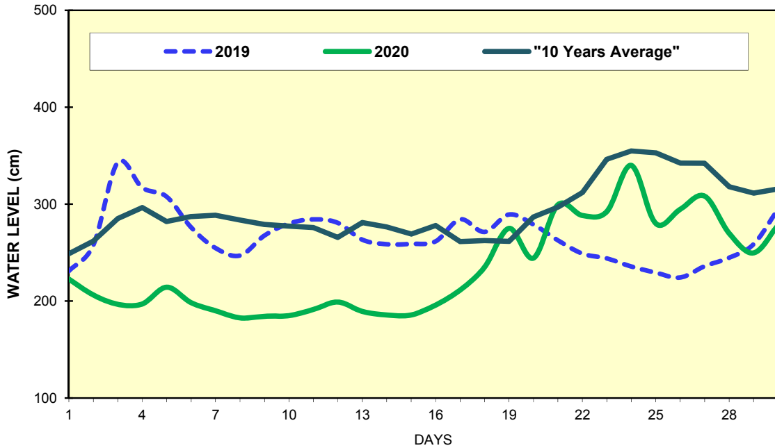
Fig(1) COMPARISON OF APRIL WATER LEVELS OF 2020 WITH APRIL WATER LEVELS OF 2019 AND 10 YEARS AVERAGE (MYITKYINA)
