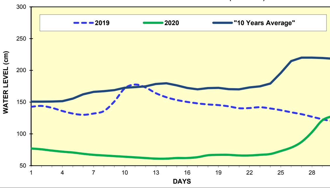
Fig(6) COMPARISON OF APRIL WATER LEVELS OF 2020 WITH APRIL WATER LEVELS OF 2019 AND 10 YEARS AVERAGE (MAWLAIK)
