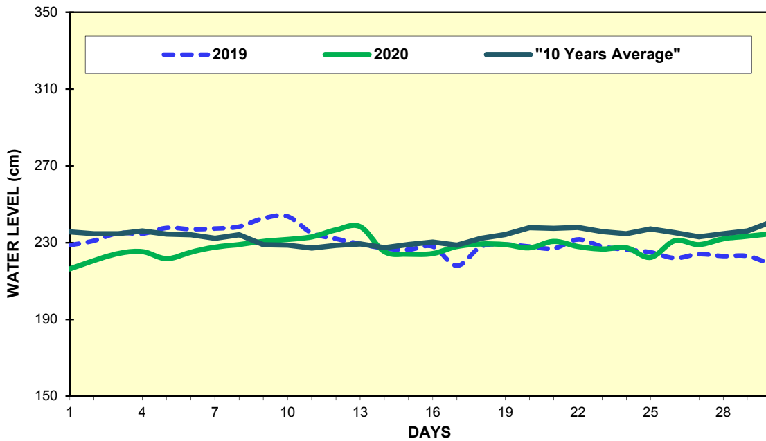
Fig(16) COMPARISON OF APRIL WATER LEVELS OF 2020 WITH APRIL WATER LEVELS OF 2019 AND 10 YEARS AVERAGE (KYAUK TAW)
