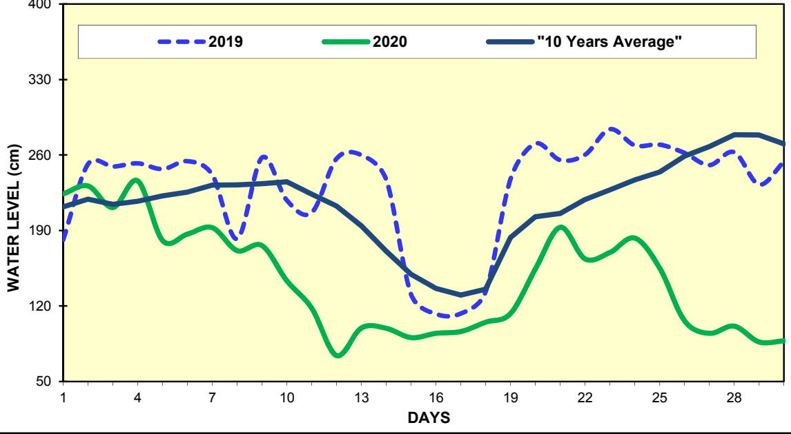
Fig(8) COMPARISON OF APRIL WATER LEVELS OF 2020 WITH APRIL WATER LEVELS OF 2019 AND 10 YEARS AVERAGE (MYITNGE)
