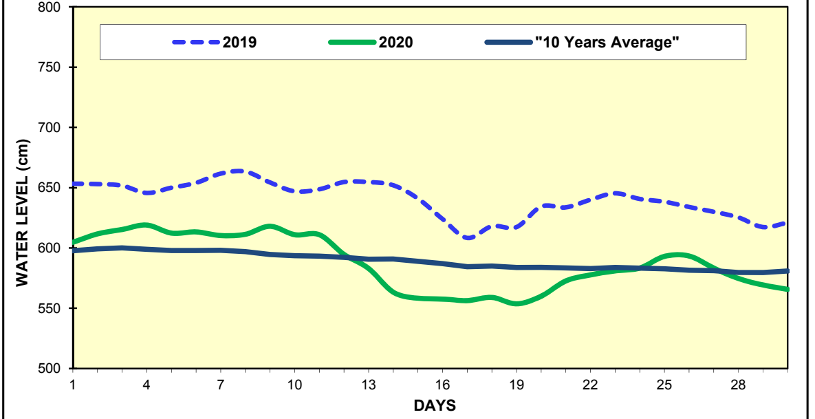
Fig(10) COMPARISON APRIL WATER LEVELS OF 2020 WITH APRIL WATER LEVELS OF 2019 AND 10 YEARS AVERAGE (MADAUK)
