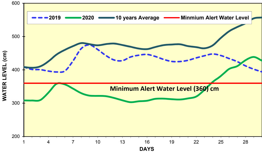
Fig(2) COMPARISON OF APRIL WATER LEVELS OF 2020 WITH APRIL WATER LEVELS OF 2019 AND 10 YEARS AVERAGE (MANDALAY)
