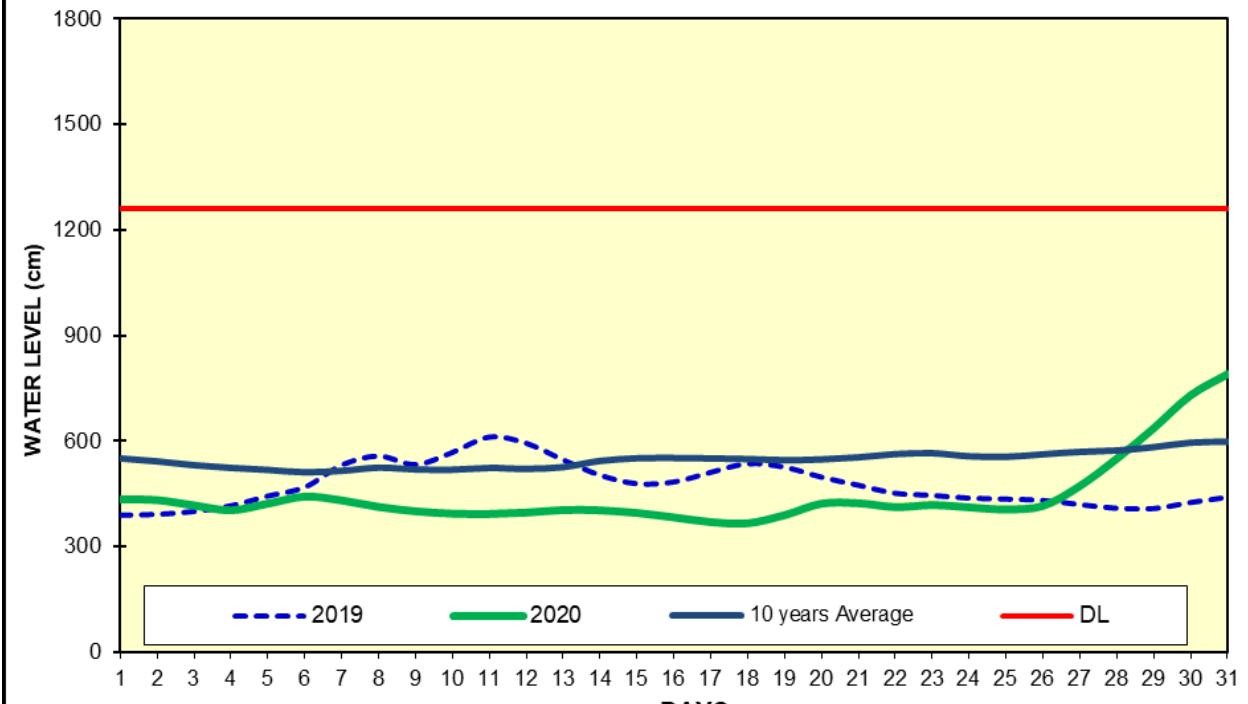
Fig(2) COMPARISON OF MAY WATER LEVELS OF 2020 WITH MAY WATER LEVELS OF 2019 AND 10 YEARS AVERAGE (MANDALAY)
