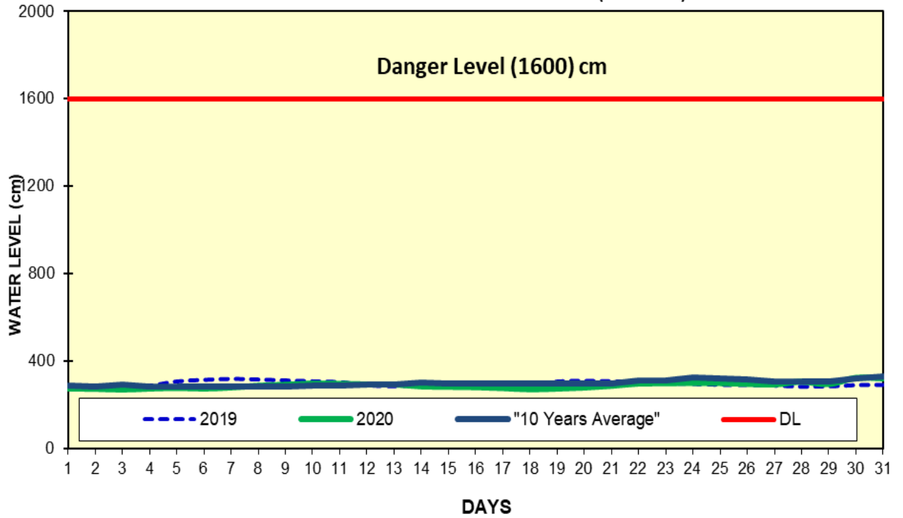
Fig(17) COMPARISON OF MAY WATER LEVELS OF 2020 WITH MAY WATER LEVELS OF 2019 AND 10 YEARS AVERAGE (PALEWA)
