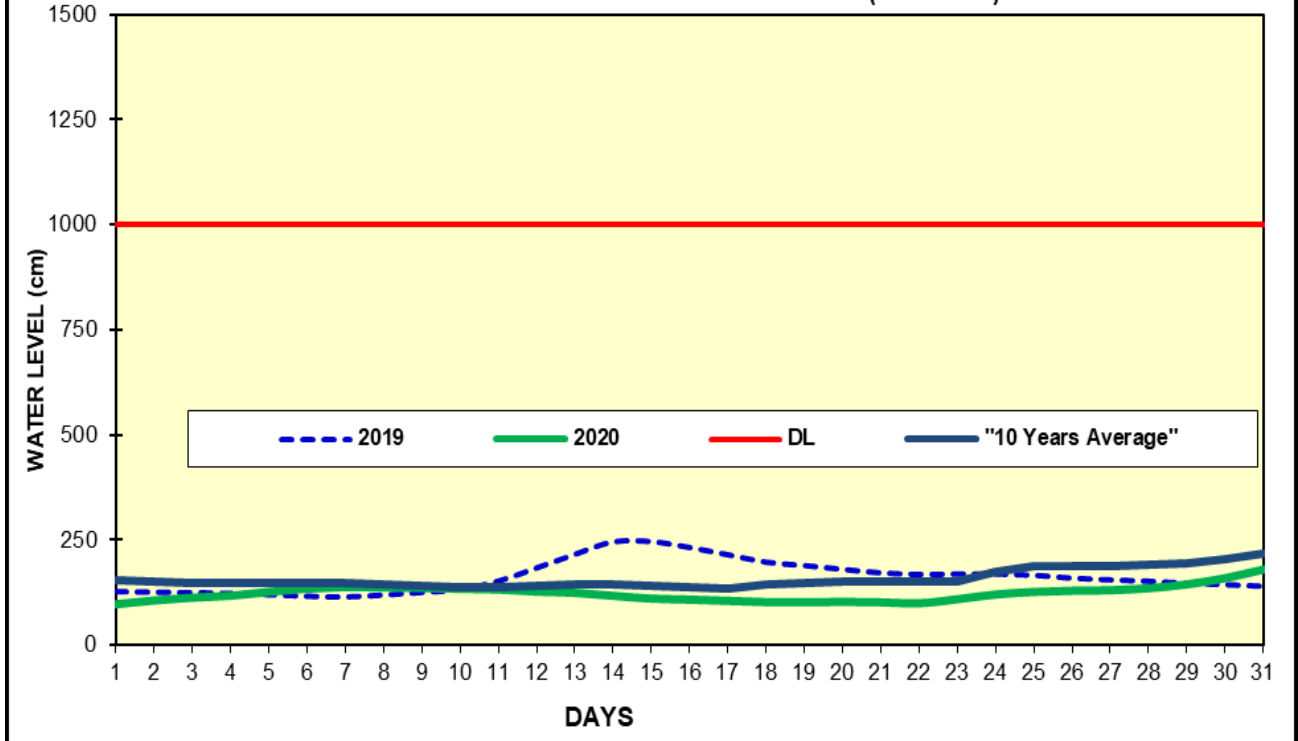
Fig(7) COMPARISON OF MAY WATER LEVELS OF 2020 WITH MAY WATER LEVELS OF 2019 AND 10 YEARS AVERAGE (MONYWA)
