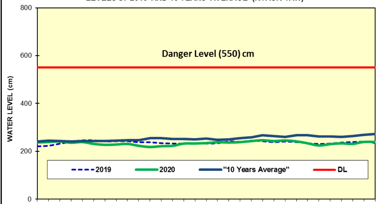
Fig(16) COMPARISON OF MAY WATER LEVELS OF 2020 WITH MAY WATER LEVELS OF 2019 AND 10 YEARS AVERAGE (KYAUK TAW)
