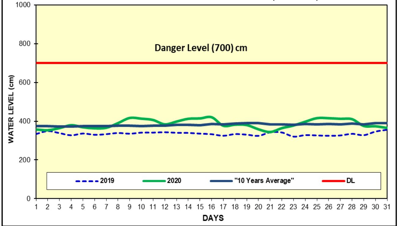
Fig(11) COMPARISON OF MAY WATER LEVELS OF 2020 WITH MAY WATER LEVELS OF 2019 AND 10 YEARS AVERAGE (SHWEGYIN)
