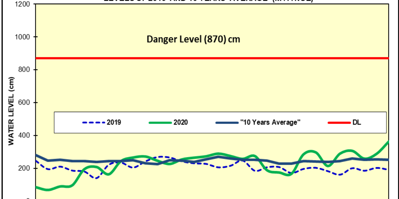
Fig(8) COMPARISON OF MAY WATER LEVELS OF 2020 WITH MAY WATER LEVELS OF 2019 AND 10 YEARS AVERAGE (MYITNGE)
