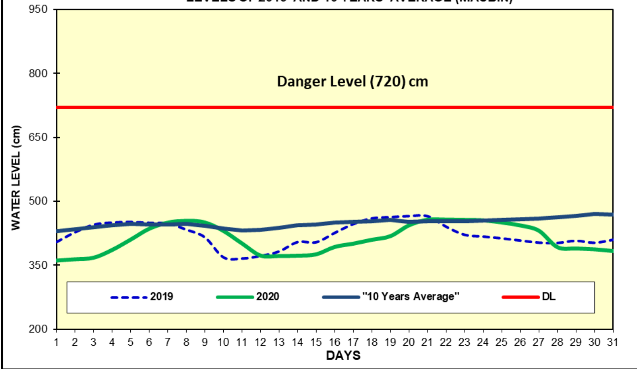
Fig(15) COMPARISON OF MAY WATER LEVELS OF 2020 WITH MAY WATER LEVELS OF 2019 AND 10 YEARS AVERAGE (MAUBIN)
