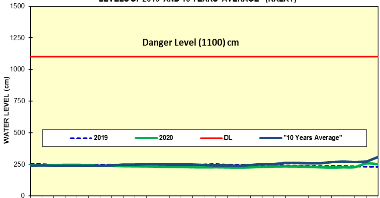
Fig(18) COMPARISON OF MAY WATER LEVELS OF 2020 WITH MAY WATER LEVELS OF 2019 AND 10 YEARS AVERAGE (KALAY)
