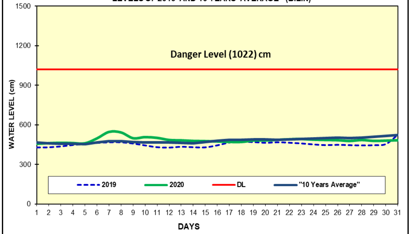
Fig(19) COMPARISON OF MAY WATER LEVELS OF 2020 WITH MAY WATER LEVELS OF 2019 AND 10 YEARS AVERAGE (BILIN)
