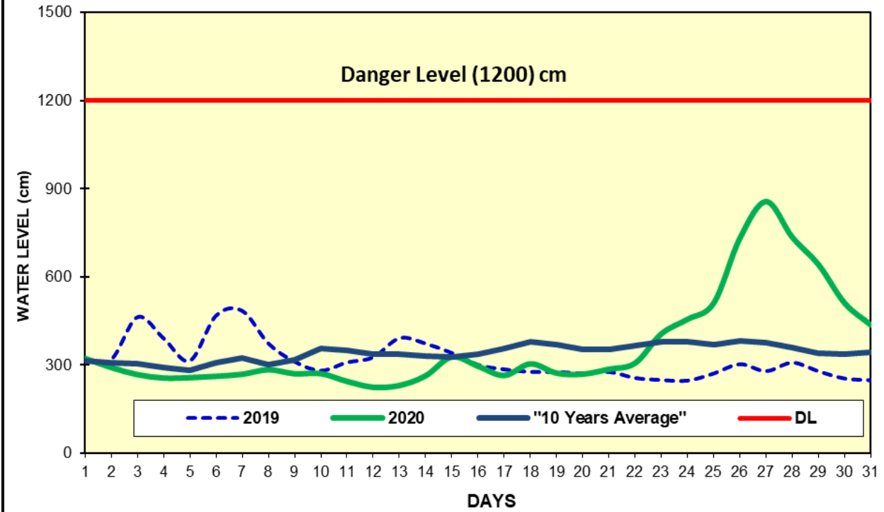
Fig(1) COMPARISON OF MAY WATER LEVELS OF 2020 WITH MAY WATER LEVELS OF 2019 AND 10 YEARS AVERAGE (MYITKYINA)
