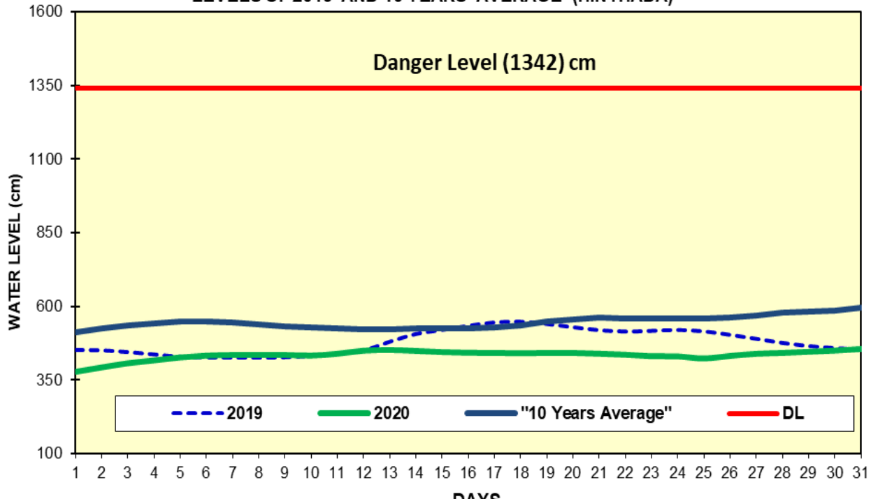
Fig(4) COMPARISON OF MAY WATER LEVELS OF 2020 WITH MAY WATER LEVELS OF 2019 AND 10 YEARS AVERAGE (HINTHADA)
