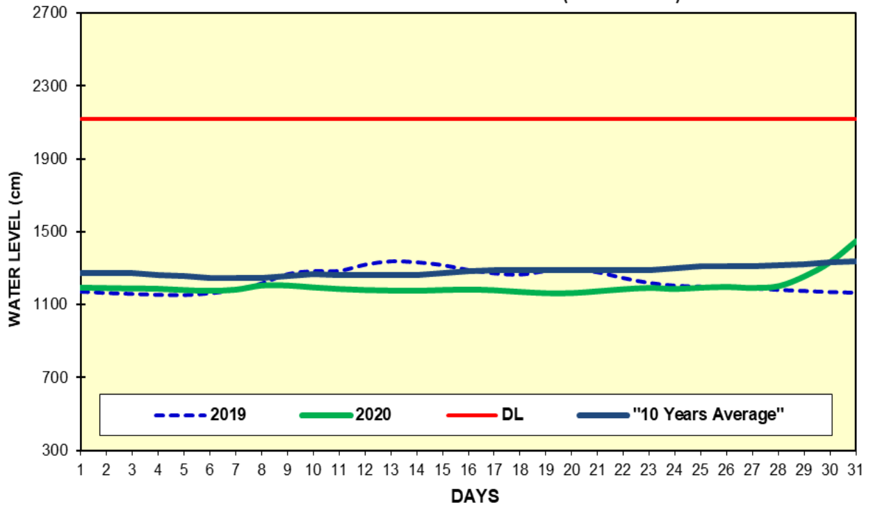
Fig(3) COMPARISON OF MAY WATER LEVELS OF 2020 WITH MAY WATER LEVELS OF 2019 AND 10 YEARS AVERAGE (NYAUNG OO)
