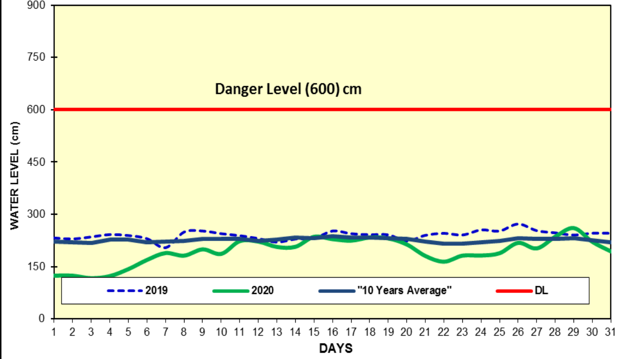
Fig(9) COMPARISON OF MAY WATER LEVELS OF 2020 WITH MAY WATER LEVELS OF 2019 AND 10 YEARS AVERAGE (TOUNGOO)
