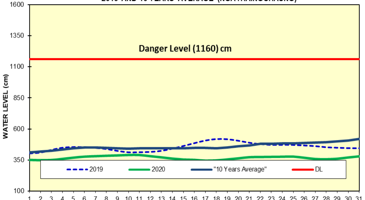
Fig(14) COMPARISON OF MAY WATER LEVELS OF 2020 WITH MAY LEVELS OF 2019 AND 10 YEARS AVERAGE (NGATHAINGCHAUNG)
