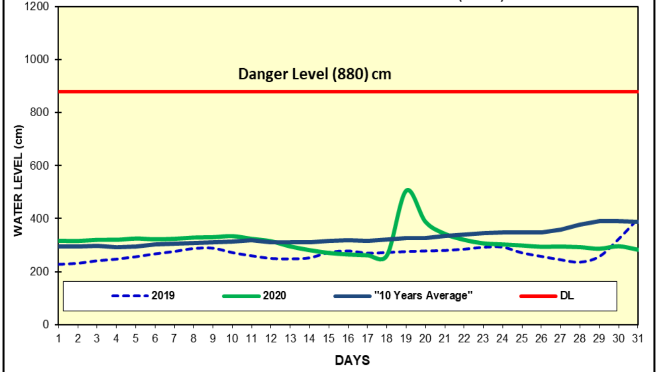
Fig(12) COMPARISON OF MAY WATER LEVELS OF 2020 WITH MAY WATER LEVELS OF 2019 AND 10 YEARS AVERAGE (BAGO)
