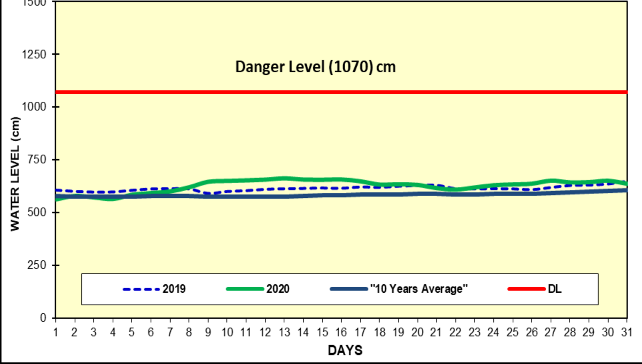
Fig(10) COMPARISON OF MAY WATER LEVELS OF 2020 WITH MAY WATER LEVELS OF 2019 AND 10 YEARS AVERAGE (MADAUK)
