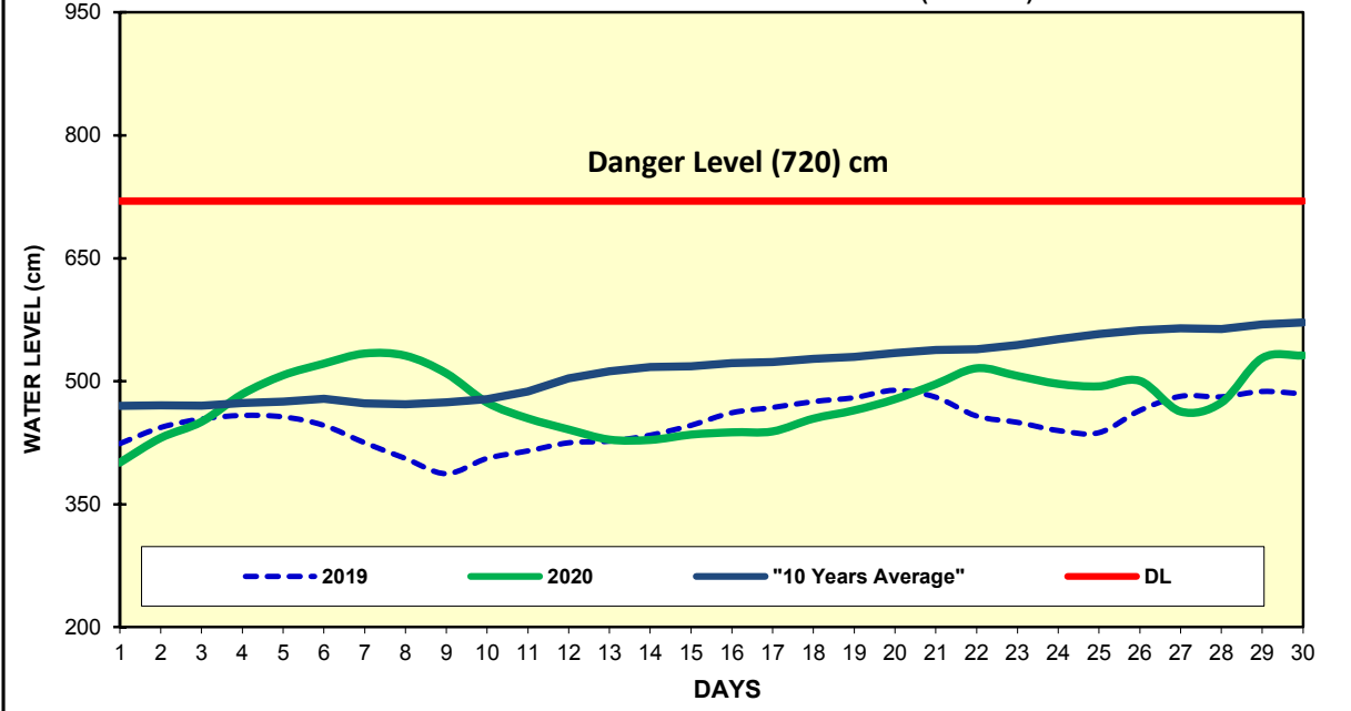
Fig(15) COMPARISON OF JUNE WATER LEVELS OF 2020 WITH JUNE WATER LEVELS OF 2019 AND 10 YEARS AVERAGE (MAUBIN)
