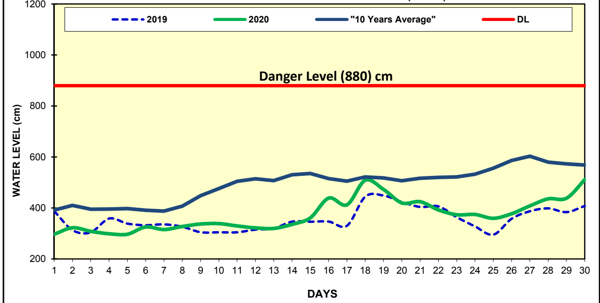
Fig(12) COMPARISON OF JUNE WATER LEVELS OF 2020 WITH JUNE WATER LEVELS OF 2019 AND 10 YEARS AVERAGE (BAGO)
