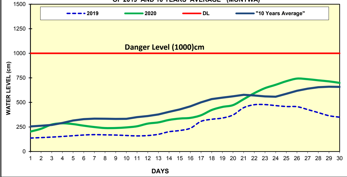
Fig(7) COMPARISON OF JUNE WATER LEVELS OF 2020 WITH JUNE WATER LEVELS OF 2019 AND 10 YEARS AVERAGE (MONYWA)
