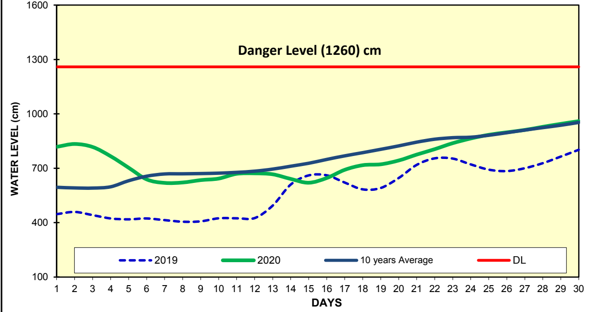
Fig(2) COMPARISON OF JUNE WATER LEVELS OF 2020 WITH JUNE WATER LEVELS OF 2019 AND 10 YEARS AVERAGE (MANDALAY)
