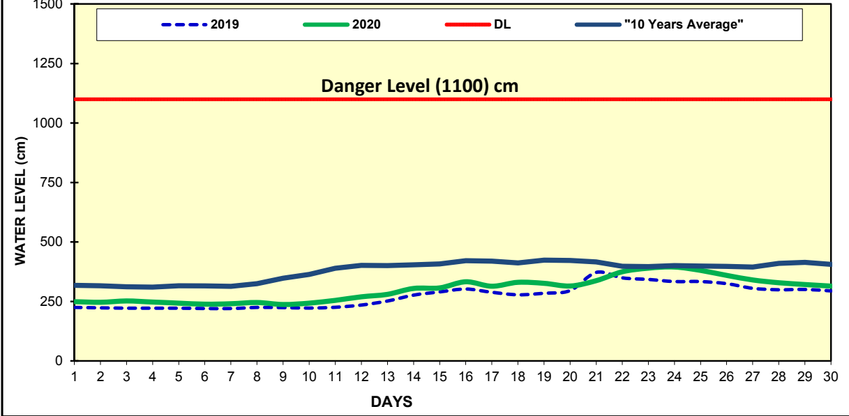
Fig(18) COMPARISON OF JUNE WATER LEVELS OF 2020 WITH JUNE WATER LEVELS OF 2019 AND 10 YEARS AVERAGE (KALAY)
