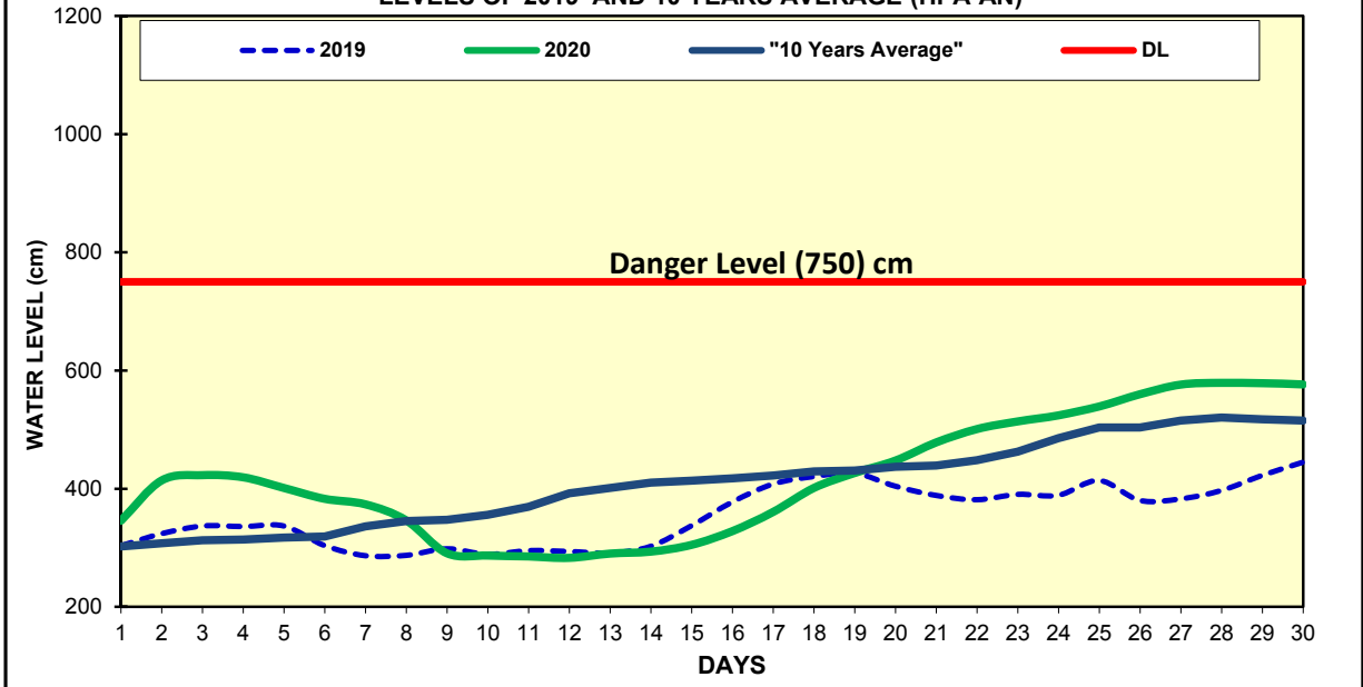
Fig(13) COMPARISON OF JUNE WATER LEVELS OF 2020 WITH JUNE WATER LEVELS OF 2019 AND 10 YEARS AVERAGE (HPA-AN)
