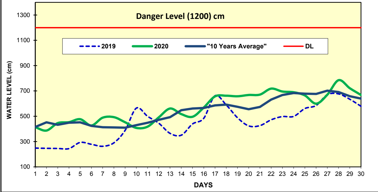
Fig(1) COMPARISON OF JUNE WATER LEVELS OF 2020 WITH JUNE WATER LEVELS OF 2019 AND 10 YEARS AVERAGE (MYITKYINA)
