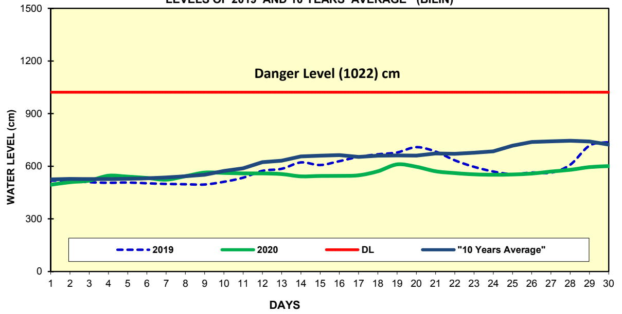
Fig(19) COMPARISON OF JUNE WATER LEVELS OF 2020 WITH JUNE WATER LEVELS OF 2019 AND 10 YEARS AVERAGE (BILIN)
