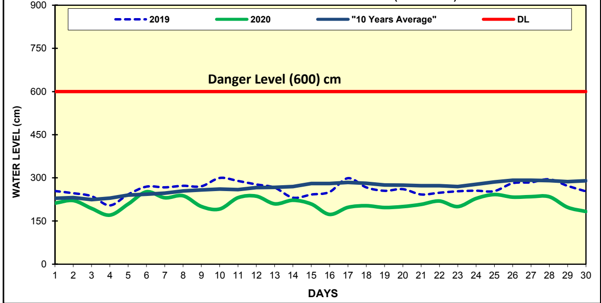
Fig(9) COMPARISON OF JUNE WATER LEVELS OF 2020 WITH JUNE WATER LEVELS OF 2019 AND 10 YEARS AVERAGE (TOUNGOO)
