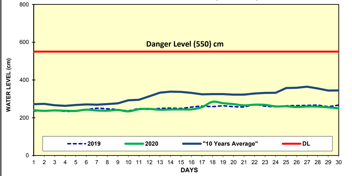
Fig(16) COMPARISON OF JUNE WATER LEVELS OF 2020 WITH JUNE WATER LEVELS OF 2019 AND 10 YEARS AVERAGE (KYAUK TAW)
