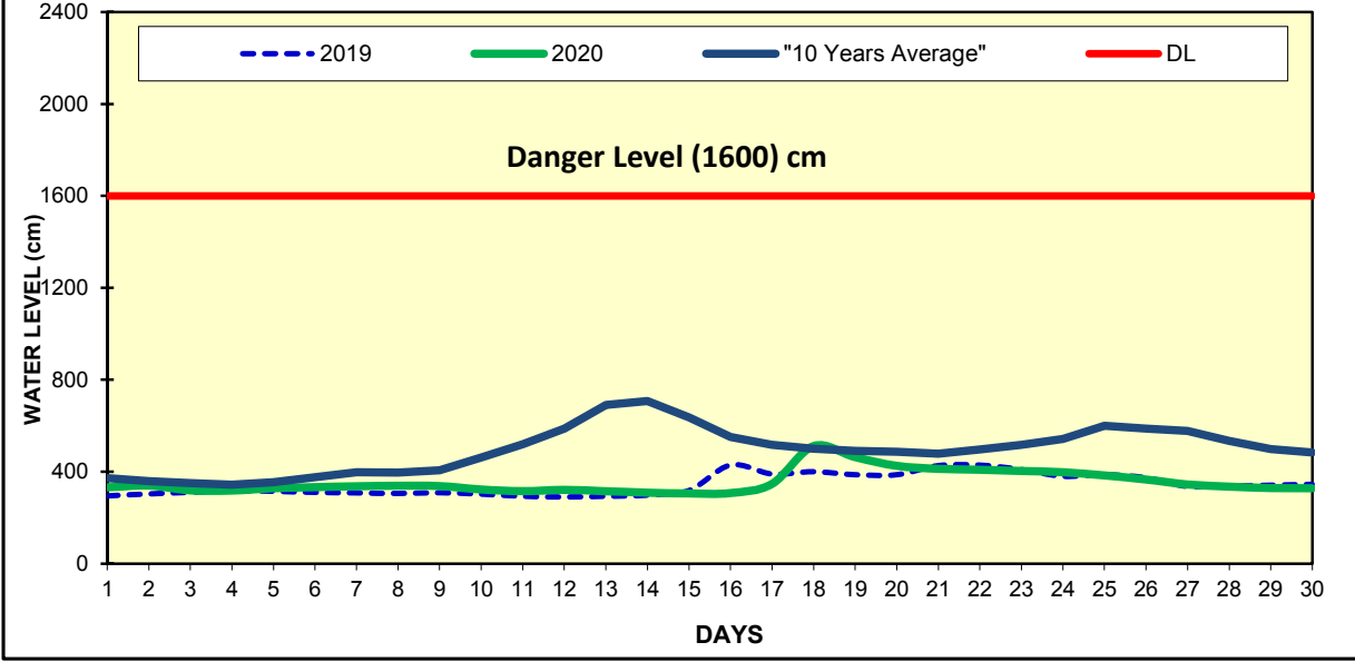
Fig(17) COMPARISON OF JUNE WATER LEVELS OF 2020 WITH JUNE WATER LEVELS OF 2019 AND 10 YEARS AVERAGE (PALEWA)
