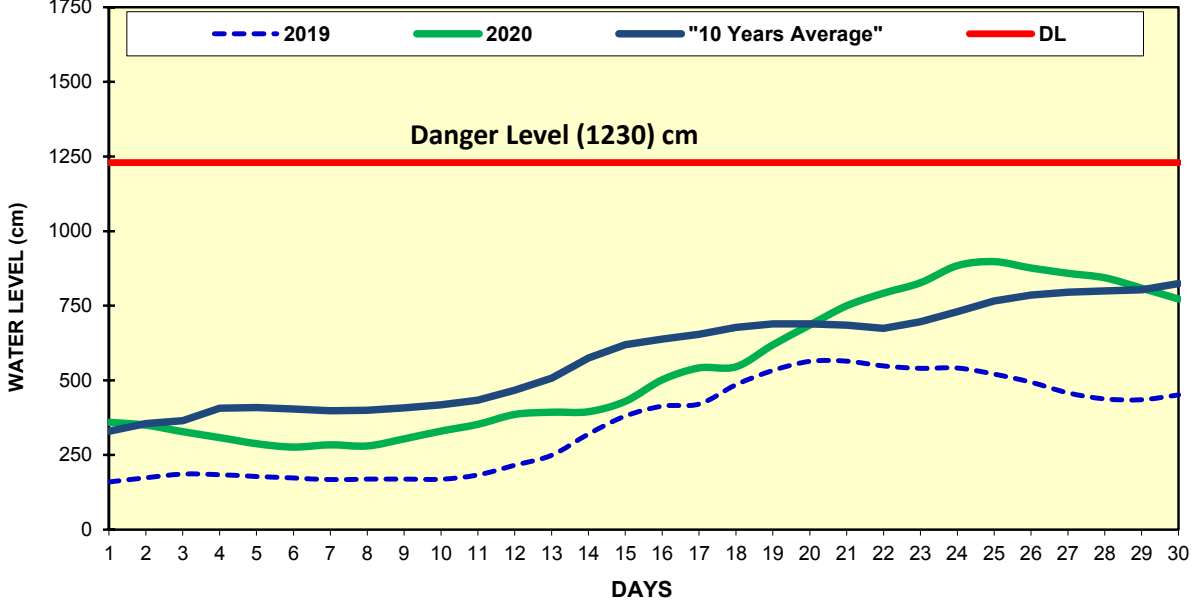
Fig(6) COMPARISON OF JUNE WATER LEVELS OF 2020 WITH JUNE WATER LEVELS OF 2019 AND 10 YEARS AVERAGE (MAWLAIK)
