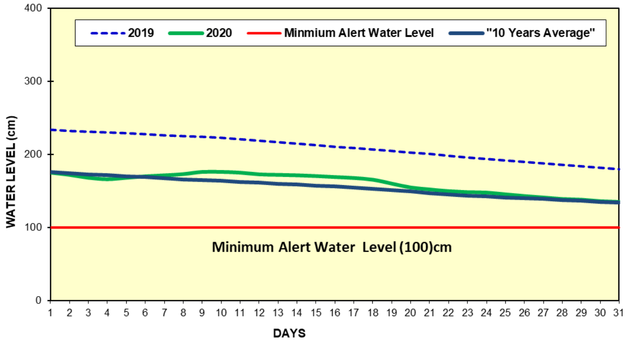
Fig(7) COMPARISON OF JANUARY WATER LEVELS OF 2020 WITH JANUARY WATER LEVELS OF 2019 AND 10 YEARS AVERAGE (MONYWA)
