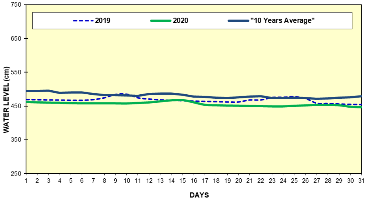
Fig(17) COMPARISON OF JANUARY WATER LEVELS OF 2020 WITH JANUARY WATER LEVELS OF 2019 AND 10 YEARS AVERAGE (BILIN)
