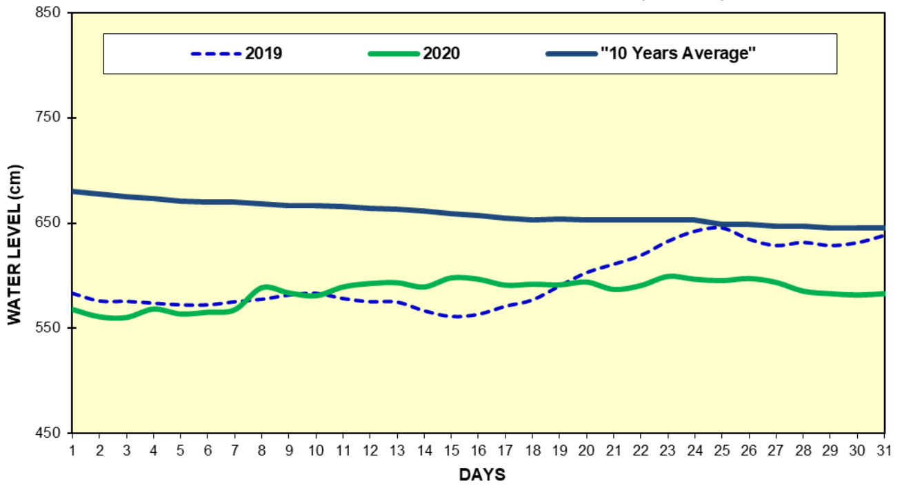
Fig(10) COMPARISON OF JANUARY WATER LEVELS OF 2020 WITH JANUARY WATER LEVELS OF 2019 AND 10 YEARS AVERAGE (MADAUK)
