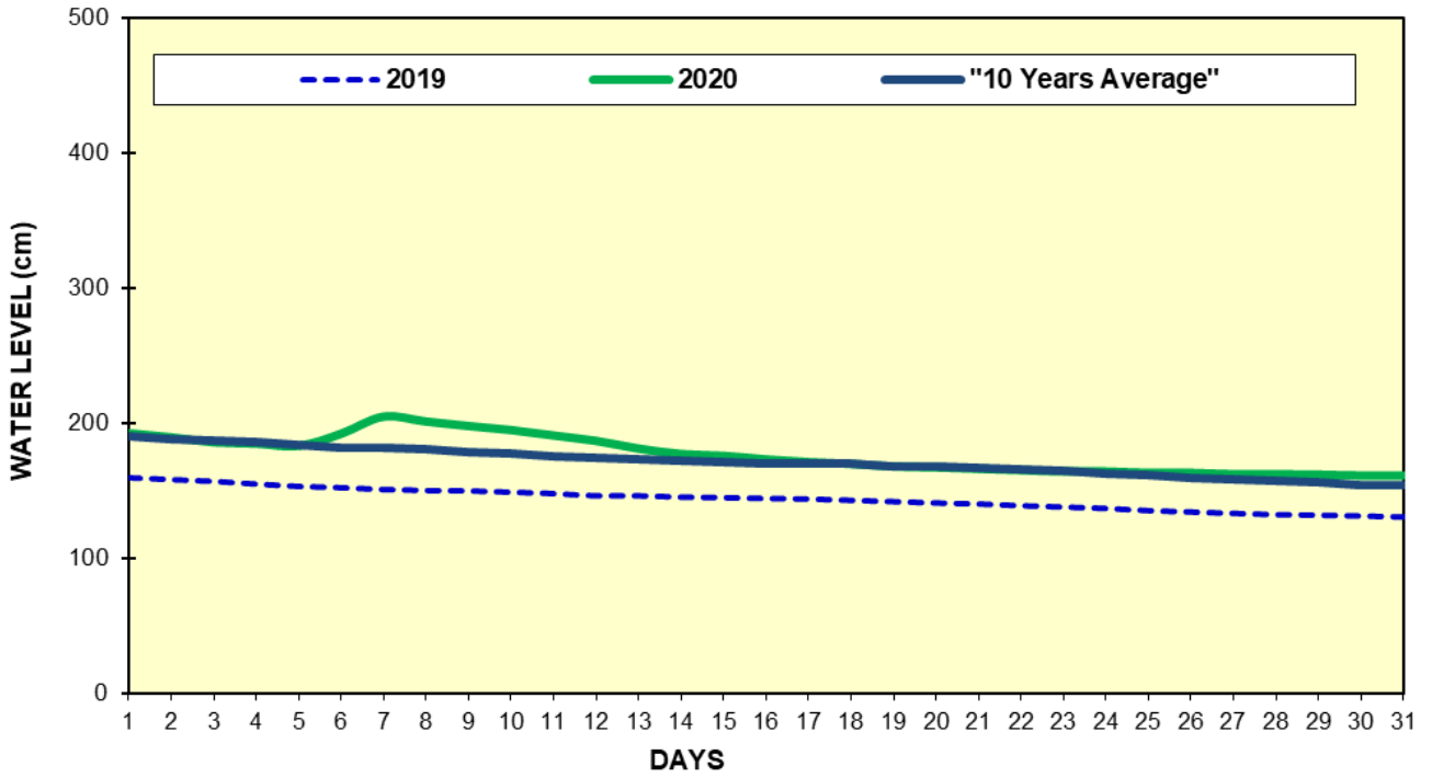
Fig(5) COMPARISON OF JANUARY WATER LEVELS OF 2020 WITH JANUARY WATER LEVELS OF 2019 AND 10 YEARS AVERAGE (HKAMTI)
