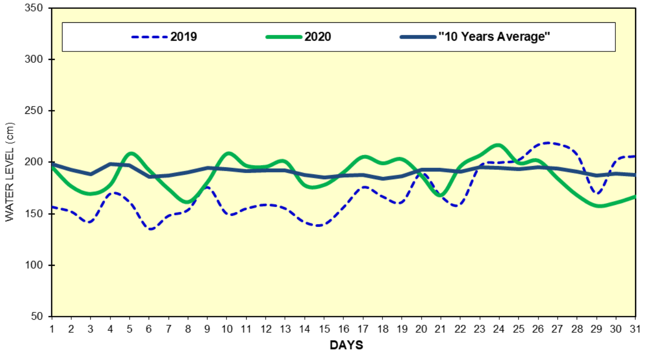
Fig(9) COMPARISON OF JANUARY WATER LEVELS OF 2020 WITH JANUARY WATER LEVELS OF 2019 AND 10 YEARS AVERAGE (TOUNGOO)
