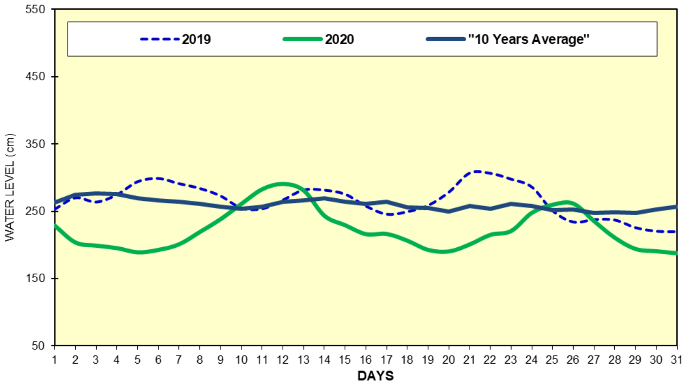
Fig(13) COMPARISON OF JANUARY WATER LEVELS OF 2020 WITH JANUARY WATER LEVELS OF 2019 AND 10 YEARS AVERAGE (HPA-AN)
