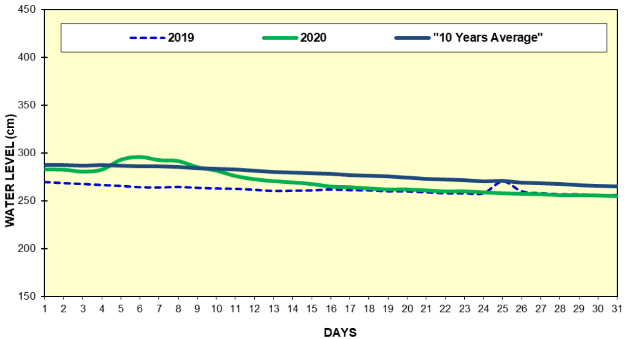
Fig(18) COMPARISON OF JANUARY WATER LEVELS OF 2020 WITH JANUARY WATER LEVELS OF 2019 AND 10 YEARS AVERAGE (KALAY)
