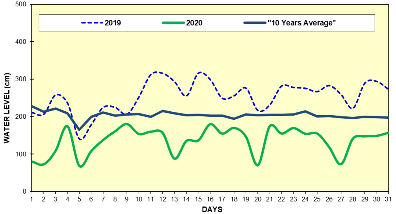
Fig(8) COMPARISON OF JANUARY WATER LEVELS OF 2020 WITH JANUARY WATER LEVELS OF 2019 AND 10 YEARS AVERAGE (MYITNGE)
