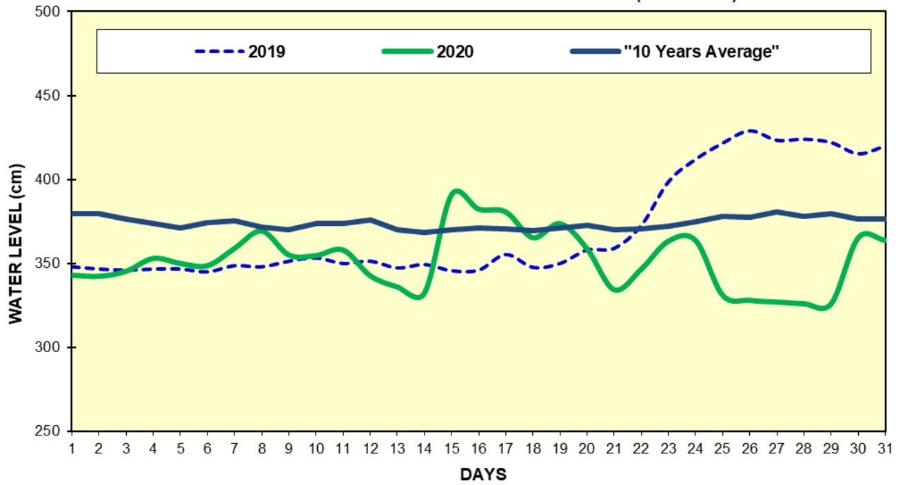
Fig(11) COMPARISON OF JANUARY WATER LEVELS OF 2020 WITH JANUARY WATER LEVELS OF 2019 AND 10 YEARS AVERAGE (SHWEGYIN)
