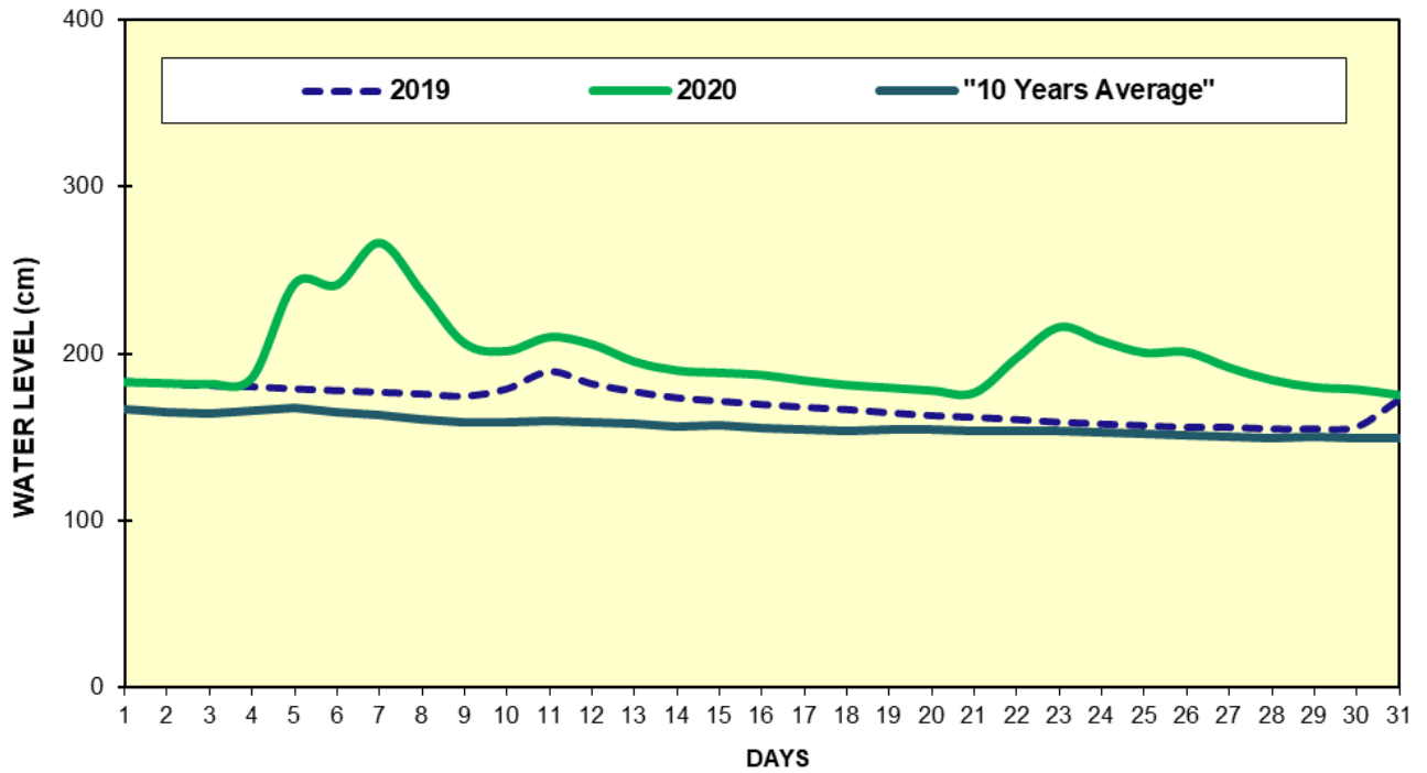
Fig(1) COMPARISON OF JANUARY WATER LEVELS OF 2020 WITH JANUARY WATER LEVELS OF 2019 AND 10 YEARS AVERAGE (MYITKYINA)
