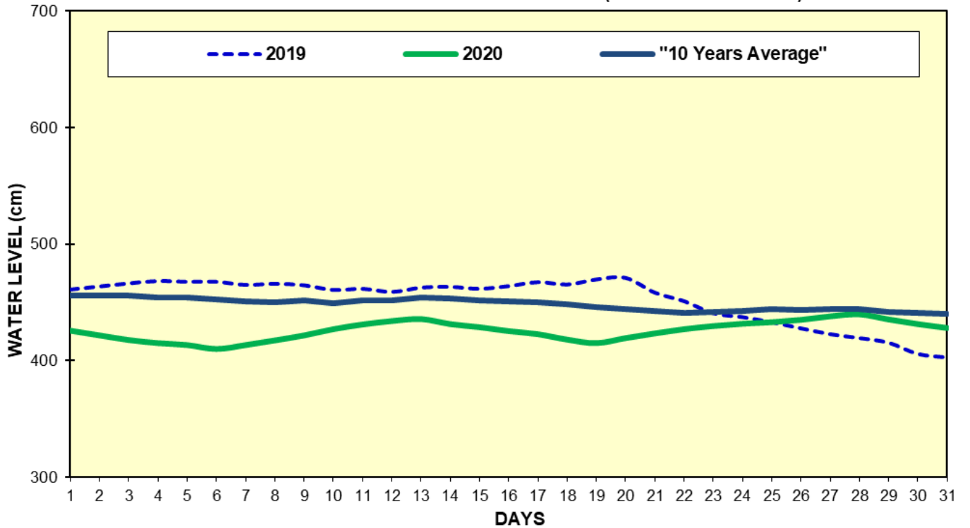
Fig(14) COMPARISON OF JANUARY WATER LEVELS OF 2020 WITH JANUARY LEVELS OF 2019 AND 10 YEARS AVERAGE (NGATHAINGCHAUNG)
