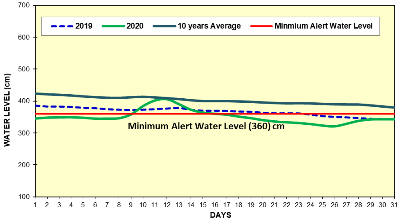
Fig(2) COMPARISON OF JANUARY WATER LEVELS OF 2020 WITH JANUARY WATER LEVELS OF 2019 AND 10 YEARS AVERAGE (MANDALAY)
