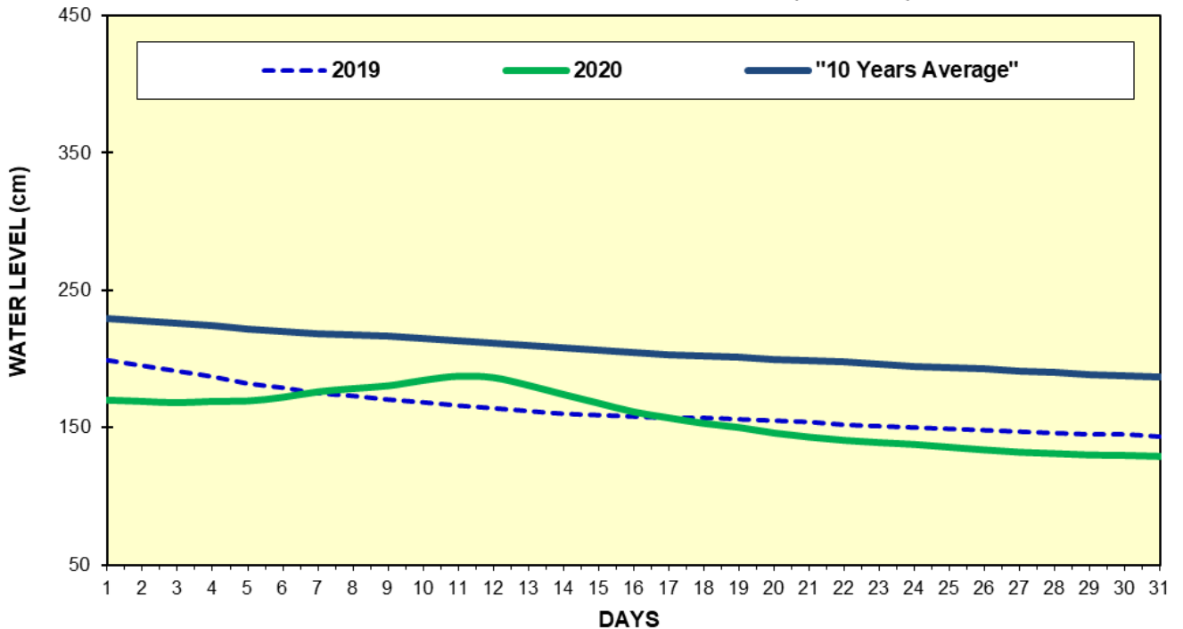
Fig(6) COMPARISON OF JANUARY WATER LEVELS OF 2020 WITH JANUARY WATER LEVELS OF 2019 AND 10 YEARS AVERAGE (MAWLAIK)
