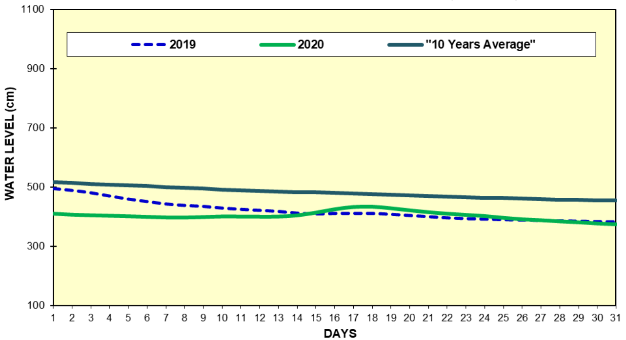
Fig(4) COMPARISON OF JANUARY WATER LEVELS OF 2020 WITH JANUARY WATER LEVELS OF 2019 AND 10 YEARS AVERAGE (HINTHADA)
