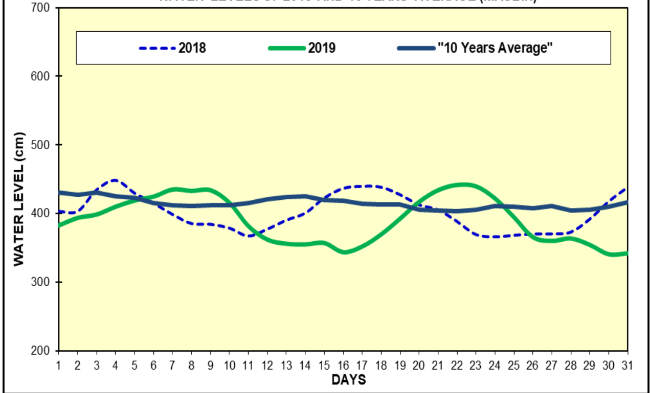
Fig(15) COMPARISON OF JANUARY WATER LEVELS OF 2019 WITH JANUARY WATER LEVELS OF 2018 AND 10 YEARS AVERAGE (MAUBIN)
