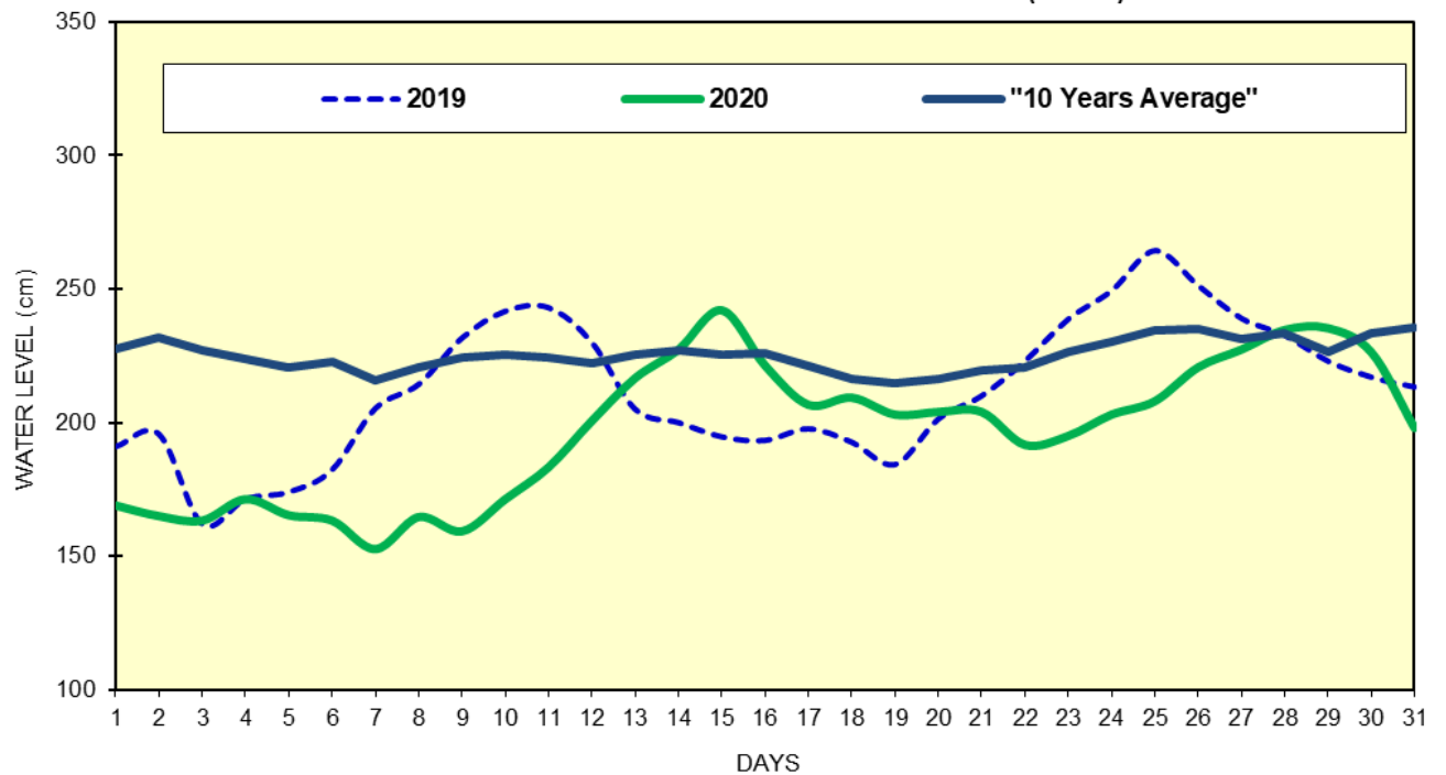
Fig(12) COMPARISON OF JANUARY WATER LEVELS OF 2020 WITH JANUARY WATER LEVELS OF 2019 AND 10 YEARS AVERAGE (BAGO)
