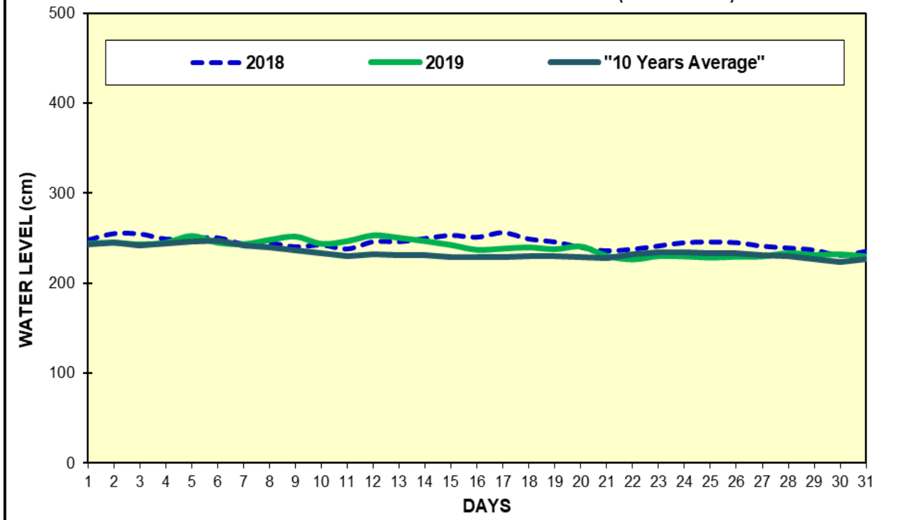
Fig(16) COMPARISON OF JANUARY WATER LEVELS OF 2019 WITH JANUARY WATER LEVELS OF 2018 AND 10 YEARS AVERAGE (KYAUK TAW)
