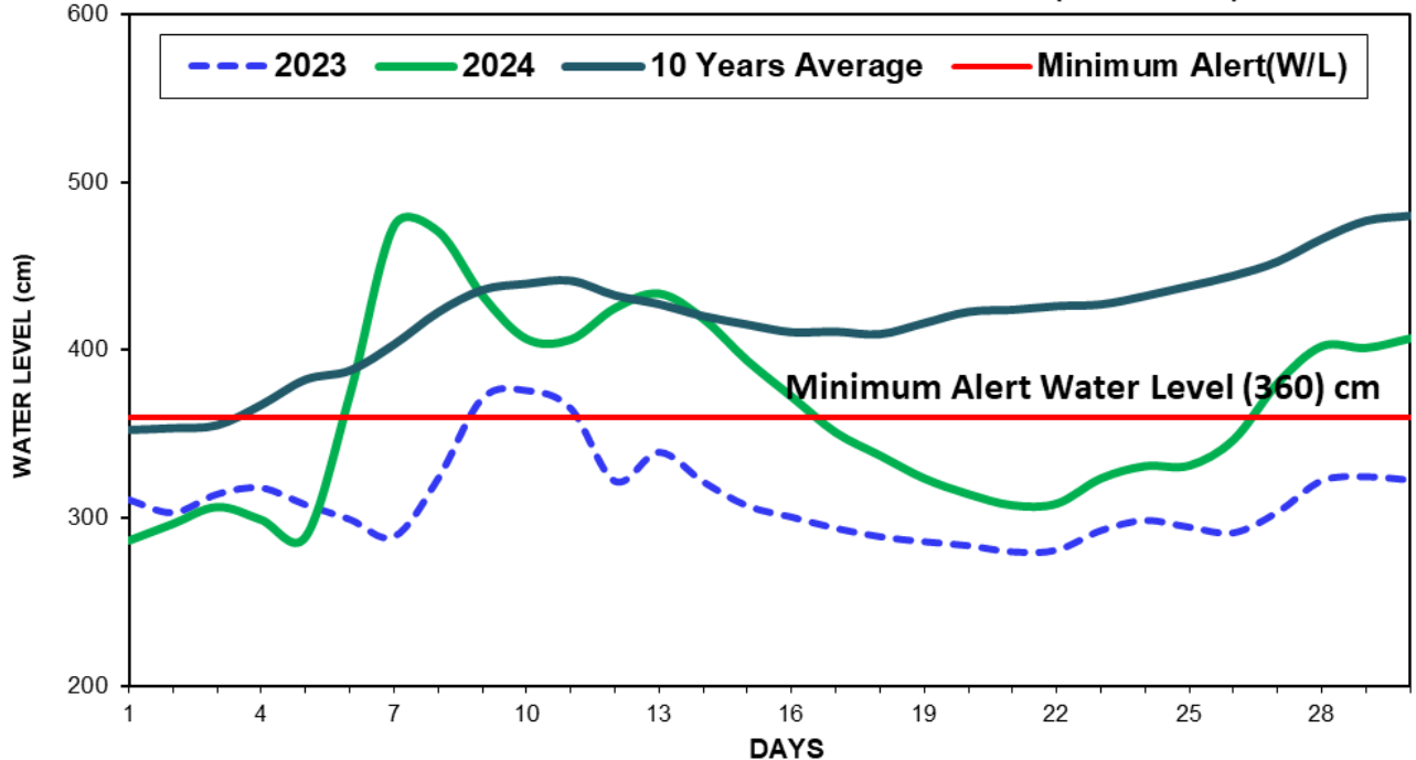
Fig(2) COMPARISON OF APRIL WATER LEVELS OF 2024 WITH APRIL WATER LEVELS OF 2023 AND 10 YEARS AVERAGE (MANDALAY)
