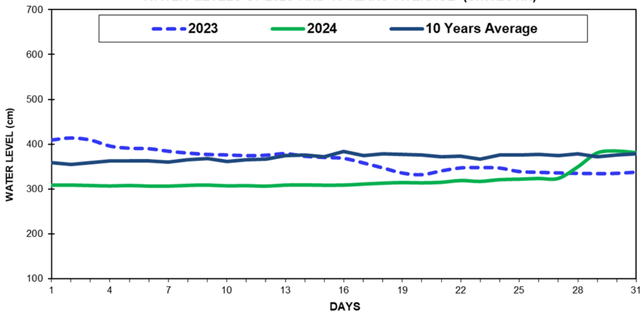
Fig(11) COMPARISON OF MAY WATER LEVELS OF 2024 WITH MAY WATER LEVELS OF 2023 AND 10 YEARS AVERAGE (SHWEGYIN)
