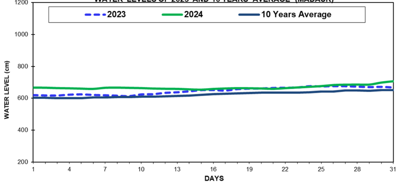
Fig(10) COMPARISON OF MAY WATER LEVELS OF 2024 WITH MAY WATER LEVELS OF 2023 AND 10 YEARS AVERAGE (MADAUK)
