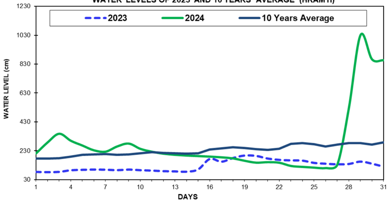
Fig(5) COMPARISON OF MAY WATER LEVELS OF 2024 WITH MAY WATER LEVELS OF 2023 AND 10 YEARS AVERAGE (HKAMTI)
