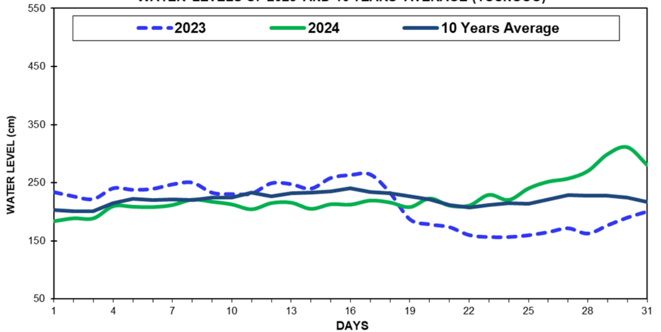
Fig(9) COMPARISON OF MAY WATER LEVELS OF 2024 WITH MAY WATER LEVELS OF 2023 AND 10 YEARS AVERAGE (TOUNGOO)
