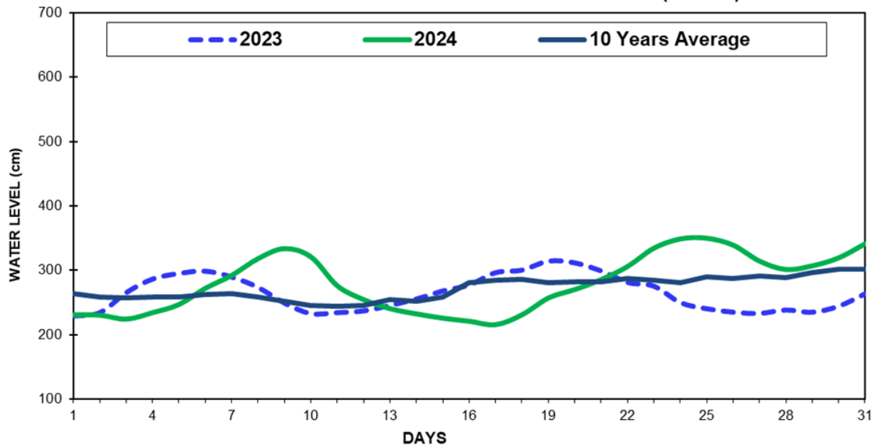
Fig(13) COMPARISON OF MAY WATER LEVELS OF 2024 WITH MAY WATER LEVELS OF 2023 AND 10 YEARS AVERAGE (HPA-AN)
