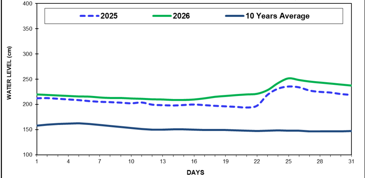
Fig(6) COMPARISON OF MARCH WATER LEVELS OF 2026 WITH MARCH WATER LEVELS OF 2025 AND 10 YEARS AVERAGE (MAWLAIK)
