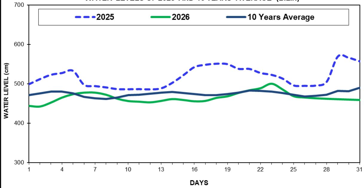
Fig(17) COMPARISON OF MARCH WATER LEVELS OF 2026 WITH MARCH WATER LEVELS OF 2025 AND 10 YEARS AVERAGE (BILIN)
