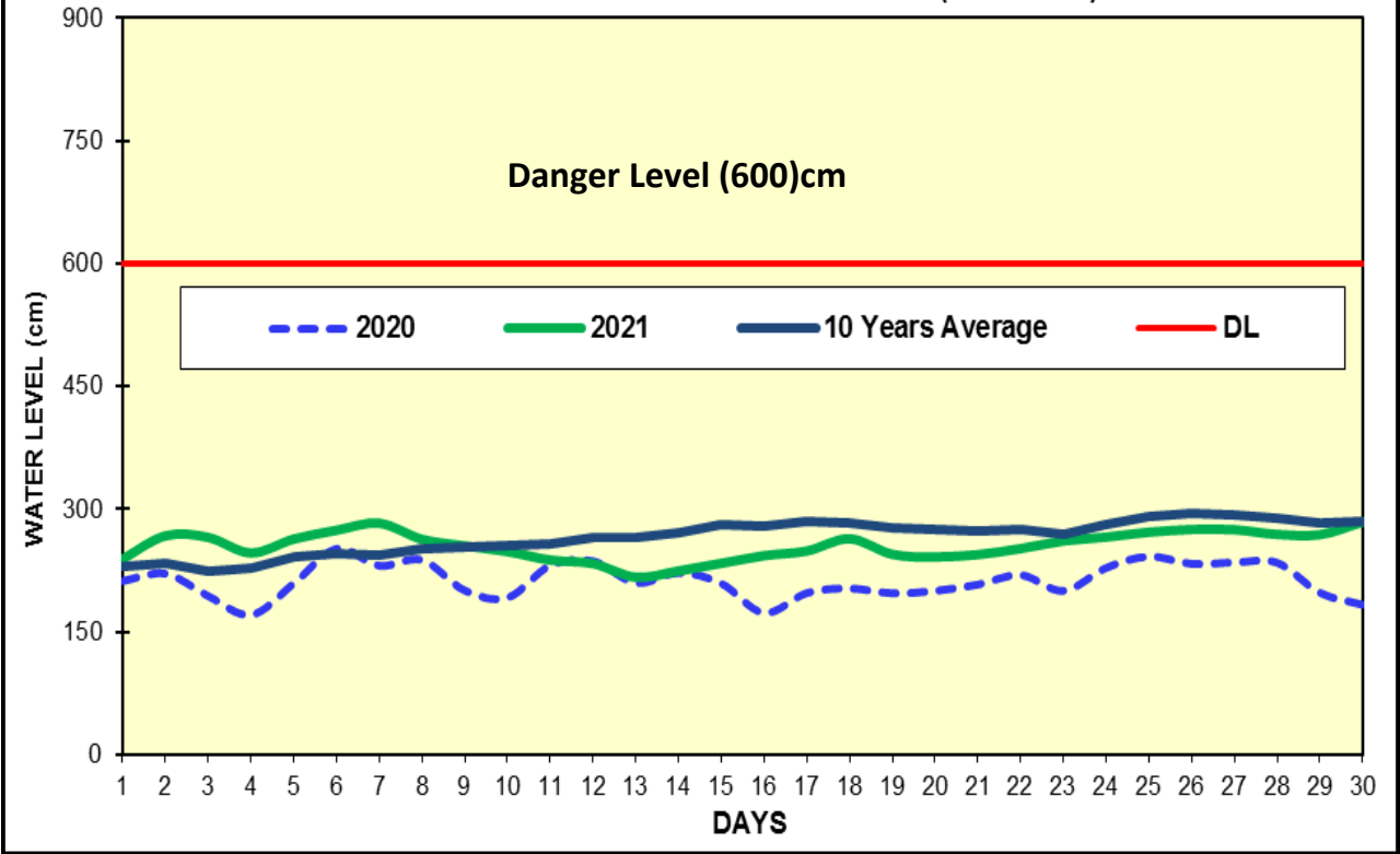
Fig(9) COMPARISON OF JUNE WATER LEVELS OF 2021 WITH JUNE WATER LEVELS OF 2020 AND 10 YEARS AVERAGE (TOUNGOO)
