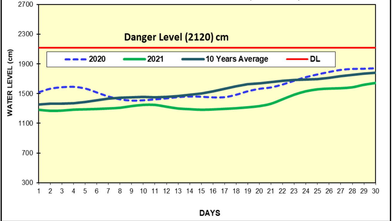
Fig(3) COMPARISON OF JUNE WATER LEVELS OF 2021 WITH JUNE WATER LEVELS OF 2020 AND 10 YEARS AVERAGE (NYAUNG OO)
