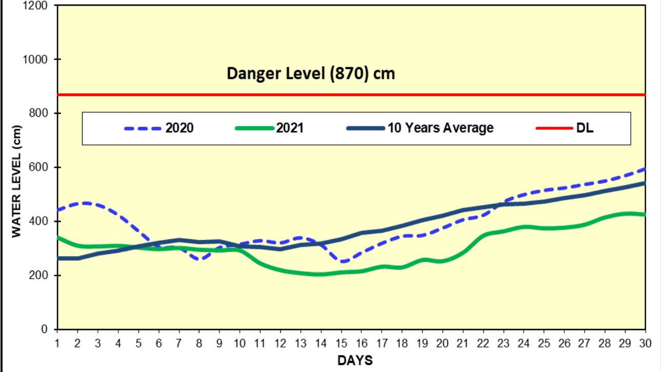
Fig(8) COMPARISON OF JUNE WATER LEVELS OF 2021 WITH JUNE WATER LEVELS OF 2020 AND 10 YEARS AVERAGE (MYITNGE)
