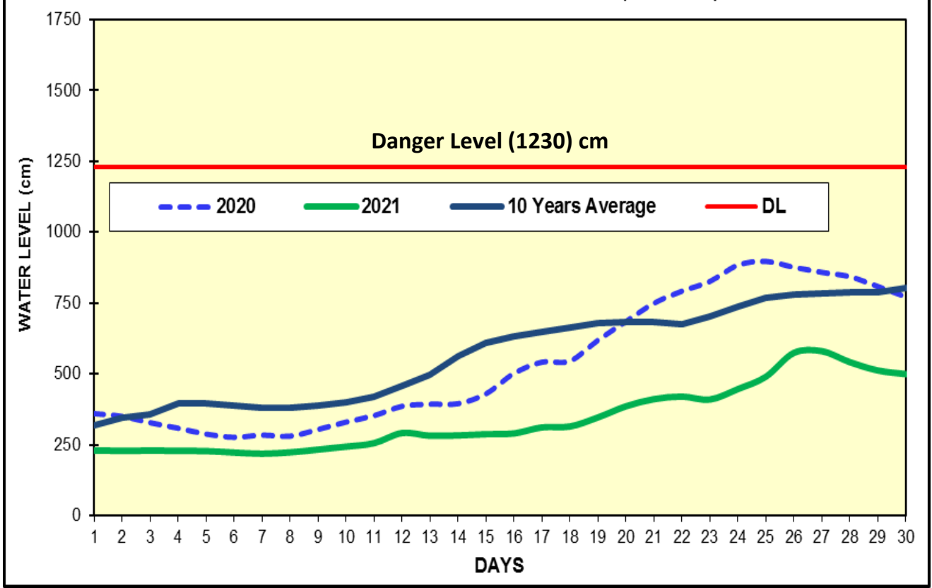
Fig(6) COMPARISON OF JUNE WATER LEVELS OF 2021 WITH JUNE WATER LEVELS OF 2020 AND 10 YEARS AVERAGE (MAWLAIK)
