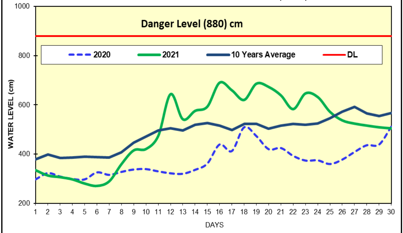
Fig(12) COMPARISON OF JUNE WATER LEVELS OF 2021 WITH JUNE WATER LEVELS OF 2020 AND 10 YEARS AVERAGE (BAGO)
