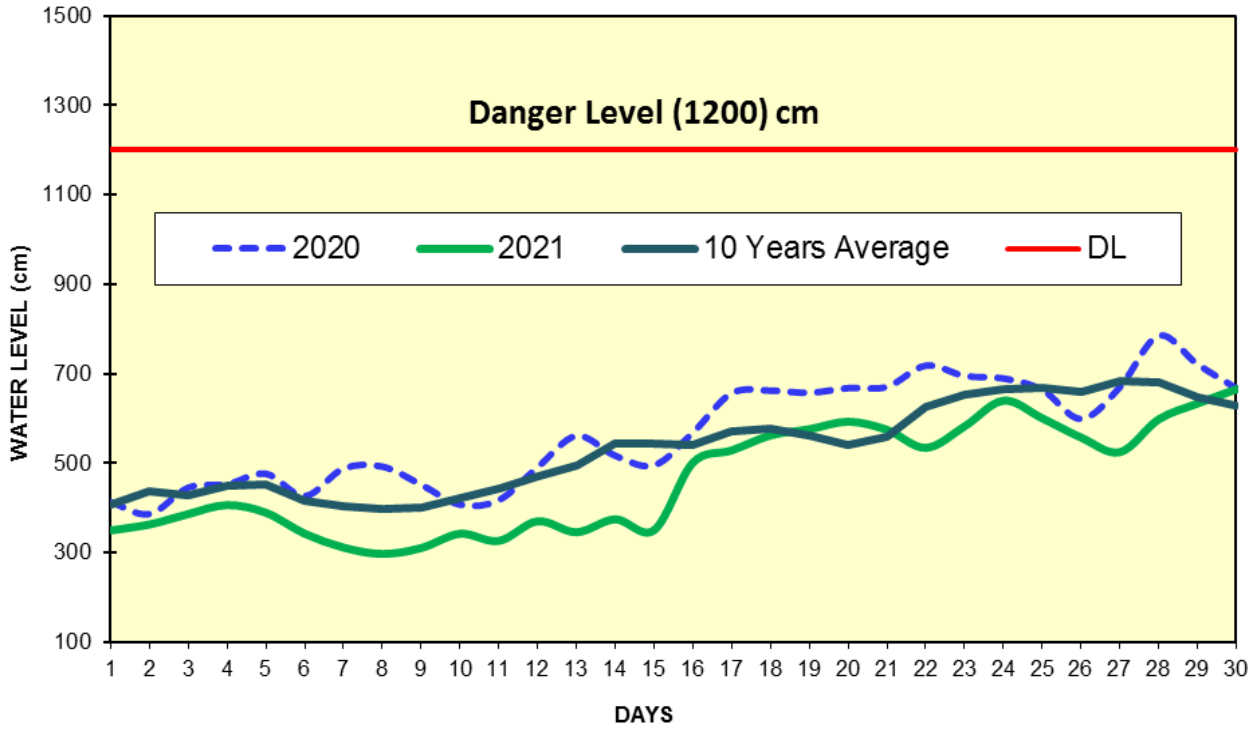
Fig(1) COMPARISON OF JUNE WATER LEVELS OF 2021 WITH JUNE WATER LEVELS OF 2020 AND 10 YEARS AVERAGE (MYITKYINA)
