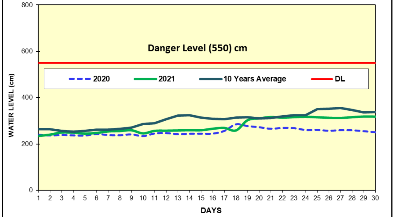
Fig(16) COMPARISON OF JUNE WATER LEVELS OF 2021 WITH JUNE WATER LEVELS OF 2020 AND 10 YEARS AVERAGE (KYAUK TAW)
