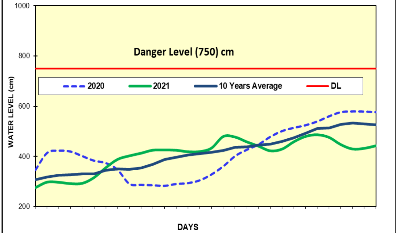
Fig(13) COMPARISON OF JUNE WATER LEVELS OF 2021 WITH JUNE WATER LEVELS OF 2020 AND 10 YEARS AVERAGE (HPA-AN)
