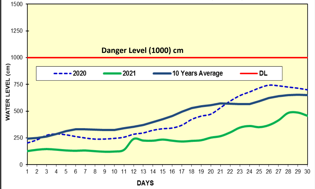
Fig(7) COMPARISON OF JUNE WATER LEVELS OF 2021 WITH JUNE WATER LEVELS OF 2020 AND 10 YEARS AVERAGE (MONYWA)
