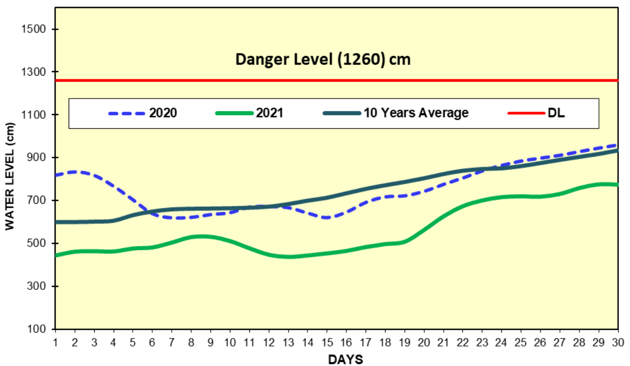
Fig(2) COMPARISON OF JUNE WATER LEVELS OF 2021 WITH JUNE WATER LEVELS OF 2020 AND 10 YEARS AVERAGE (MANDALAY)
