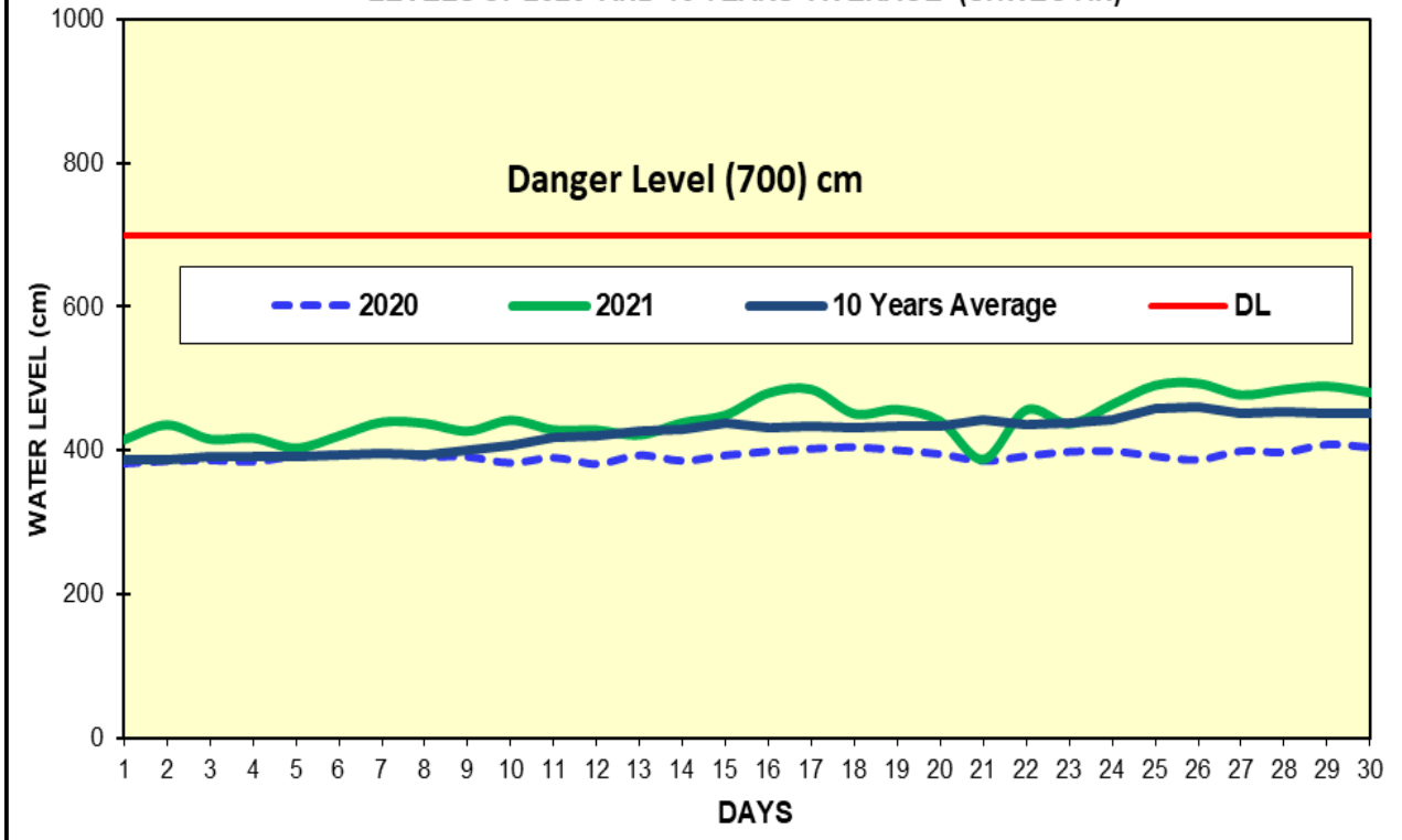
Fig(11) COMPARISON OF JUNE WATER LEVELS OF 2021 WITH JUNE WATER LEVELS OF 2020 AND 10 YEARS AVERAGE (SHWEGYIN)
