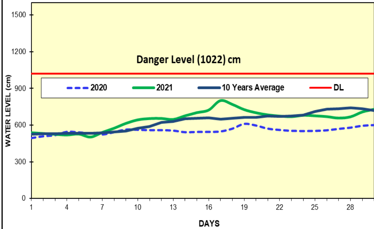
Fig(19) COMPARISON OF JUNE WATER LEVELS OF 2021 WITH JUNE WATER LEVELS OF 2020 AND 10 YEARS AVERAGE (BILIN)
