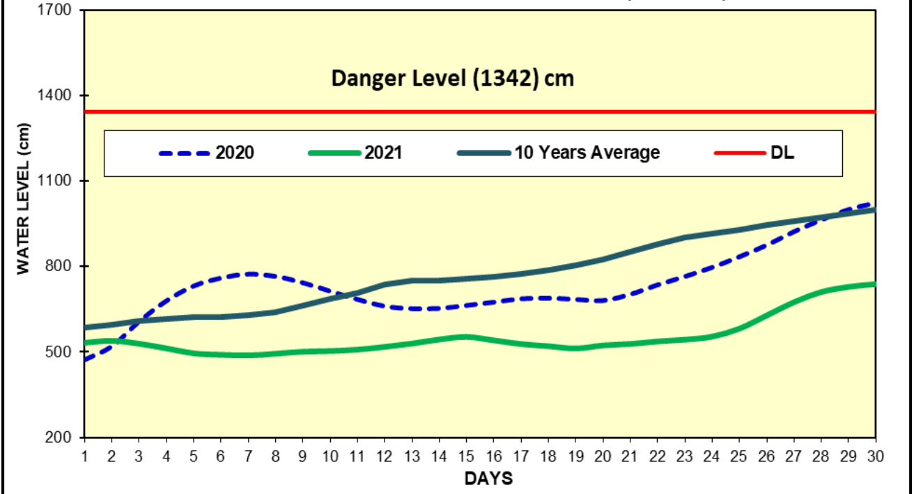
Fig(4) COMPARISON OF JUNE WATER LEVELS OF 2021 WITH JUNE WATER LEVELS OF 2020 AND 10 YEARS AVERAGE (HINTHADA)
