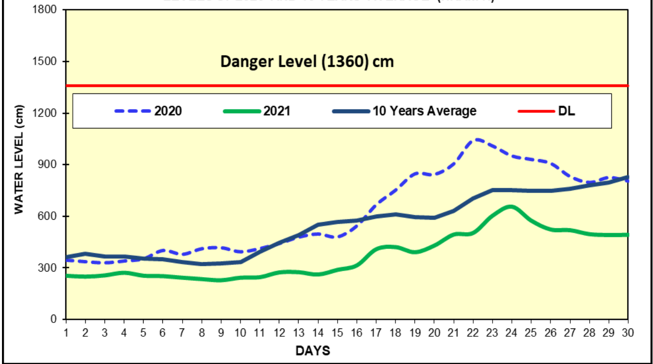
Fig(5) COMPARISON OF JUNE WATER LEVELS OF 2021 WITH JUNE WATER LEVELS OF 2020 AND 10 YEARS AVERAGE (HKAMTI)
