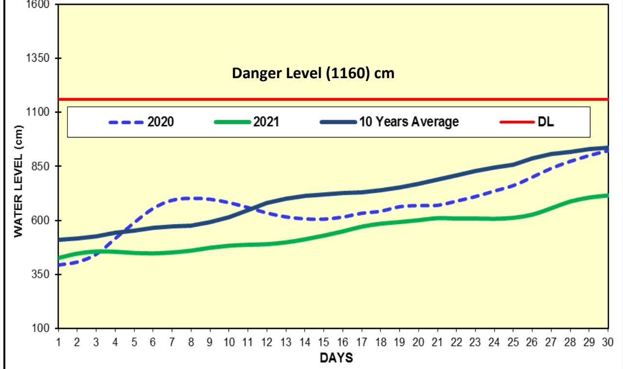
Fig(14) COMPARISON OF JUNE WATER LEVELS OF 2021 WITH JUNE LEVELS OF 2020 AND 10 YEARS AVERAGE (NGATHAINGCHAUNG)
