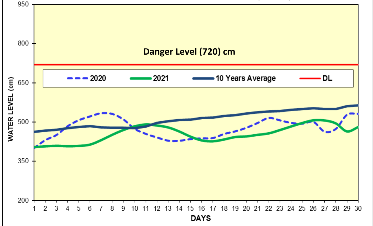
Fig(15) COMPARISON OF JUNE WATER LEVELS OF 2021 WITH JUNE WATER LEVELS OF 2020 AND 10 YEARS AVERAGE (MAUBIN)
