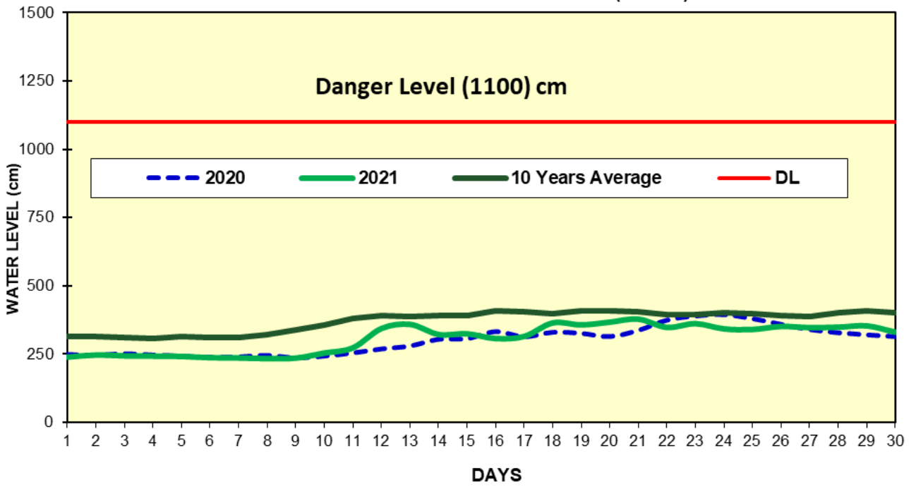
Fig(18) COMPARISON OF JUNE WATER LEVELS OF 2021 WITH JUNE WATER LEVELS OF 2020 AND 10 YEARS AVERAGE (KALAY)
