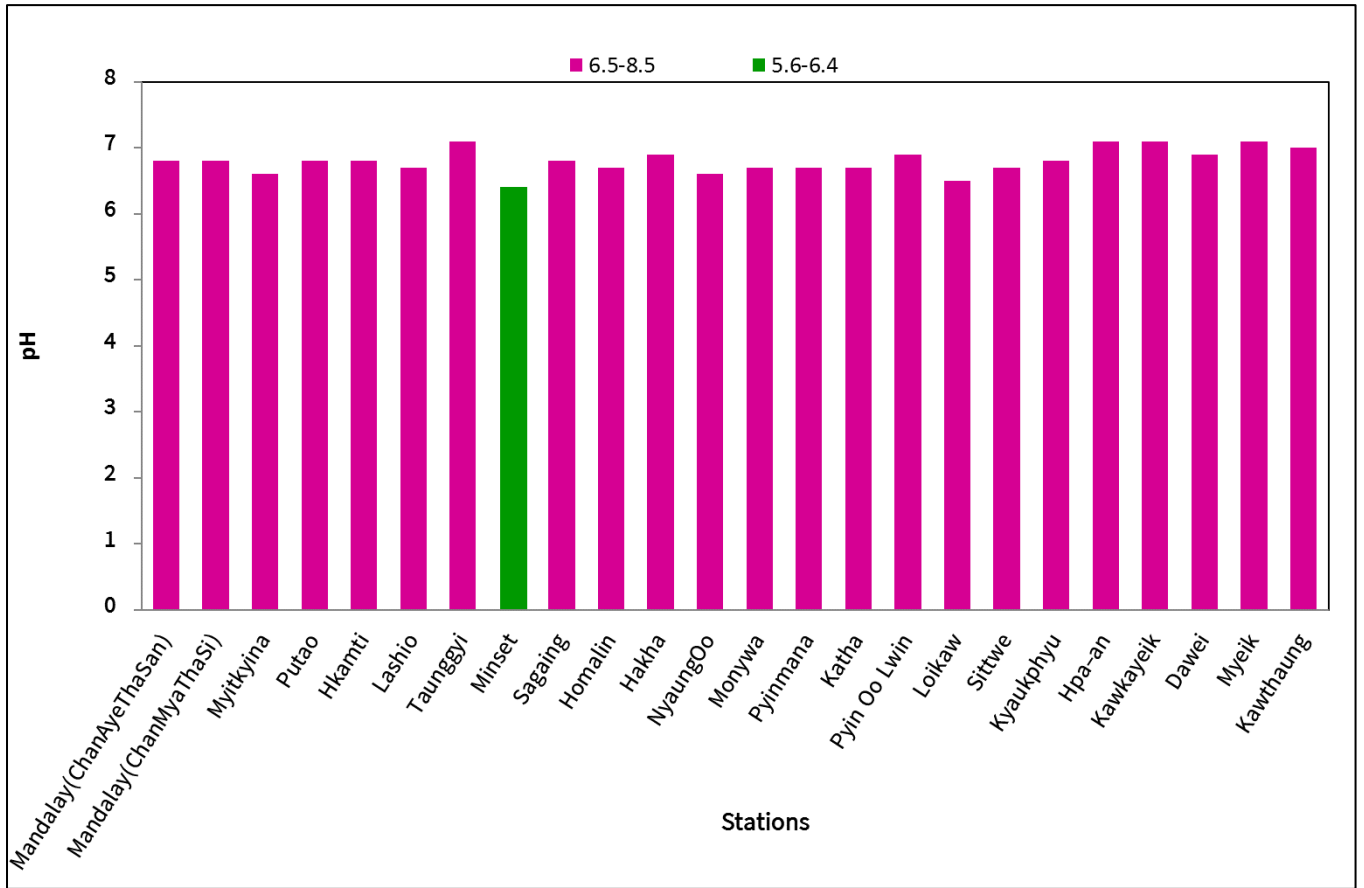
pH Value's Graph of Rain Water Sample on April 2023
