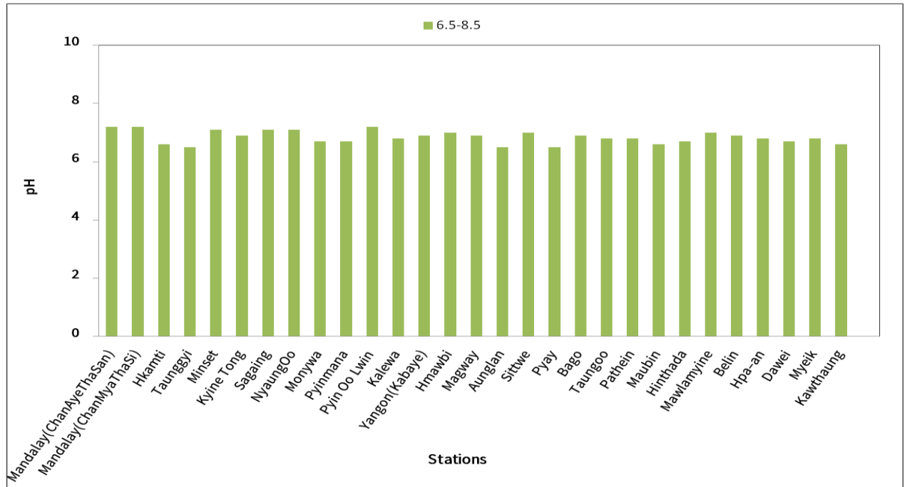
pH Value's Graph of Rain Water Sample on May 2025
