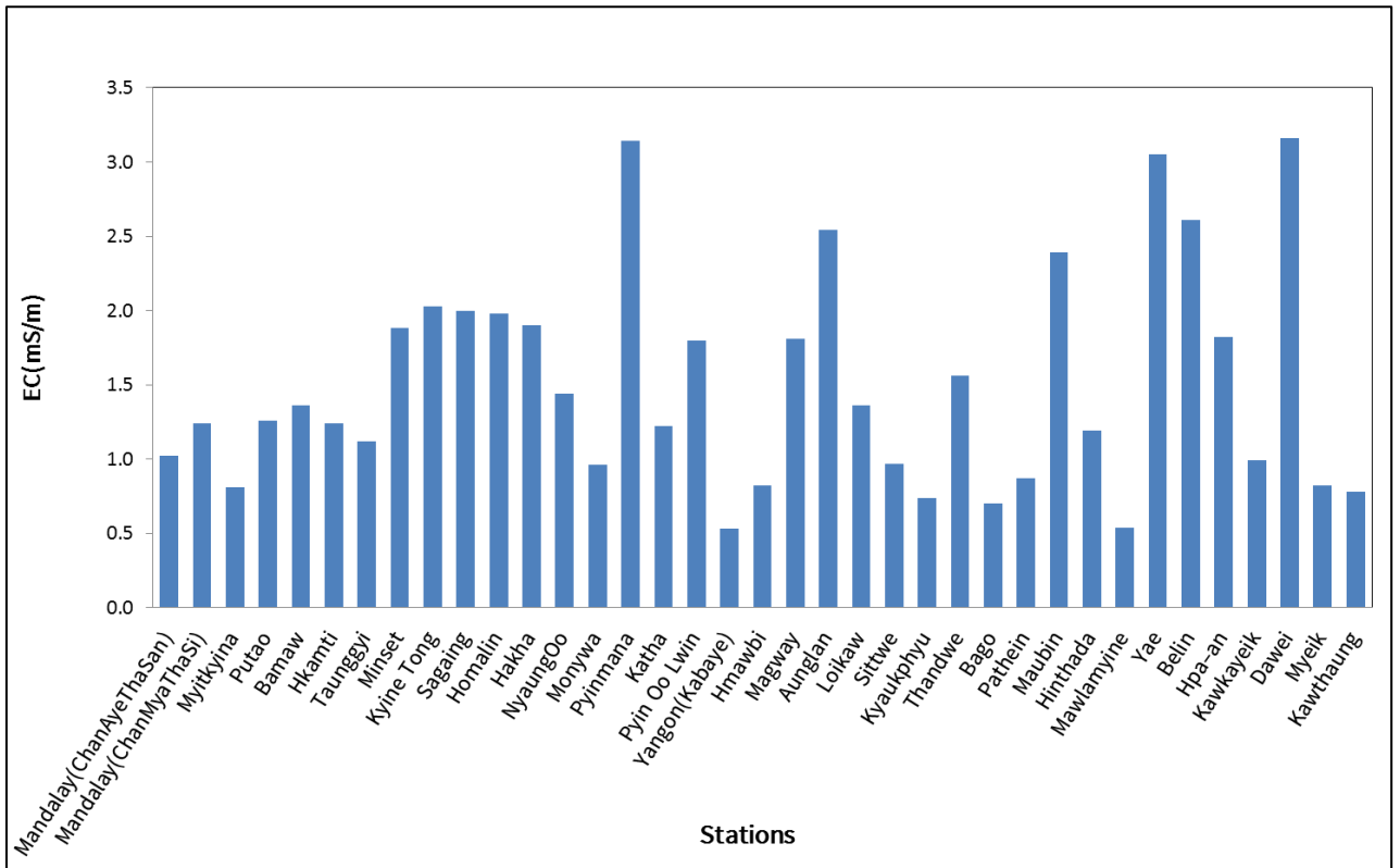
EC (mS/m) Value's Graph of Rain Water Sample on November 2023
