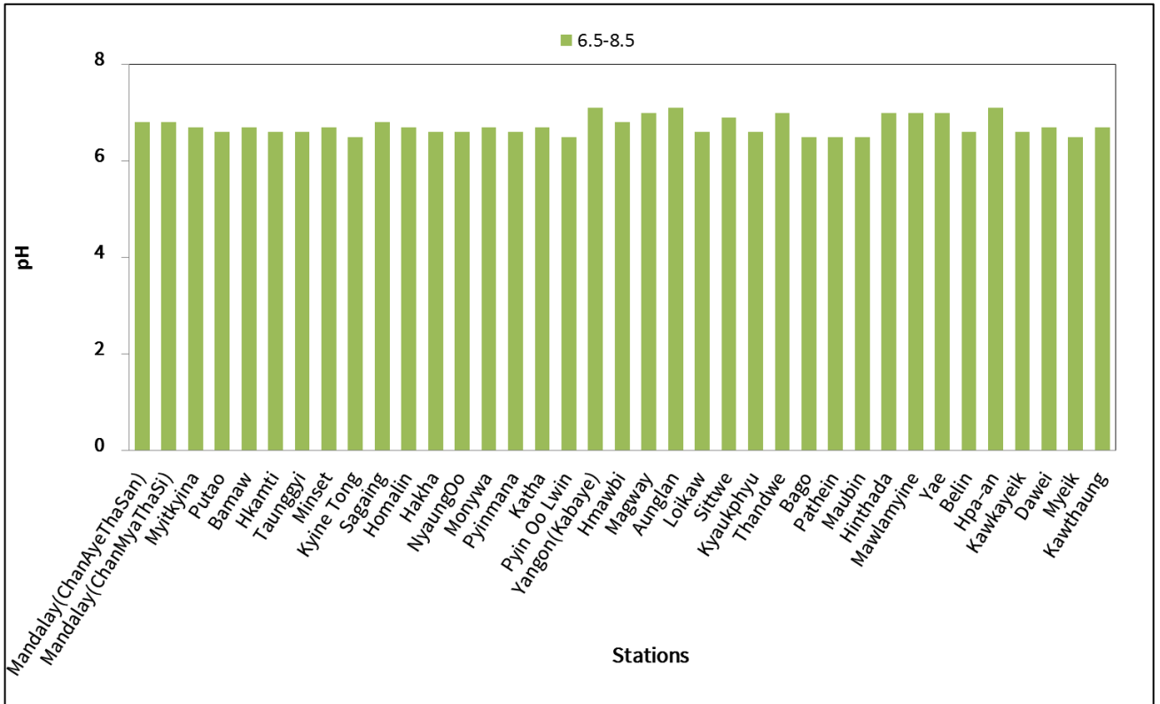
pH Value's Graph of Rain Water Sample on November 2023
