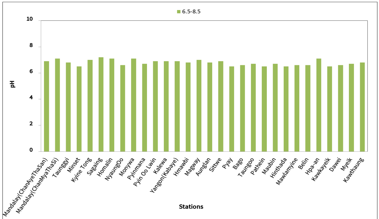
pH Value's Graph of Rain Water Sample on April 2025
