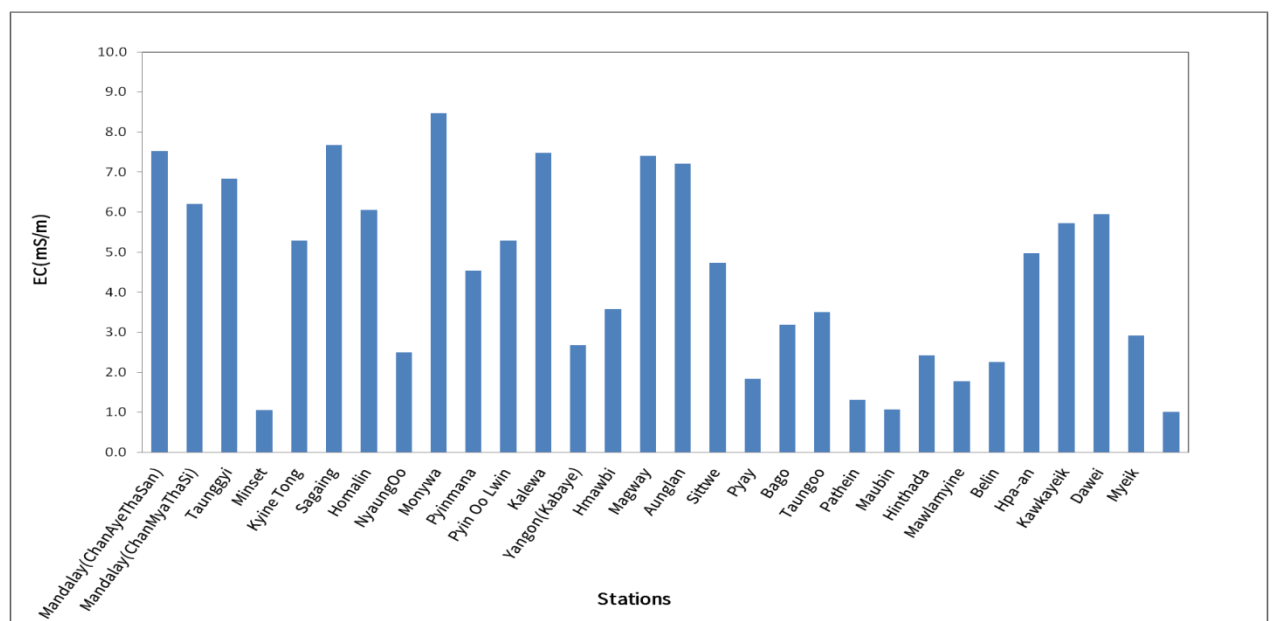
EC (mS/m) Value's Graph of Rain Water Sample on April 2025
