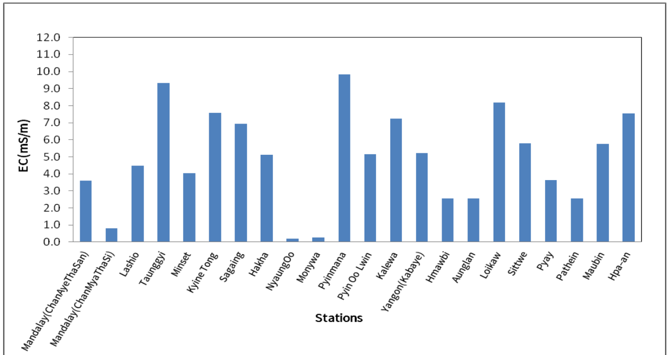
EC (mS/m) Value's Graph of Rain Water Sample on March 2026
