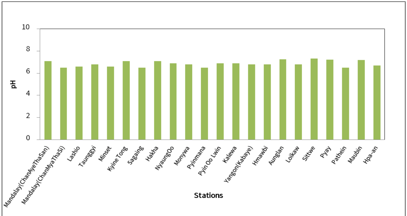
pH Value's Graph of Rain Water Sample on March 2026
