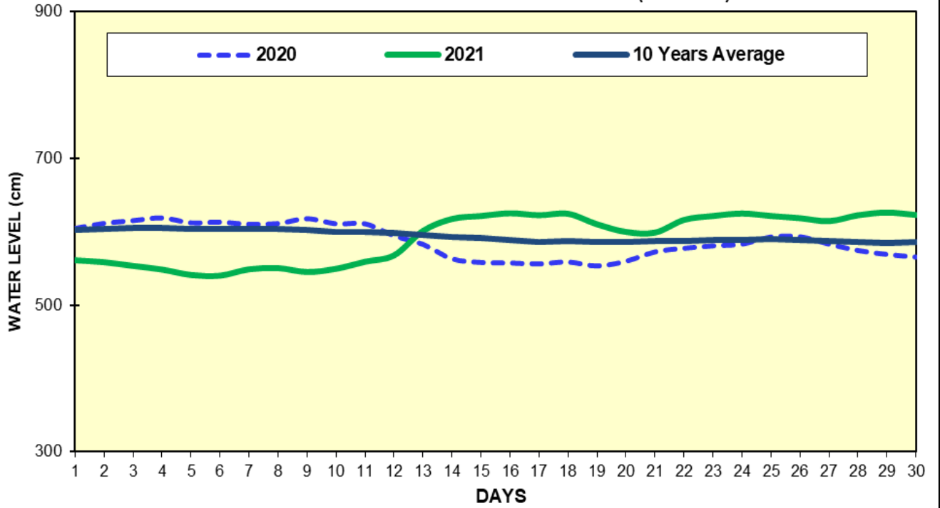
Fig(10) COMPARISON APRIL WATER LEVELS OF 2021 WITH APRIL WATER LEVELS OF 2020 AND 10 YEARS AVERAGE (MADAUK)
