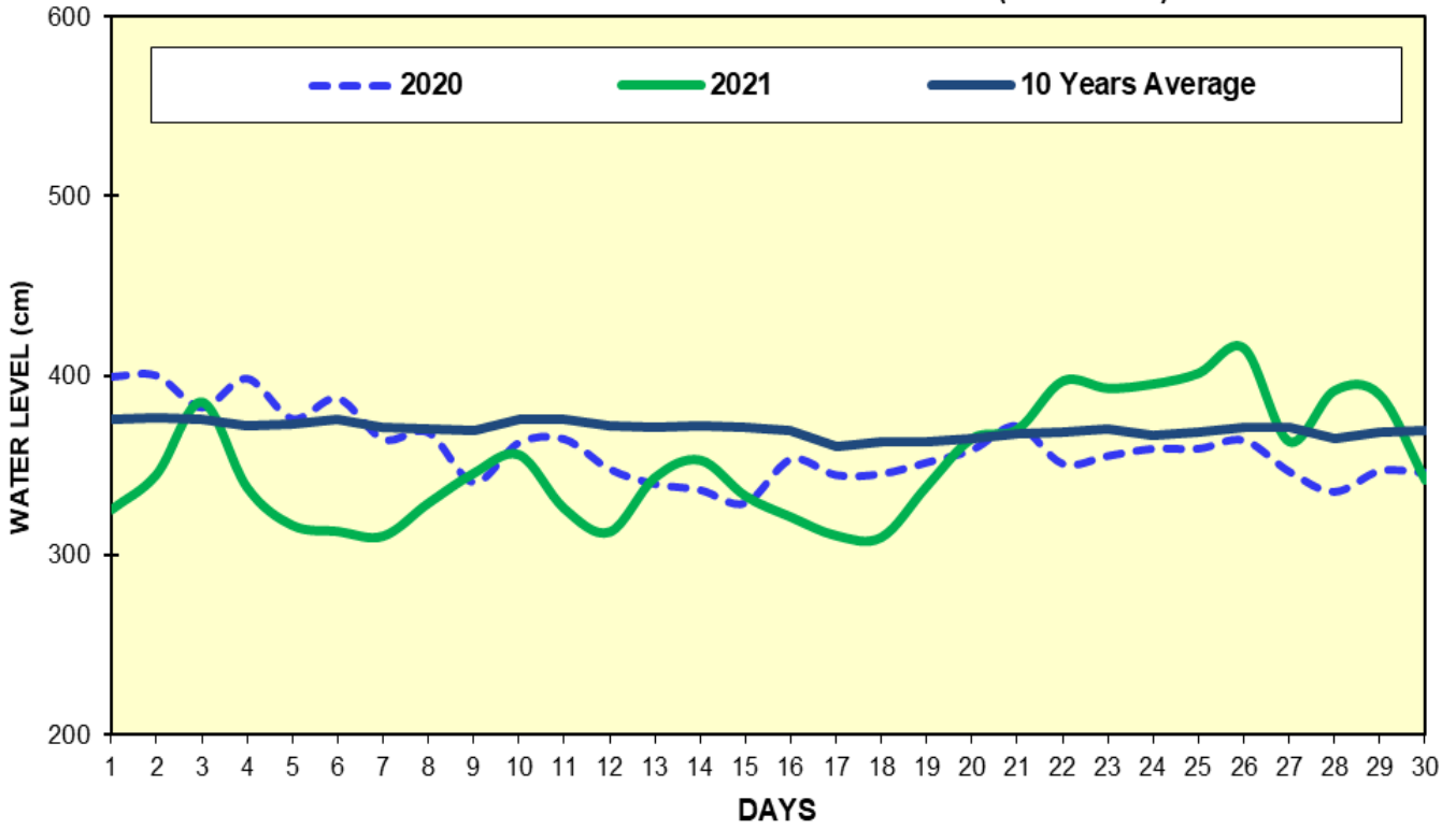
Fig(11) COMPARISON OF APRIL WATER LEVELS OF 2021 WITH APRIL WATER LEVELS OF 2020 AND 10 YEARS AVERAGE (SHWEGYIN)
