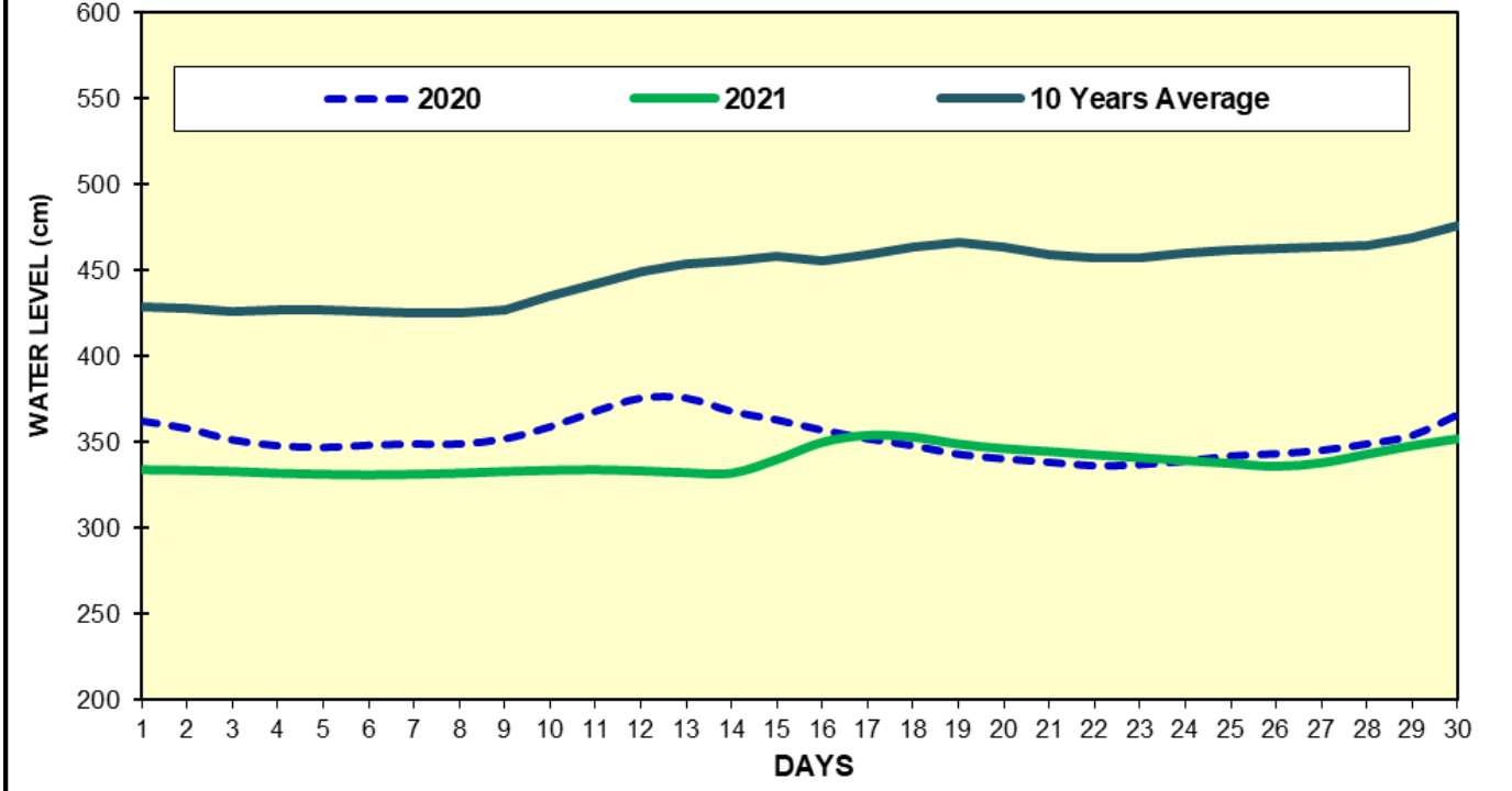
Fig(4) COMPARISON OF APRIL WATER LEVELS OF 2021 WITH APRIL WATER LEVELS OF 2020 AND 10 YEARS AVERAGE (HINTHADA)
