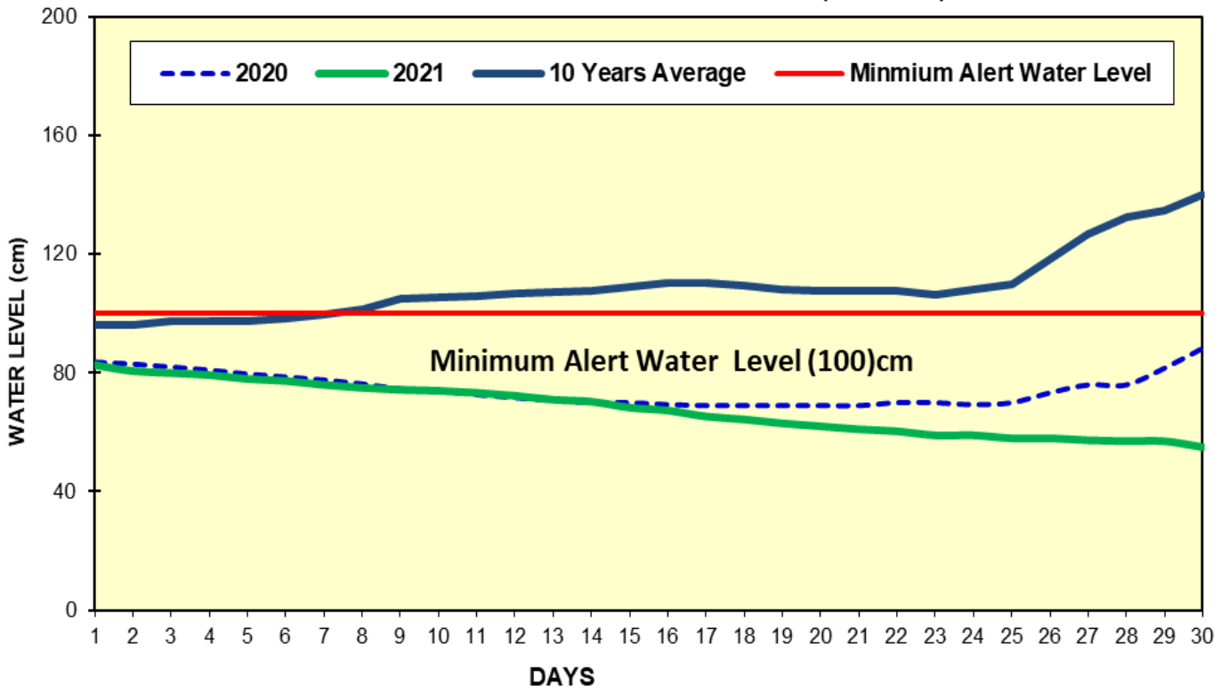
Fig(7) COMPARISON OF APRIL WATER LEVELS OF 2021 WITH APRIL WATER LEVELS OF 2020 AND 10 YEARS AVERAGE (MONYWA)
