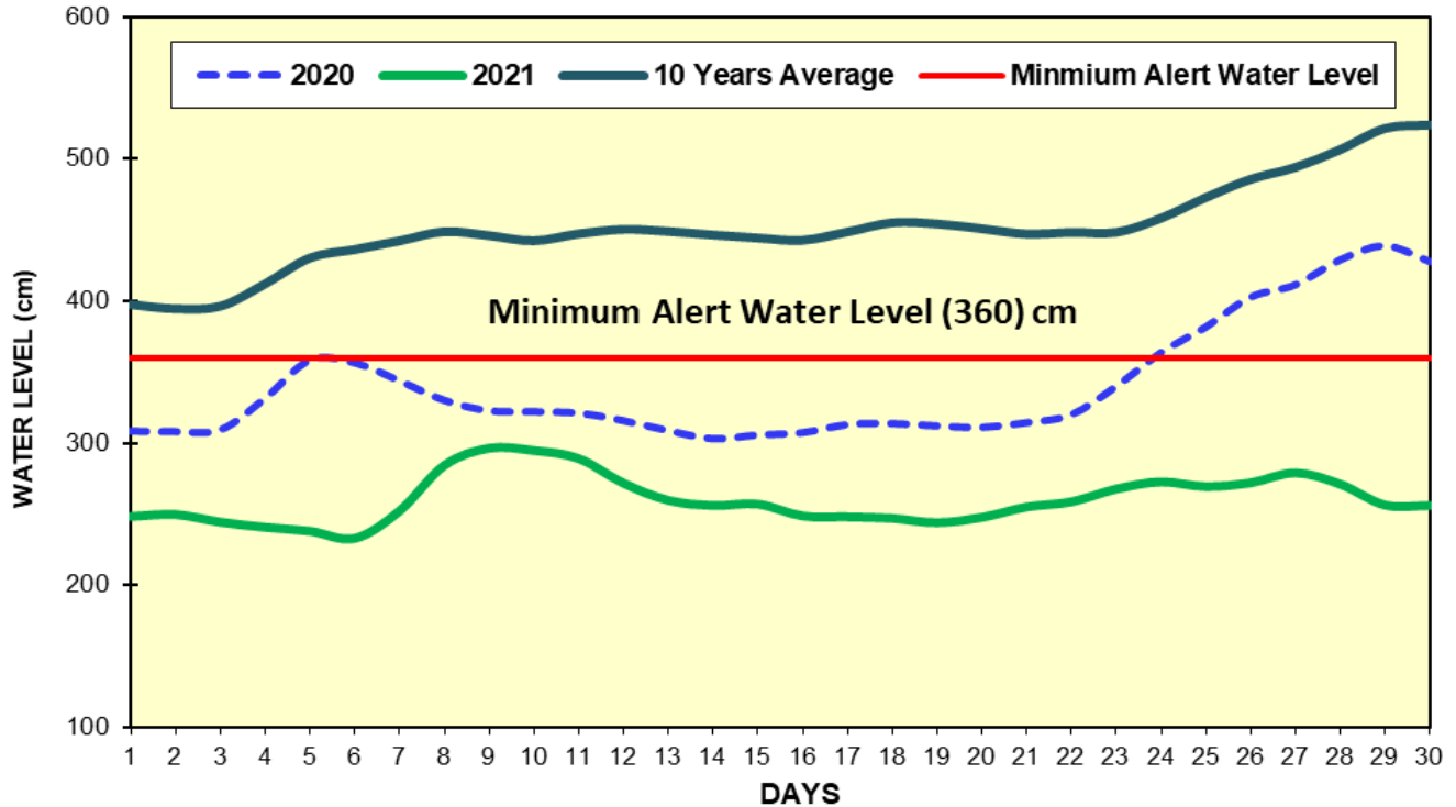
Fig(2) COMPARISON OF APRIL WATER LEVELS OF 2021 WITH APRIL WATER LEVELS OF 2020 AND 10 YEARS AVERAGE (MANDALAY)
