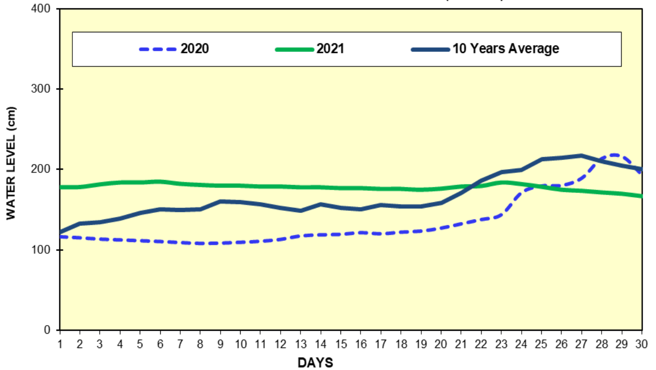
Fig(5) COMPARISON OF APRIL WATER LEVELS OF 2021 WITH APRIL WATER LEVELS OF 2020 AND 10 YEARS AVERAGE (HKAMTI)
