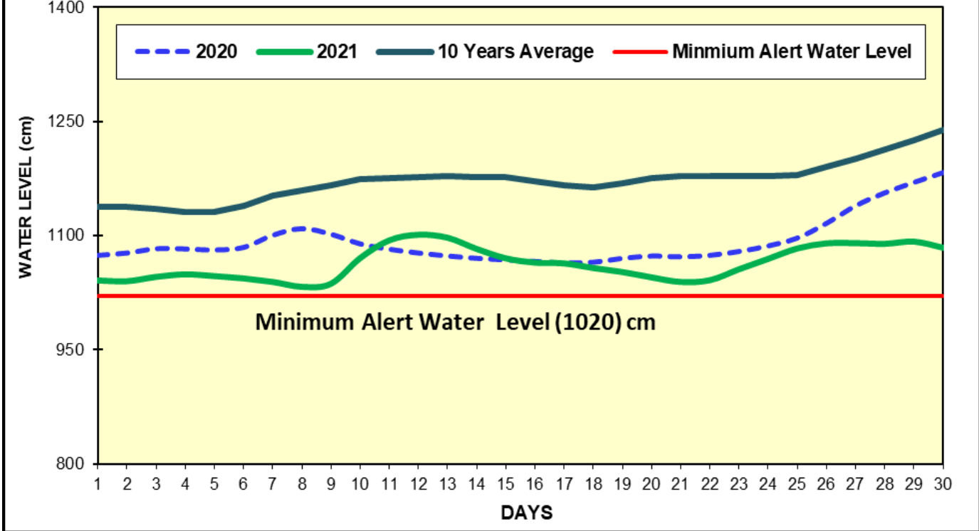
Fig(3) COMPARISON OF APRIL WATER LEVELS OF 2021 WITH APRIL WATER LEVELS OF 2020 AND 10 YEARS AVERAGE (NYAUNG OO)
