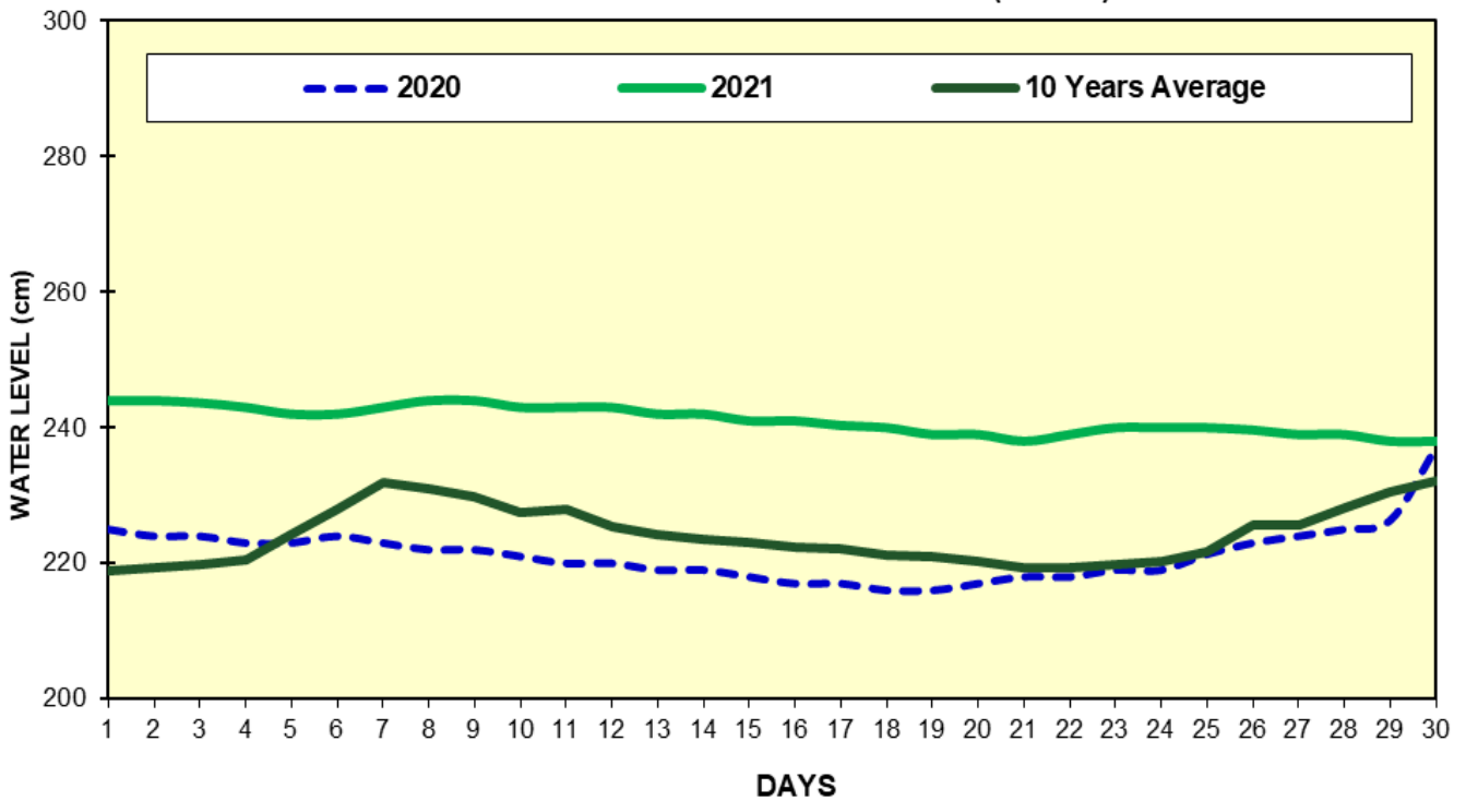
Fig(18) COMPARISON OF APRIL WATER LEVELS OF 2021 WITH APRIL WATER LEVELS OF 2020 AND 10 YEARS AVERAGE (KALAY)
