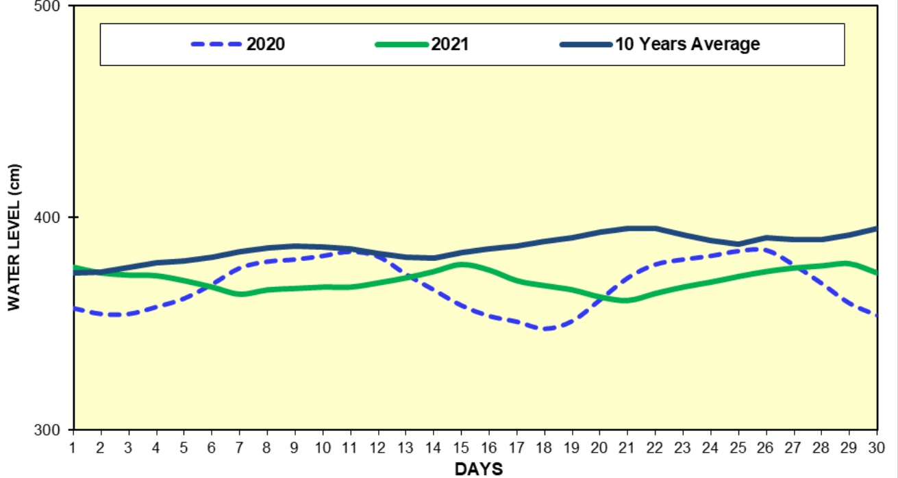
Fig(14) COMPARISON OF APRIL WATER LEVELS OF 2021 WITH APRIL LEVELS OF 2020 AND 10 YEARS AVERAGE (NGATHAINGCHAUNG)
