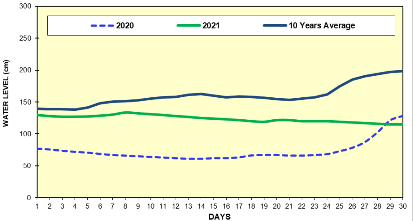
Fig(6) COMPARISON OF APRIL WATER LEVELS OF 2021 WITH APRIL WATER LEVELS OF 2020 AND 10 YEARS AVERAGE (MAWLAIK)
