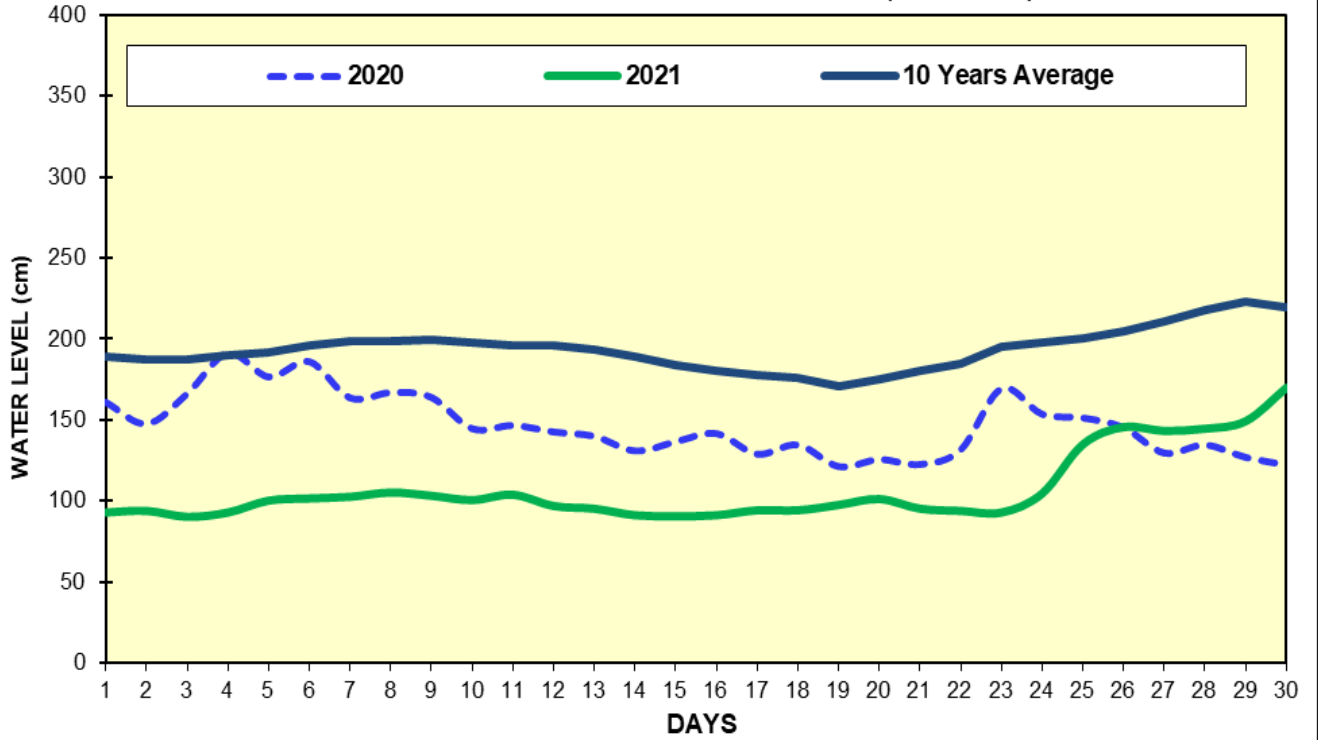
Fig(9) COMPARISON OF APRIL WATER LEVELS OF 2021 WITH APRIL WATER LEVELS OF 2020 AND 10 YEARS AVERAGE (TOUNGOO)
