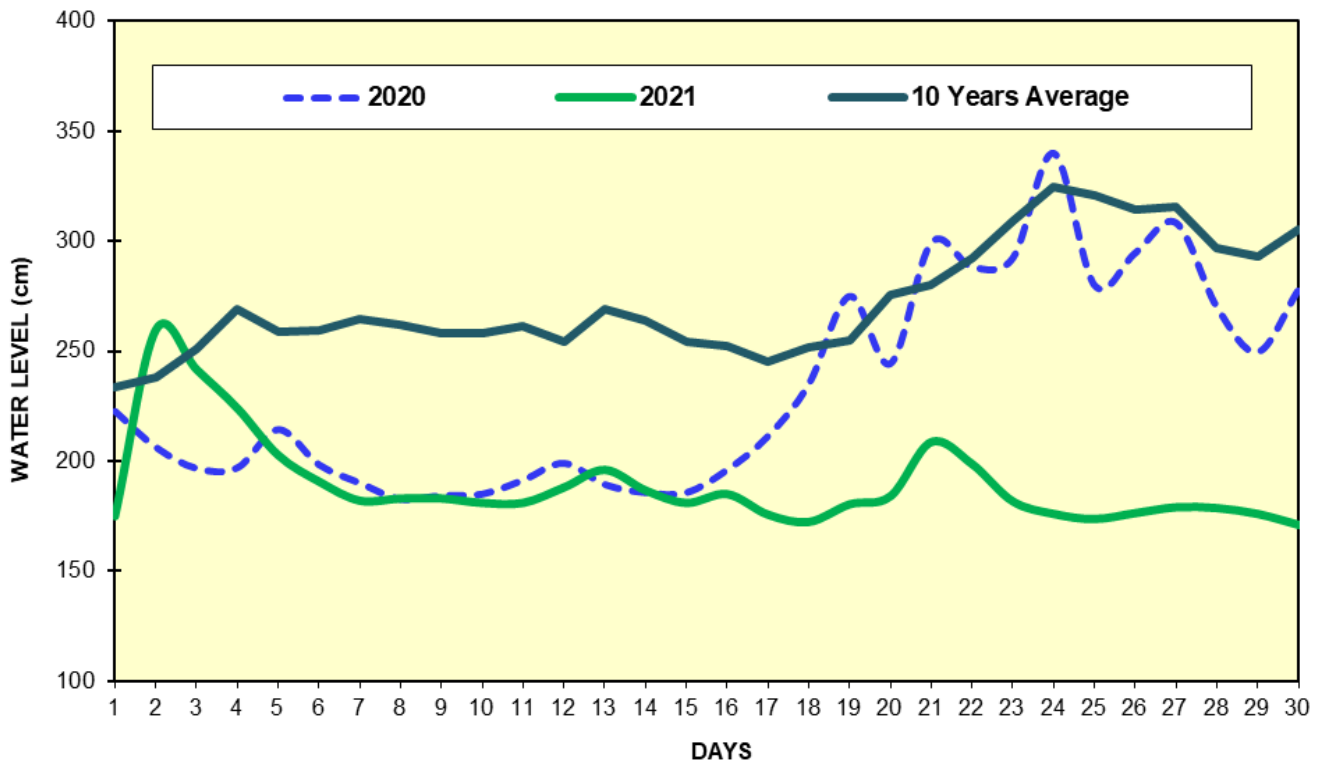
Fig(1) COMPARISON OF APRIL WATER LEVELS OF 2021 WITH APRIL WATER LEVELS OF 2020 AND 10 YEARS AVERAGE (MYITKYINA)
