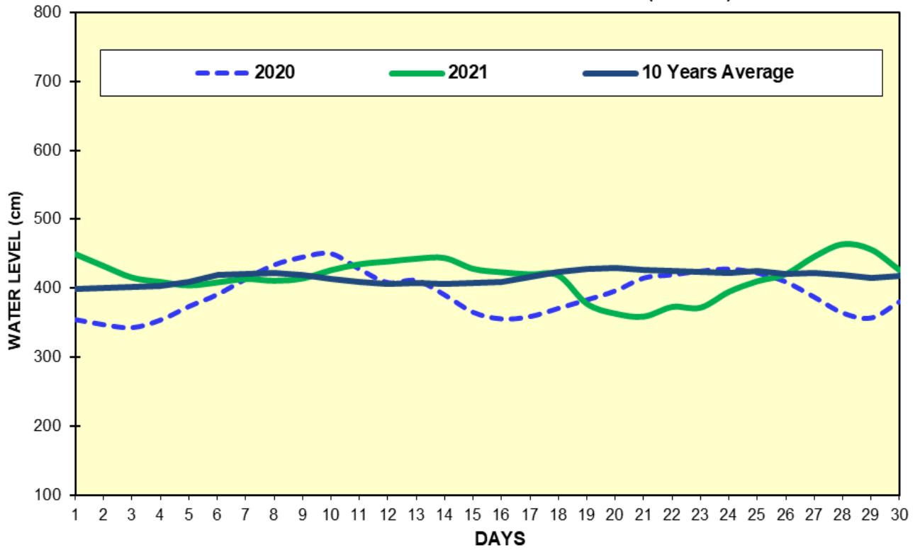
Fig(15) COMPARISON OF APRIL WATER LEVELS OF 2021 WITH APRIL WATER LEVELS OF 2020 AND 10 YEARS AVERAGE (MAUBIN)
