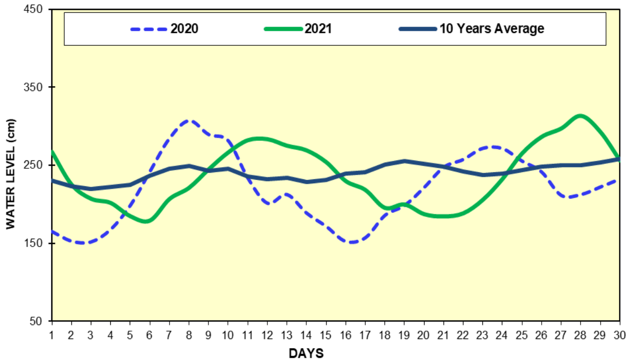
Fig(13) COMPARISON OF APRIL WATER LEVELS OF 2021 WITH APRIL WATER LEVELS OF 2020 AND 10 YEARS AVERAGE (HPA-AN)
