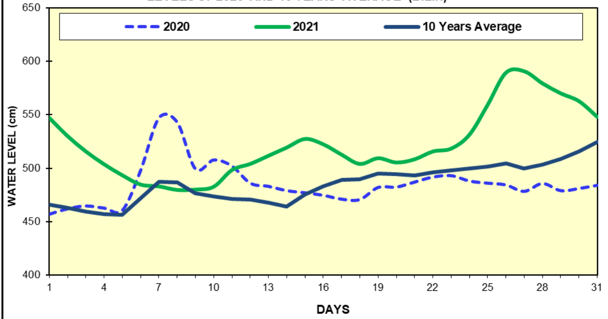
Fig(19) COMPARISON OF MAY WATER LEVELS OF 2021 WITH MAY WATER LEVELS OF 2020 AND 10 YEARS AVERAGE (BILIN)
