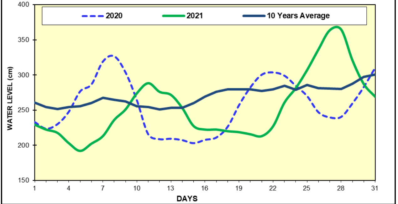
Fig(13) COMPARISON OF MAY WATER LEVELS OF 2021 WITH MAY WATER LEVELS OF 2020 AND 10 YEARS AVERAGE (HPA-AN)
