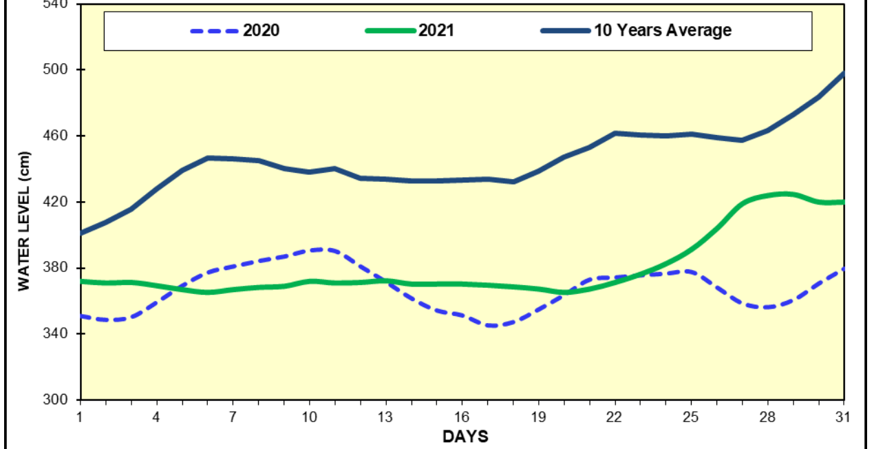
Fig(14) COMPARISON OF MAY WATER LEVELS OF 2021 WITH MAY LEVELS OF 2020 AND 10 YEARS AVERAGE (NGATHAINGCHAUNG)
