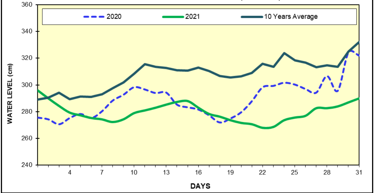
Fig(17) COMPARISON MAY WATER LEVELS OF 2021 WITH MAY WATER LEVELS OF 2020 AND 10 YEARS AVERAGE (PALETWA)
