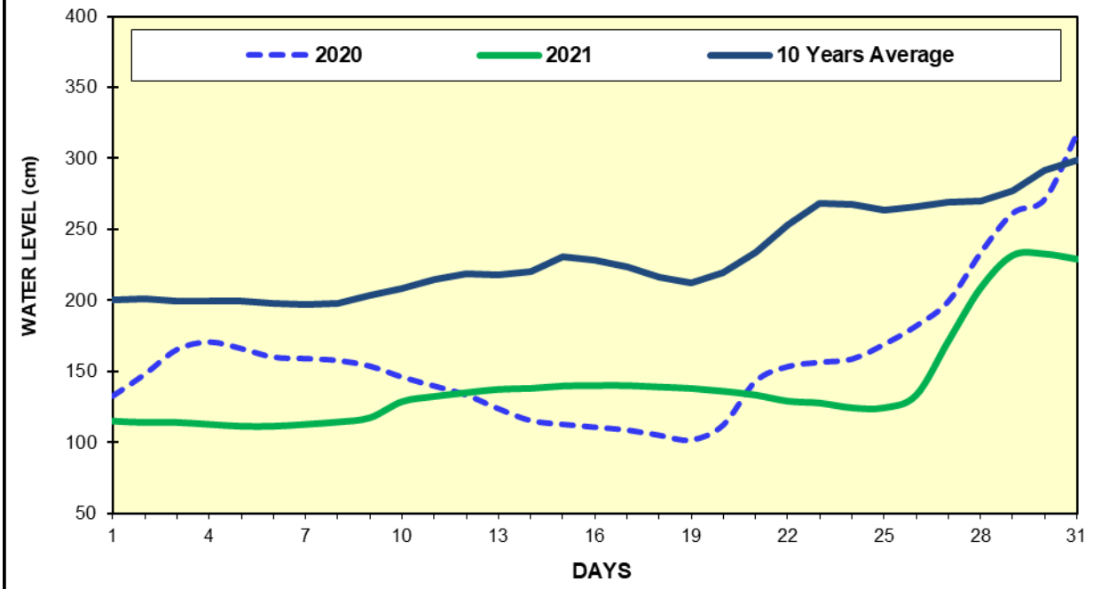
Fig(6) COMPARISON OF MAY WATER LEVELS OF 2021 WITH MAY WATER LEVELS OF 2020 AND 10 YEARS AVERAGE (MAWLAIK)
