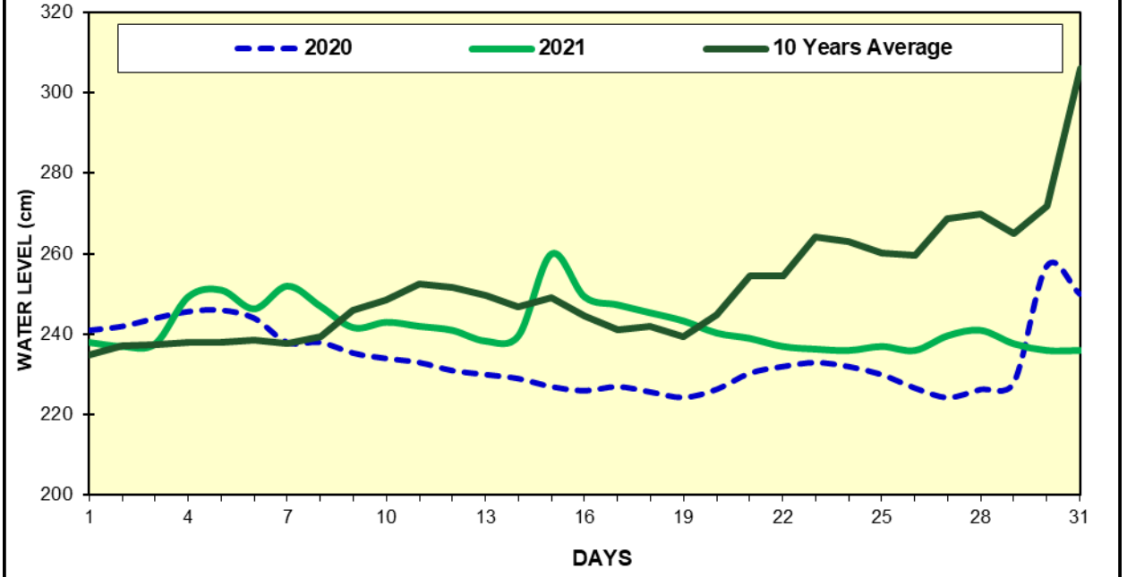
Fig(18) COMPARISON OF MAY WATER LEVELS OF 2021 WITH MAY WATER LEVELS OF 2020 AND 10 YEARS AVERAGE (KALAY)
