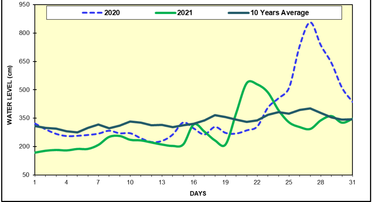
Fig(1) COMPARISON OF MAY WATER LEVELS OF 2021 WITH MAY WATER LEVELS OF 2020 AND 10 YEARS AVERAGE (MYITKYINA)
