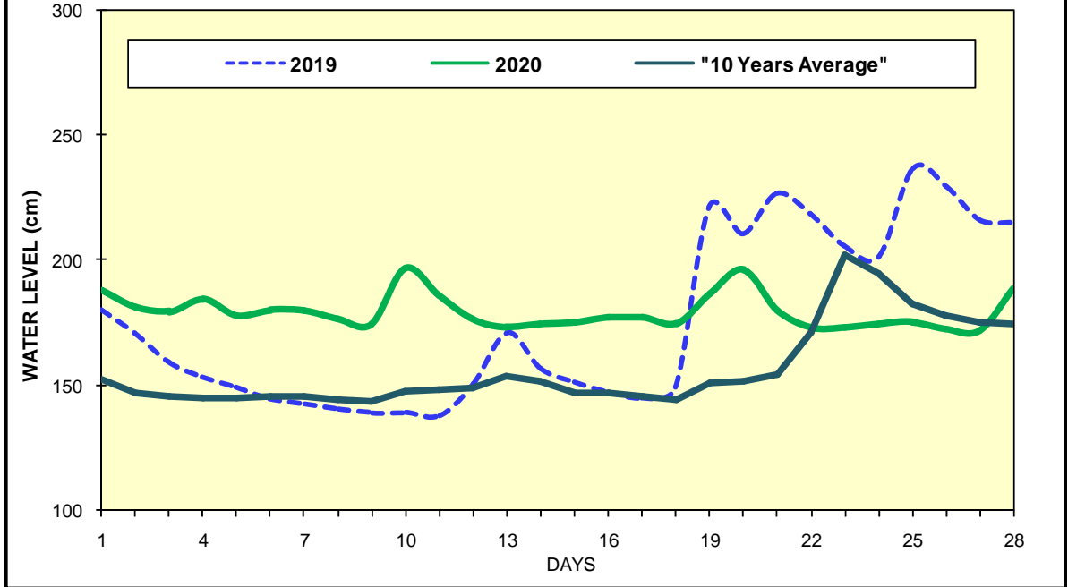
Fig(1) COMPARISON OF FEBRUARY WATER LEVELS OF 2020 WITH FEBRUARY WATER LEVELS OF 2019 AND 10 YEARS AVERAGE (MYITKYINA)
