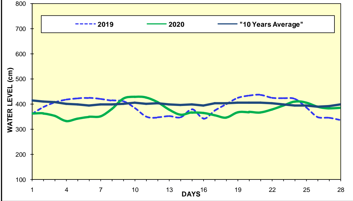
Fig(15) COMPARISON OF FEBRUARY WATER LEVELS OF 2020 WITH FEBRUARY WATER LEVELS OF 2019 AND 10 YEARS AVERAGE (MAUBIN)
