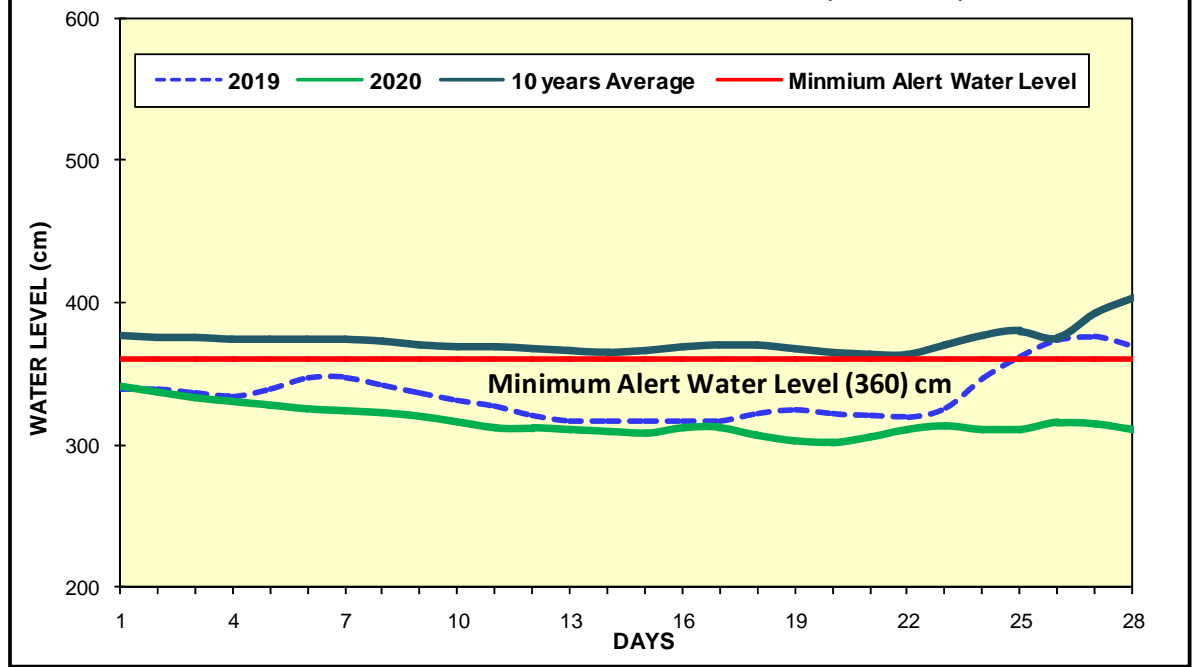
Fig(2) COMPARISON OF FEBRUARY WATER LEVELS OF 2020 WITH FEBRUARY WATER LEVELS OF 2019 AND 10 YEARS AVERAGE (MANDALAY)
