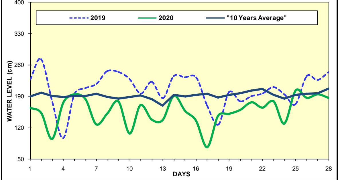
Fig(8) COMPARISON OF FEBRUARY WATER LEVELS OF 2020 WITH FEBRUARY WATER LEVELS OF 2019 AND 10 YEARS AVERAGE (MYITNGE)
