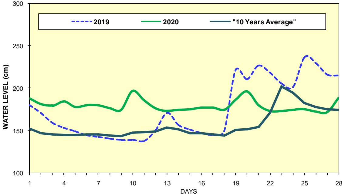
Fig(1) COMPARISON OF FEBRUARY WATER LEVELS OF 2020 WITH FEBRUARY WATER LEVELS OF 2019 AND 10 YEARS AVERAGE (MYITKYINA)
