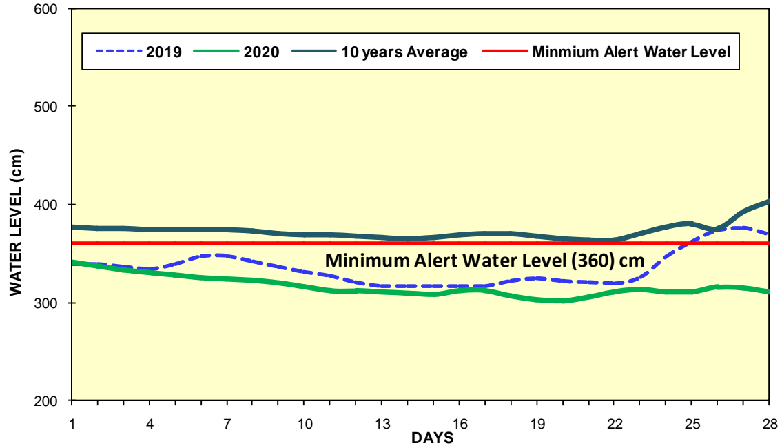
Fig(2) COMPARISON OF FEBRUARY WATER LEVELS OF 2020 WITH FEBRUARY WATER LEVELS OF 2019 AND 10 YEARS AVERAGE (MANDALAY)
