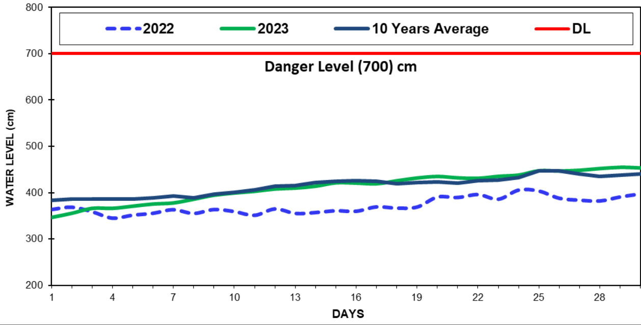
Fig(11) COMPARISON OF JUNE WATER LEVELS OF 2023 WITH JUNE WATER LEVELS OF 2022 AND 10 YEARS AVERAGE (SHWEGYIN)
