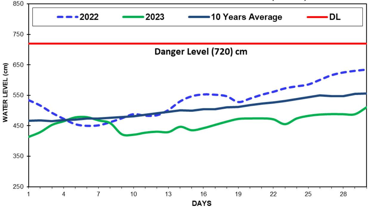
Fig(15) COMPARISON OF JUNE WATER LEVELS OF 2023 WITH JUNE WATER LEVELS OF 2022 AND 10 YEARS AVERAGE (MAUBIN)
