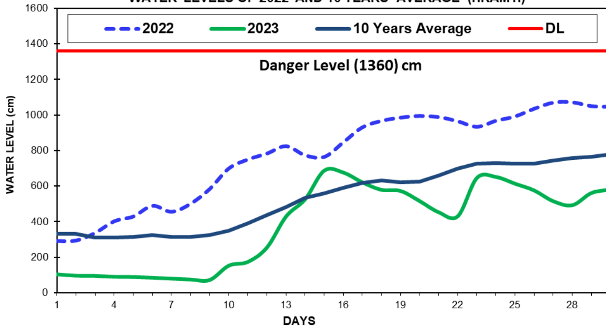
Fig(5) COMPARISON OF JUNE WATER LEVELS OF 2023 WITH JUNE WATER LEVELS OF 2022 AND 10 YEARS AVERAGE (HKAMTI)
