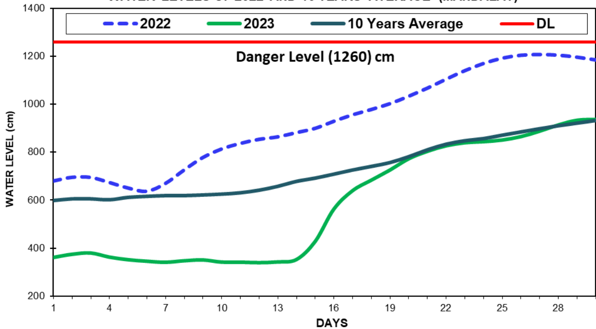
Fig(2) COMPARISON OF JUNE WATER LEVELS OF 2023 WITH JUNE WATER LEVELS OF 2022 AND 10 YEARS AVERAGE (MANDALAY)
