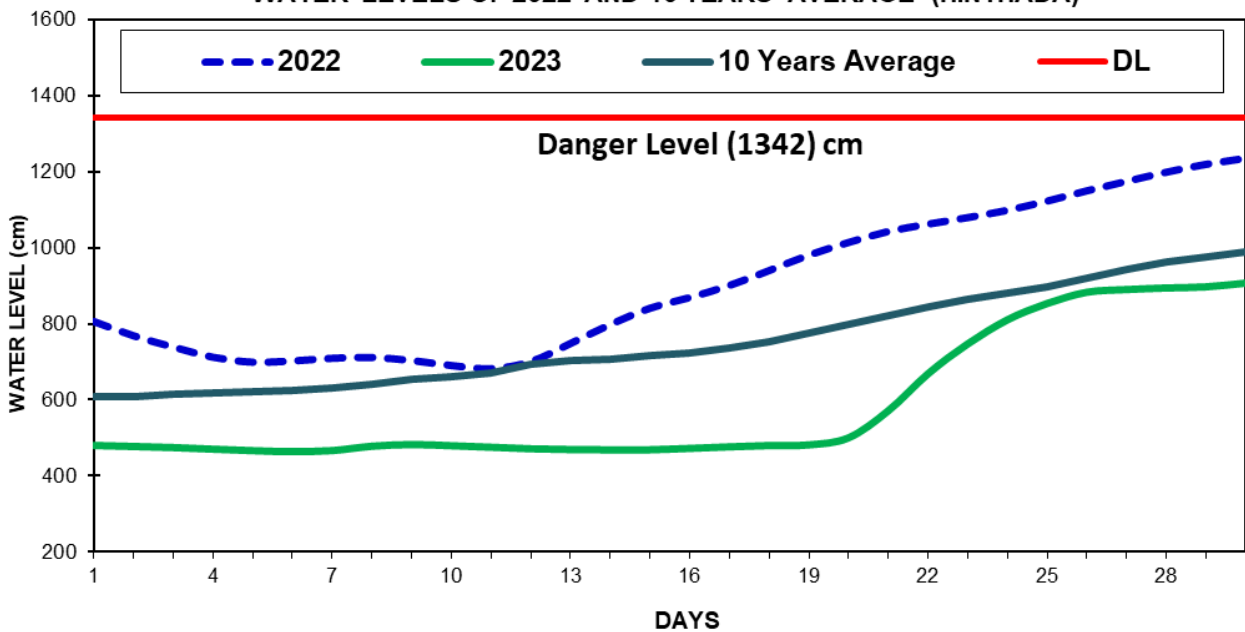
Fig(4) COMPARISON OF JUNE WATER LEVELS OF 2023 WITH JUNE WATER LEVELS OF 2022 AND 10 YEARS AVERAGE (HINTHADA)
