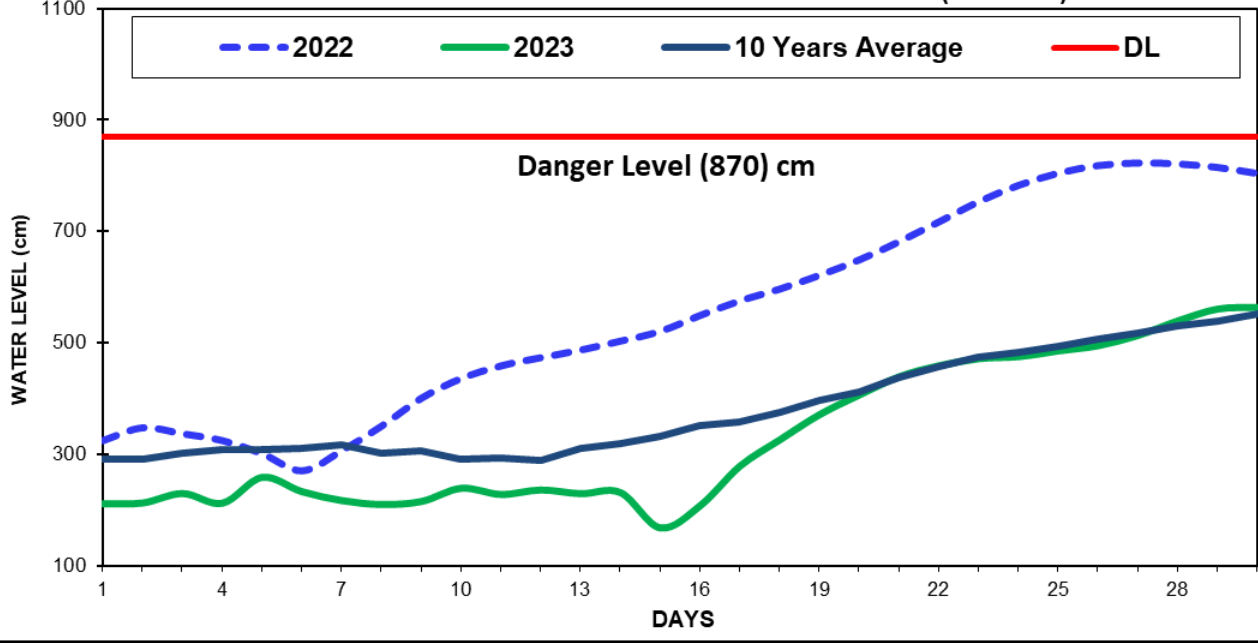
Fig(8) COMPARISON OF JUNE WATER LEVELS OF 2023 WITH JUNE WATER LEVELS OF 2022 AND 10 YEARS AVERAGE (MYITNGE)
