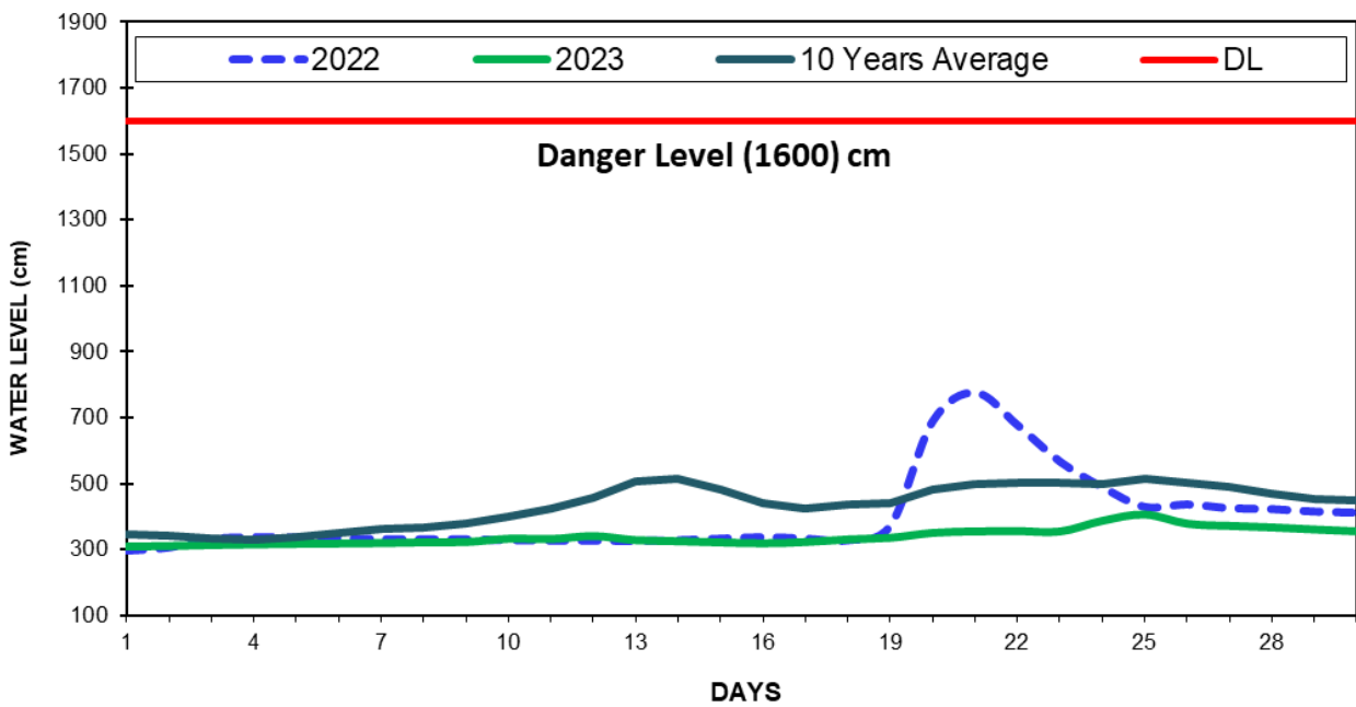
Fig(16) COMPARISON OF JUNE WATER LEVELS OF 2023 WITH JUNE WATER LEVELS OF 2022 AND 10 YEARS AVERAGE (PALETWA)
