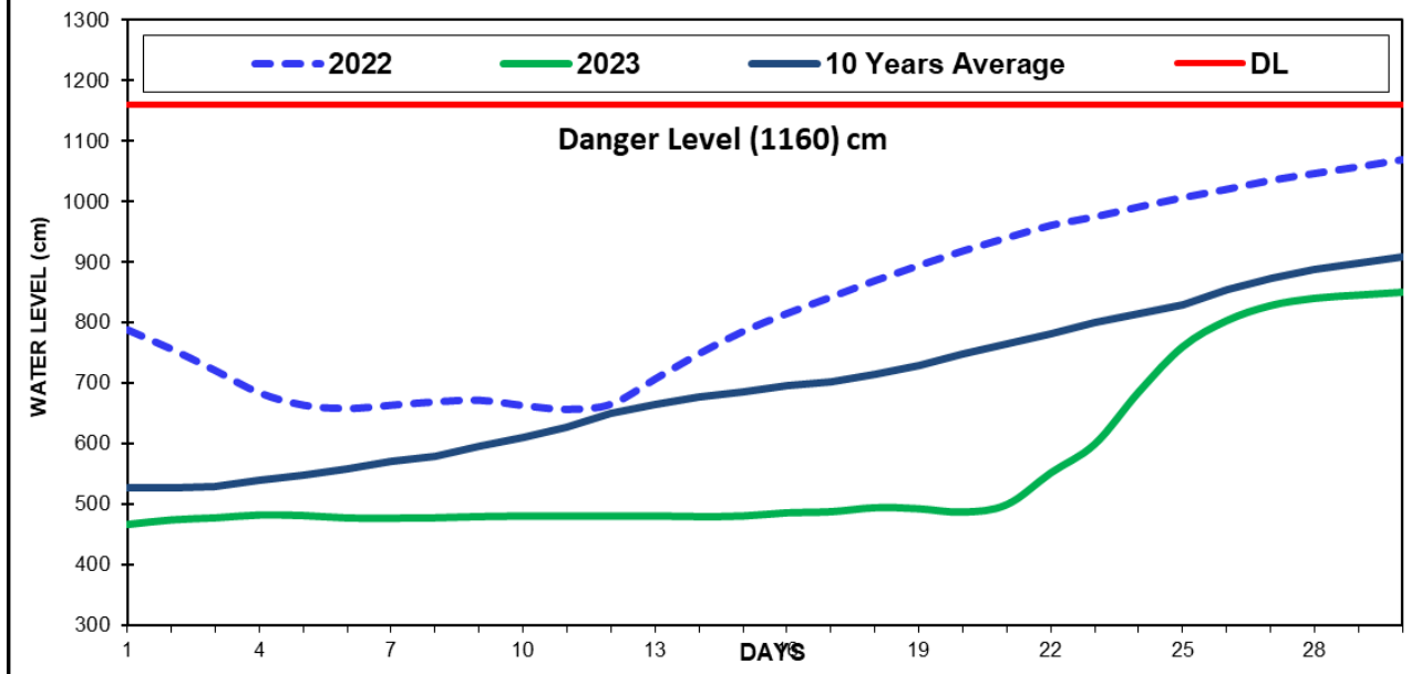
Fig(14) COMPARISON OF JUNE WATER LEVELS OF 2023 WITH JUNE WATER LEVELS OF 2022 AND 10 YEARS AVERAGE (NGATHAINGCHAUNG)
