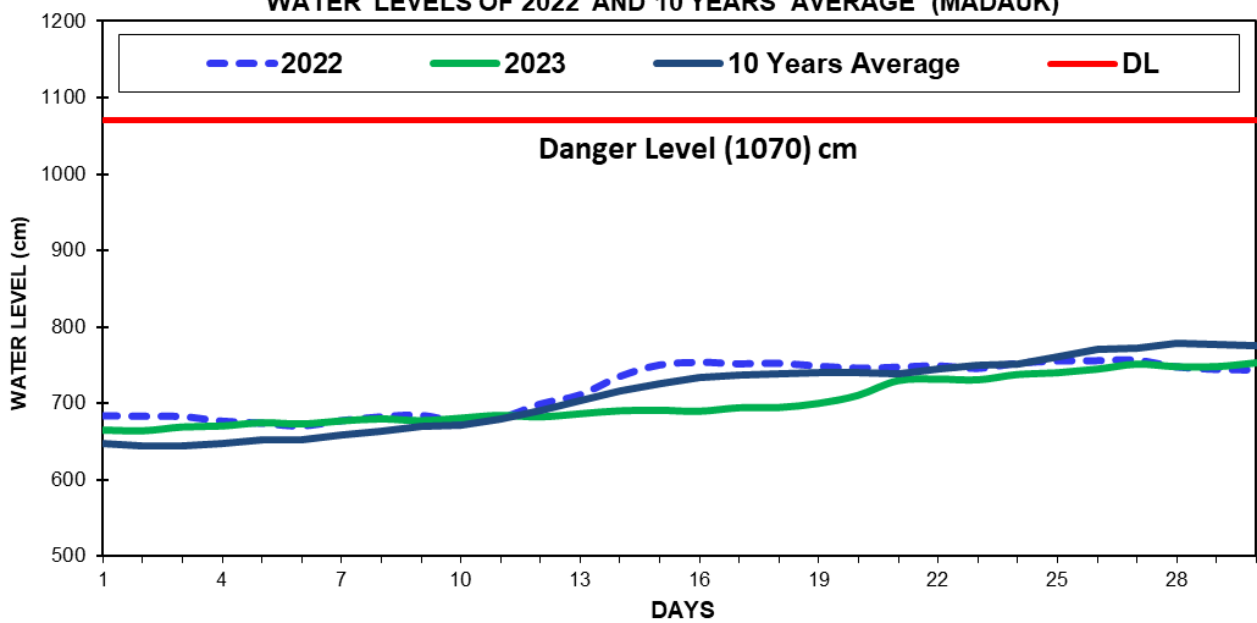
Fig(10) COMPARISON OF JUNE WATER LEVELS OF 2023 WITH JUNE WATER LEVELS OF 2022 AND 10 YEARS AVERAGE (MADAUK)
