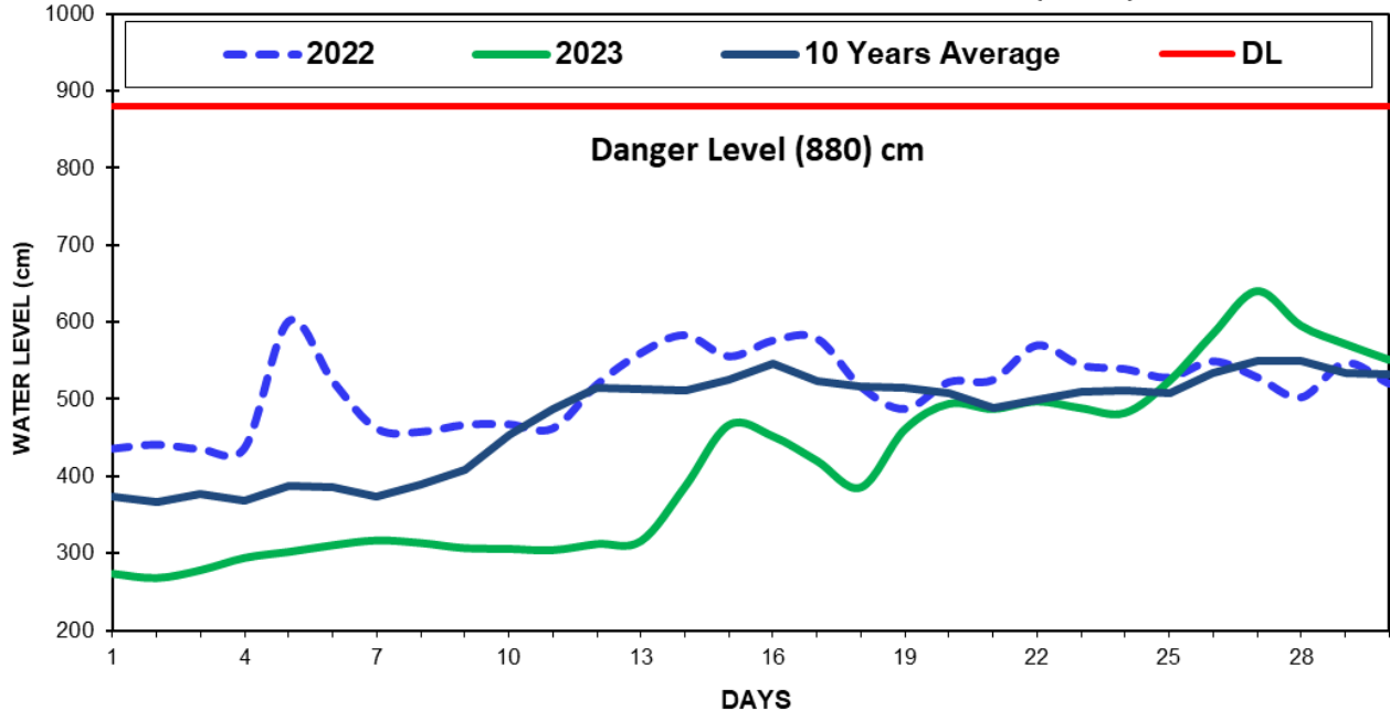
Fig(12) COMPARISON OF JUNE WATER LEVELS OF 2023 WITH JUNE WATER LEVELS OF 2022 AND 10 YEARS AVERAGE (BAGO)
