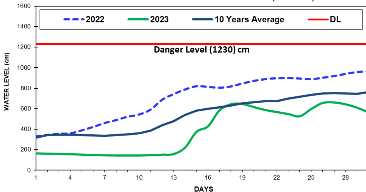
Fig(6) COMPARISON OF JUNE WATER LEVELS OF 2023 WITH JUNE WATER LEVELS OF 2022 AND 10 YEARS AVERAGE (MAWLAIK)
