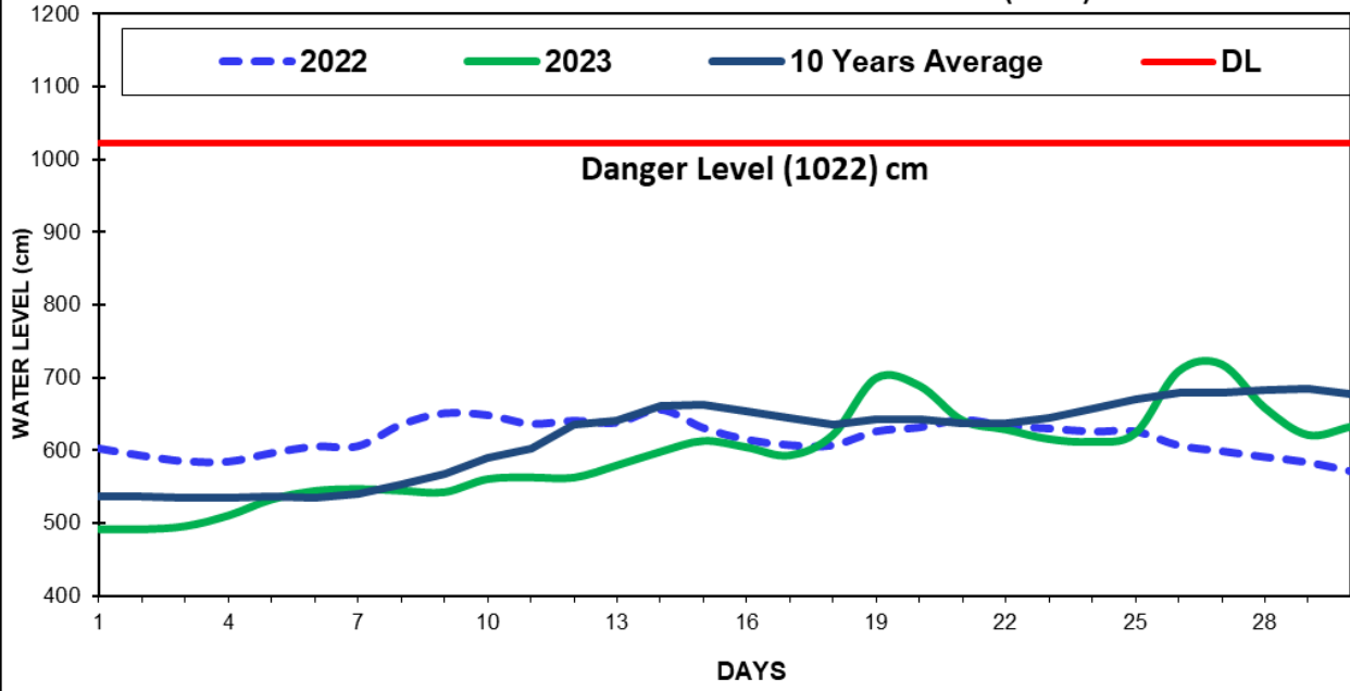
Fig(19) COMPARISON OF JUNE WATER LEVELS OF 2023 WITH JUNE WATER LEVELS OF 2022 AND 10 YEARS AVERAGE (BILIN)
