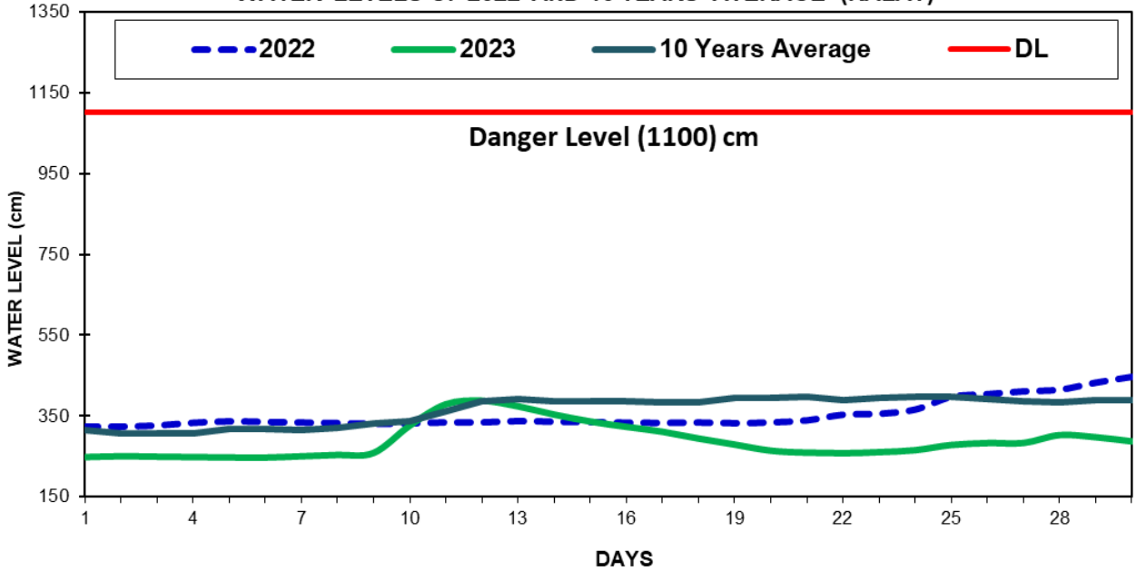
Fig(18) COMPARISON OF JUNE WATER LEVELS OF 2023 WITH JUNE WATER LEVELS OF 2022 AND 10 YEARS AVERAGE (KALAY)
