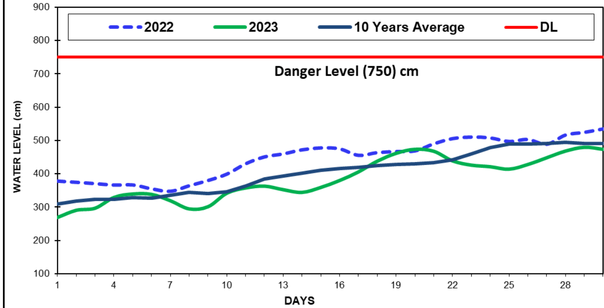
Fig(13) COMPARISON OF JUNE WATER LEVELS OF 2023 WITH JUNE WATER LEVELS OF 2022 AND 10 YEARS AVERAGE (HPA-AN)
