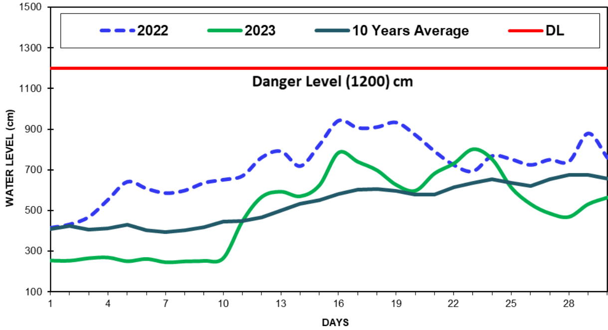
Fig(1) COMPARISON OF JUNE WATER LEVELS OF 2023 WITH JUNE WATER LEVELS OF 2022 AND 10 YEARS AVARAGE (MYITKYINA)
