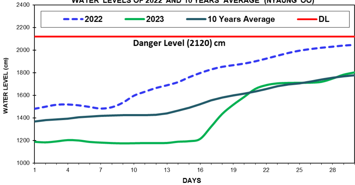
Fig(3) COMPARISON OF JUNE WATER LEVELS OF 2023 WITH JUNE WATER LEVELS OF 2022 AND 10 YEARS AVERAGE (NYAUNG OO)
