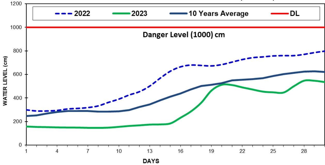
Fig(7) COMPARISON OF JUNE WATER LEVELS OF 2023 WITH JUNE WATER LEVELS OF 2022 AND 10 YEARS AVERAGE (MONYWA)
