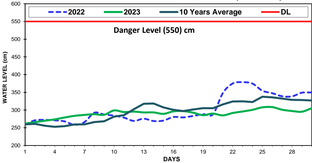
Fig(17) COMPARISON OF JUNE WATER LEVELS OF 2023 WITH JUNE WATER LEVELS OF 2022 AND 10 YEARS AVERAGE (KYAUK TAW)
